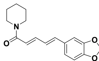
Piperine
