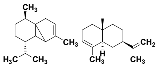
\alpha -cubebene
