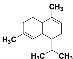
α-murolene
