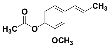
Isoeugenyl acetate
