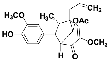
Methylpiperbetol
