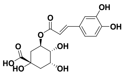
Chlorogenic acid
