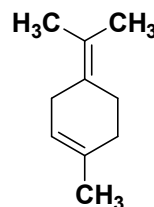
Terpinolene
