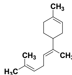
α-Bisabolene
