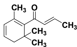
(E)-β-Damascenone
