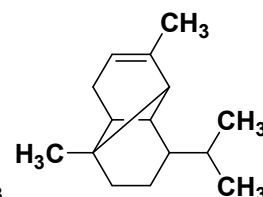
α-copaene
