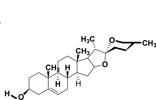
Diosgenin
