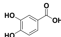
Procatechuic acid
