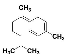
α-farnesene
