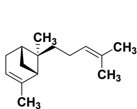
α-bergamotene
