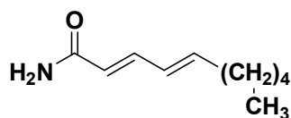
4E-decadienamide
