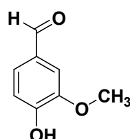
Vanillin
