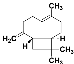
Caryophyllene
