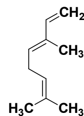
(E)-β-ocimene
