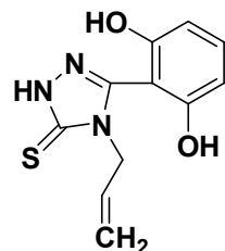
4-allyl resorcinol
