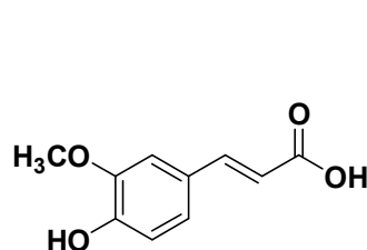
Ferulic acid
