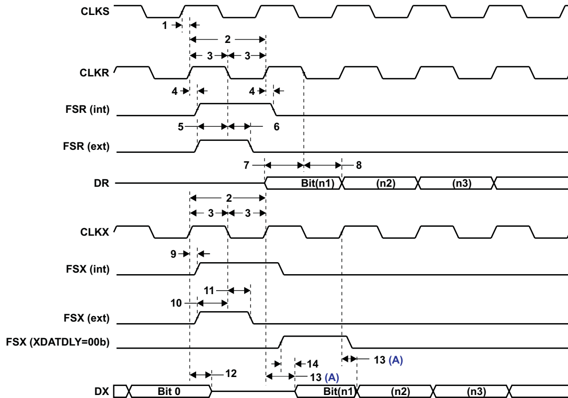
Figure 6-32. McBSP Timing
