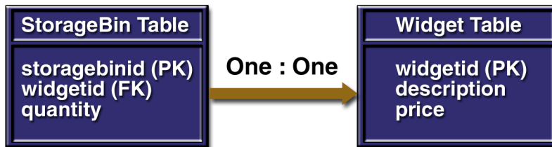
Figure 26–1 One-to-One Table Relationship
