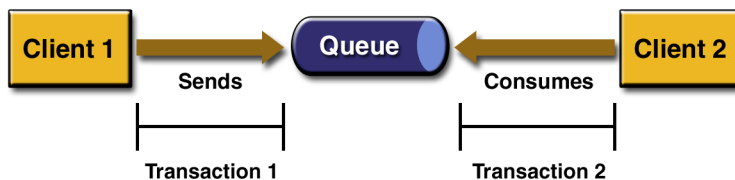
Figure 33–11 Using JMS API Local Transactions
