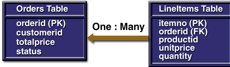
Figure 26–2 One-to-Many Relationship: Order and Line Items
