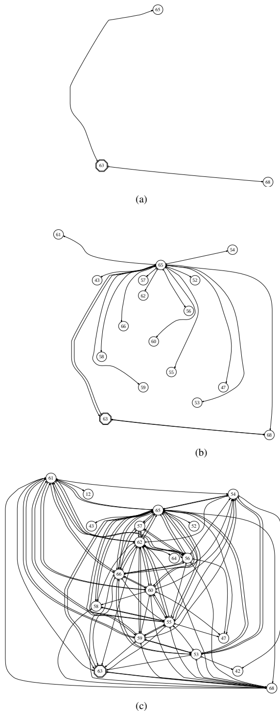
Figure 1: Host nodes that are reachable in 1 (a), 2 (b), and 3 (c) steps from a source host by traversing known_hosts edges.
