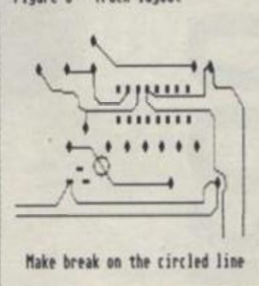
Figure 3 - Track layout
