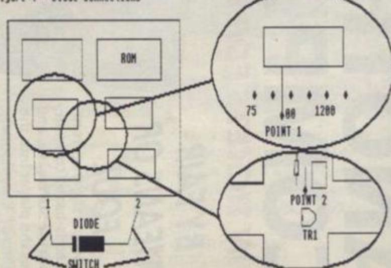
Figure 4 - Diode Connections
