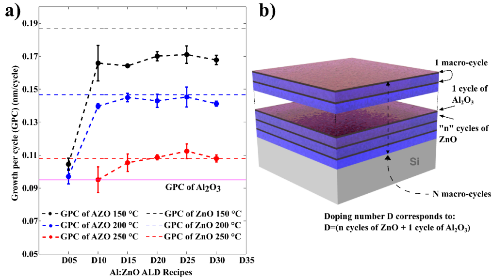
Fig. 1. ALD deposition conditions. a) Growth per cycle of Al 2 O 3 , ZnO and AZO for each temperature regime: 150 °C, 200 °C and 250 °C. b) Schematic drawing of deposited AZO layers and concept illustration of doping “D” number.
