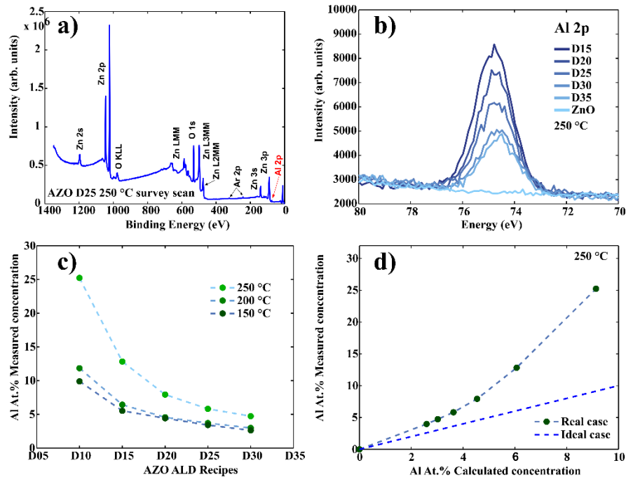
Fig. 2. XPS investigation of AZO layers. a) The typical survey scan of AZO/ZnO. b) High-resolution scan for Al2p region for AZO/ZnO samples prepared at 250 °C. c) Measured Al concentration in AZO films prepared at three temperatures: 150 °C, 200 °C and 250 °C. d) Deviation of the measured Al at. % concentration from the theoretical estimation in case of 250 °C deposition temperature.
