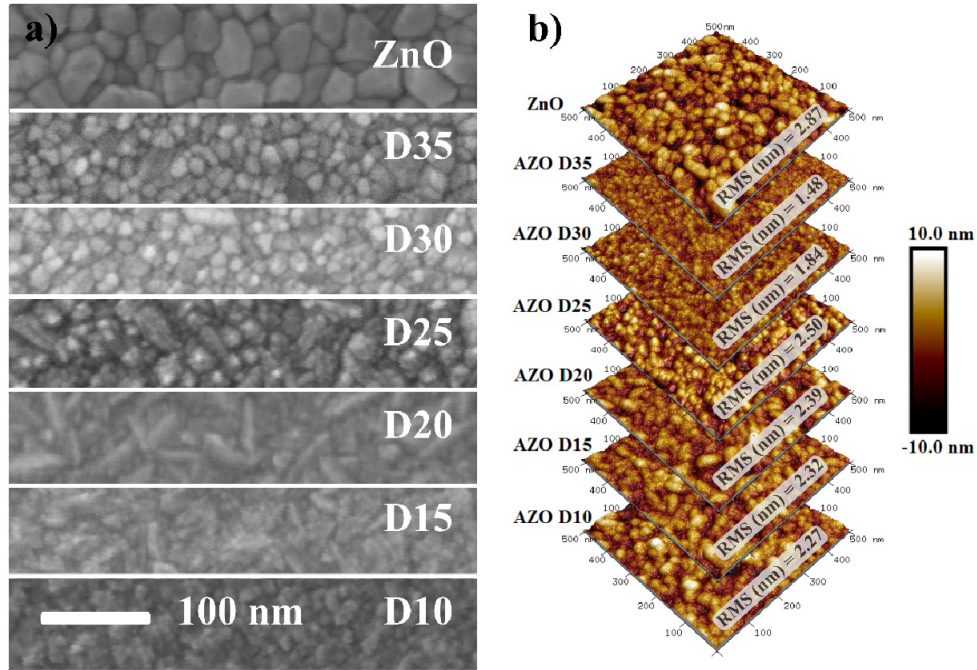
Fig. 3. Morphology inspection. a) SEM and b) AFM images (500 nm × 500 nm) of flat AZO samples prepared at 250 °C.
