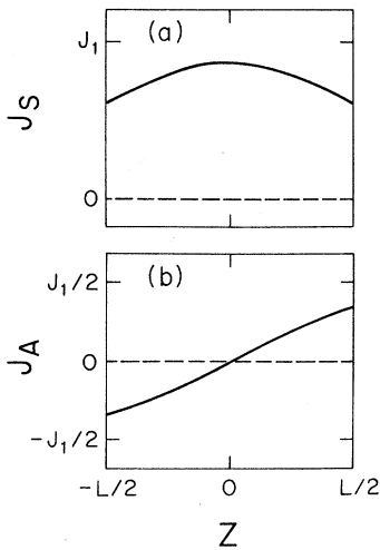
FIG. 4. Current density as a function of position in the junction for I_{dc} < I_M : (a) the symmetric part J_S = J_1 \sin\phi_0 \times \cos(2\pi z \Phi_y / L \Phi_0) ; (b) the antisymmetric part J_A = J_1 \cos\phi_0 \times \sin(2\pi z \Phi_y / L \Phi_0) . \sin\phi_0 = 0.86 ; \Phi_y = 0.25\Phi_0 .
