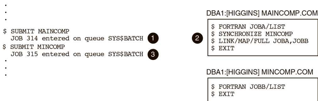
Figure 16.1. Synchronizing Batch Job Execution
