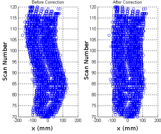
Fig. 4: Top view of bucket point cloud before (left) and after (right) sway correction is applied. A single scanline consists of points along the x axis.
