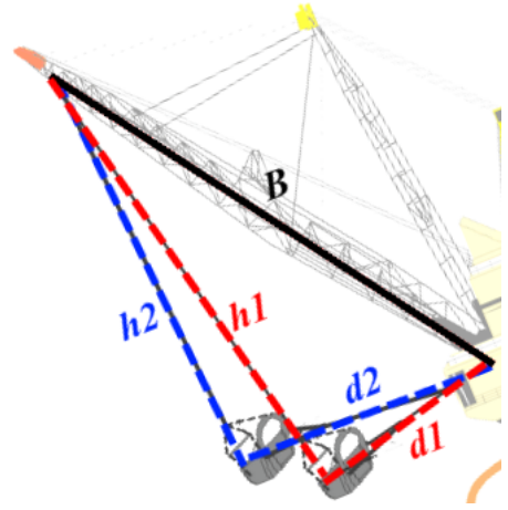
Fig. 5: Bucket position estimated from rope lengths provided by a third party dragline monitor.
