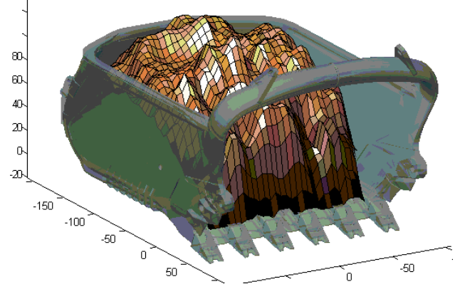
Fig. 1: Processed scaled payload data with superimposed bucket model.
