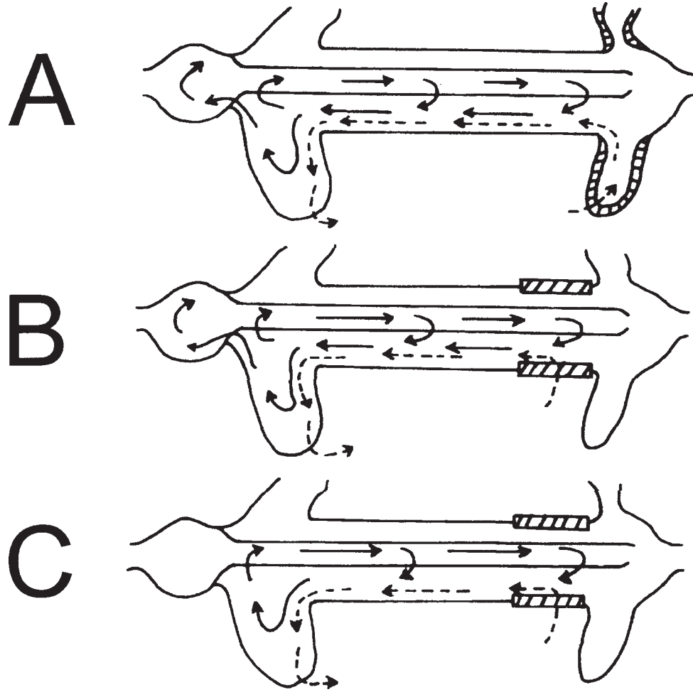
Fig. 4. Diagrammatic representation of water fluxes (dotted arrows) and the circulation of digestive enzymes (solid arrows) in putative insect ancestors (A–C). In Neoptera ancestors (A), midgut digestive enzymes pass into the crop. Countercurrent fluxes depend on the secretion of fluid by the Malpighian tubules and its absorption by the caeca. Holometabola ancestors (B) are similar, except that secretion of fluid occurs in poste-
