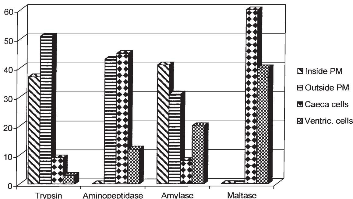
Fig. 3. Enzyme activities (%) in midgut compartments of Rhynchosciara americana . Enzymes were sampled from these compartments by aspirating the ectoperitrophic fluid from caeca with the aid of a capillary, then by dissection the contents of the peritrophic membrane and caeca and
