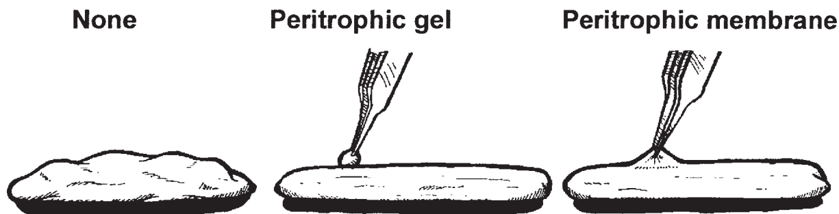
Fig. 1. Identification of film types surrounding the food bolus. After dissection, the midgut contents maintain their form (usually cylindrical) when a surrounding film is present. The
