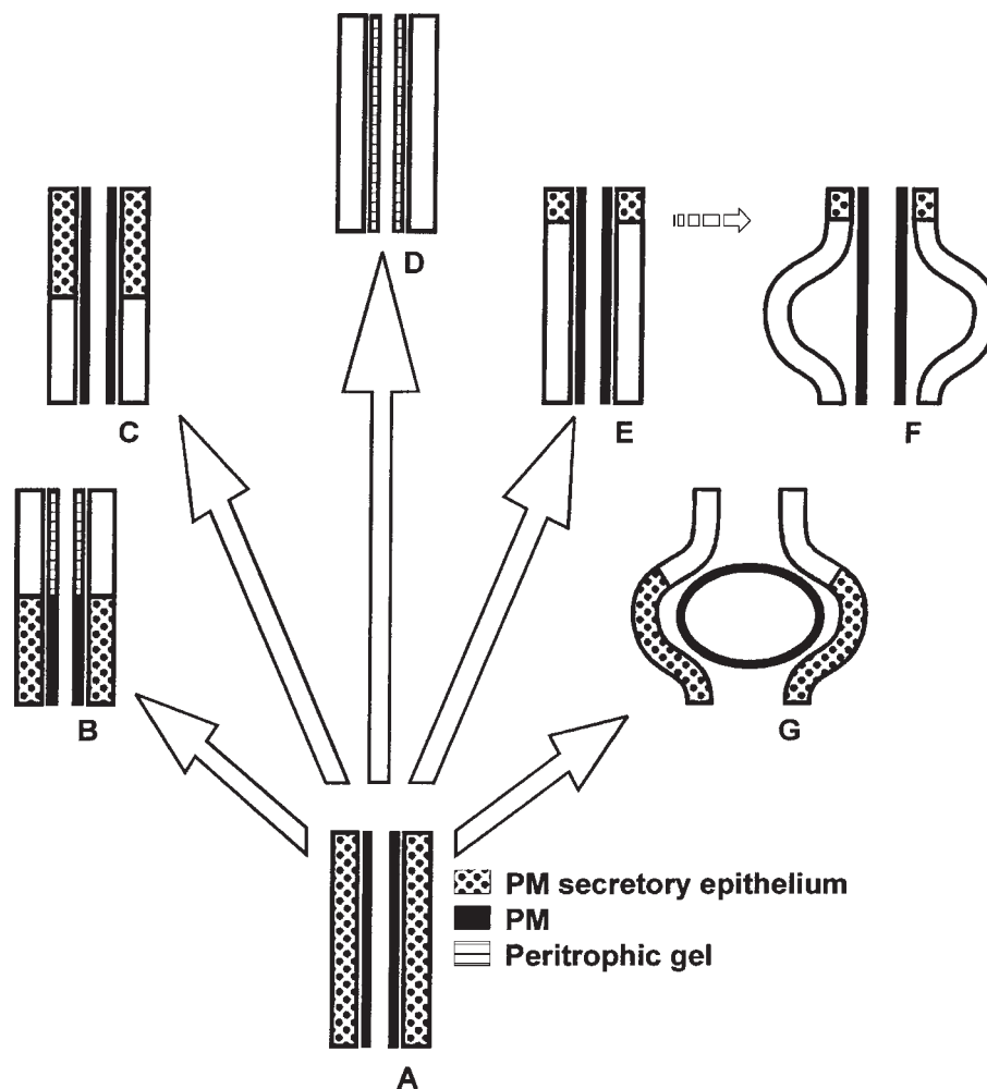
Fig. 2. Occurrence of peritrophic gel and peritrophic membrane (PM) in insects. Type I PM (A–C, D, G) is formed by most midgut epithelium, whereas type II PM (E, F) is secreted by a few row of cells at the entrance of the midgut (cardia). F is a hypothetical condition where a type II PM is formed in an insect with a dilated posterior midgut (like an
