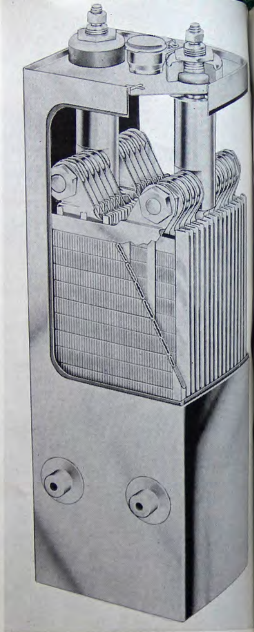
Fig. 6. This is a Gould-National Nicad cell in cut-away; both Edison and Nicad cells use the general structure made possible by the very high strength of the nickel-plated steel plates, and steel cell case. Separators aren't needed, because the plates themselves are adequately rigid.
