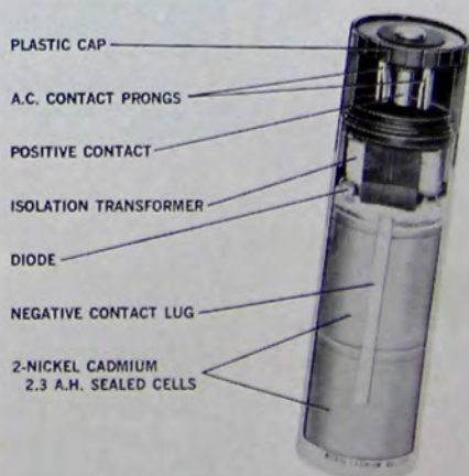
Fig. 11. Cut-away view of the typical plug-in-the-wall rechargeable Ni-Cd flashlight battery unit. This one's the Nicad Battery Co. design, but Nicad supplies them to a number of companies for sale under assorted brand-names.
