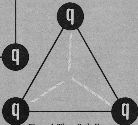
Figure 4. Three Body Forces
