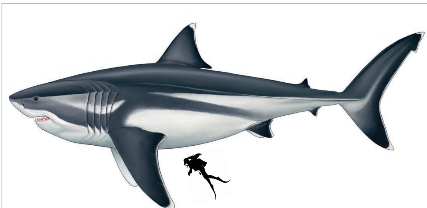
Fig. 5: The final full-body reconstruction of a 16 metre Megalodon created from our work, compared against a 1.6 m diver. Reconstruction by Oliver E. Demuth. Figure from Cooper et al. , Sci. Rep. 10 , 1–9 (2020). Copyright © 2020, Springer Nature. Creative Commons CC BY license.
