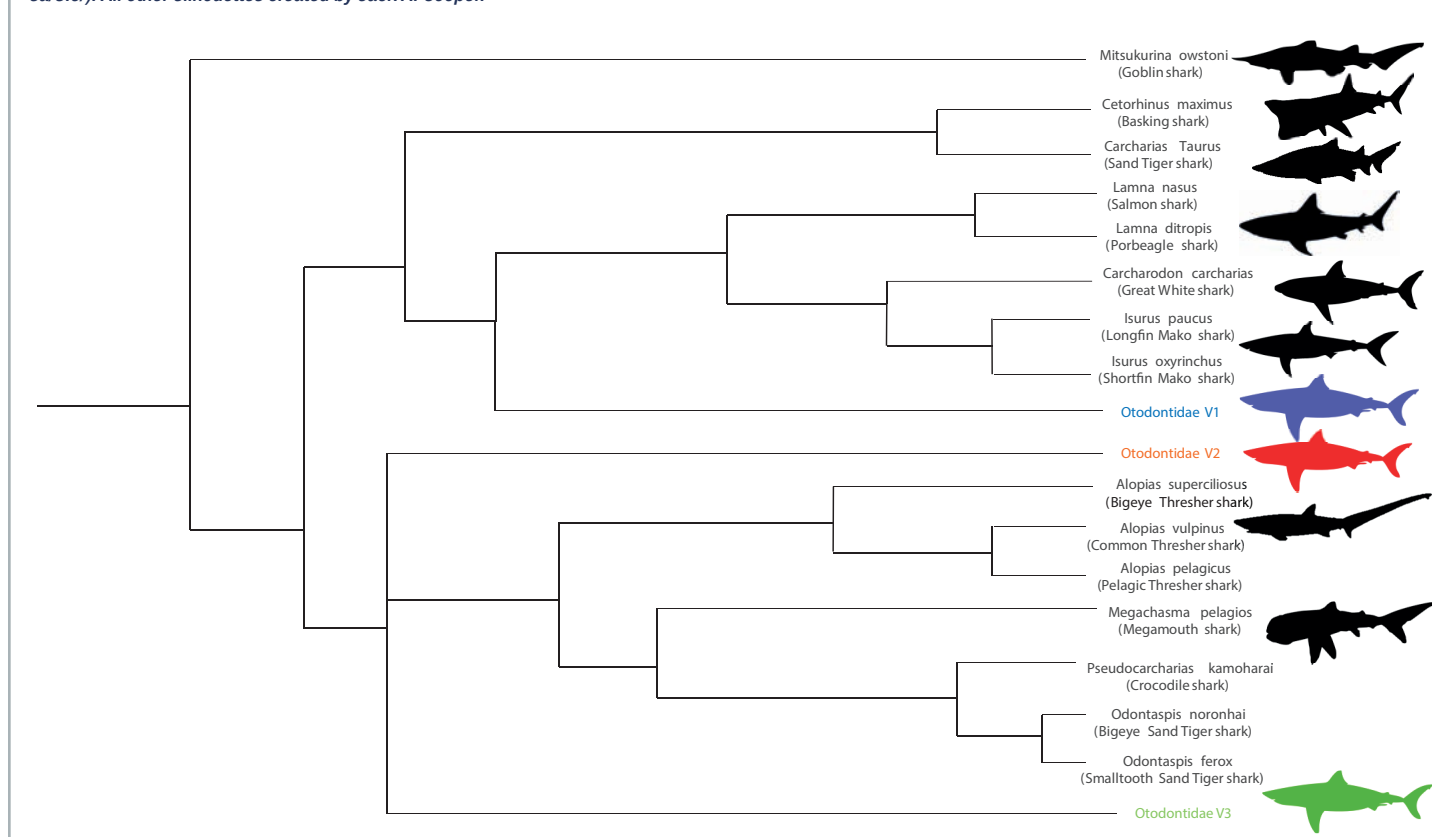
Fig. 3: A phylogenetic, or family tree of Order Lamniformes. There are 15 extant species in the Lamniformes order (shown in black). It is unclear where the Otodontidae family, that of Megalodon , sits in relation to these living sharks and 3 separate hypotheses (V1, V2 and V3 – shown in blue, orange and green respectively) are shown as examples. V1 (blue) suggests that the closest living ancestors would be family Lamnidae, the family consisting of the great white, mako, salmon and porbeagle sharks. V2 and V3 suggest that Otodontidae share common ancestors with thresher and sand tiger sharks respectively, theories that have also been proposed. However, given that Megalodon shares numerous traits with the lamnid sharks, including dental and physiological similarities, we suggest that the V1 placement is the most parsimonious. Silhouettes for M. owstoni (by Haplochromis, vectorised by T. Michael Kessey), C. carcharias (by Steven Traver), Isurus species (uncredited), O. megalodon (by Scarlet23, vectorised by T. Michael Kessey) and M. pelagicus (by Jose I. Castro, vectorised by J. Boyle) are found on Phylopic (licence: https://creativecommons.org/licenses/by-sa/3.0/ ). All other silhouettes created by Jack A. Cooper.
