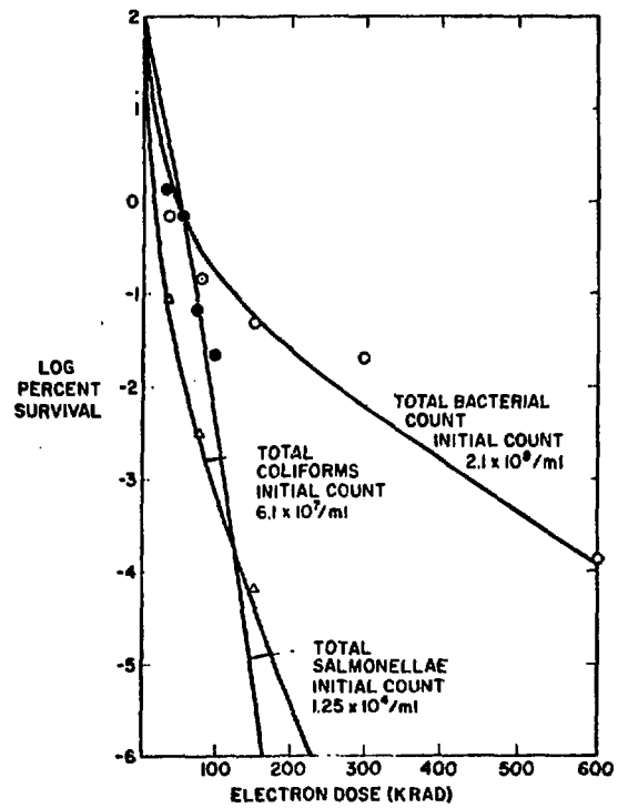
Figure 1. Electron Inactivation of Bacteria in Primary Raw Sludge
