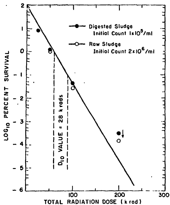
Figure 2. Electron Inactivation of Fecal Coliforms in Primary Raw and Anaerobically Digested Sludge
