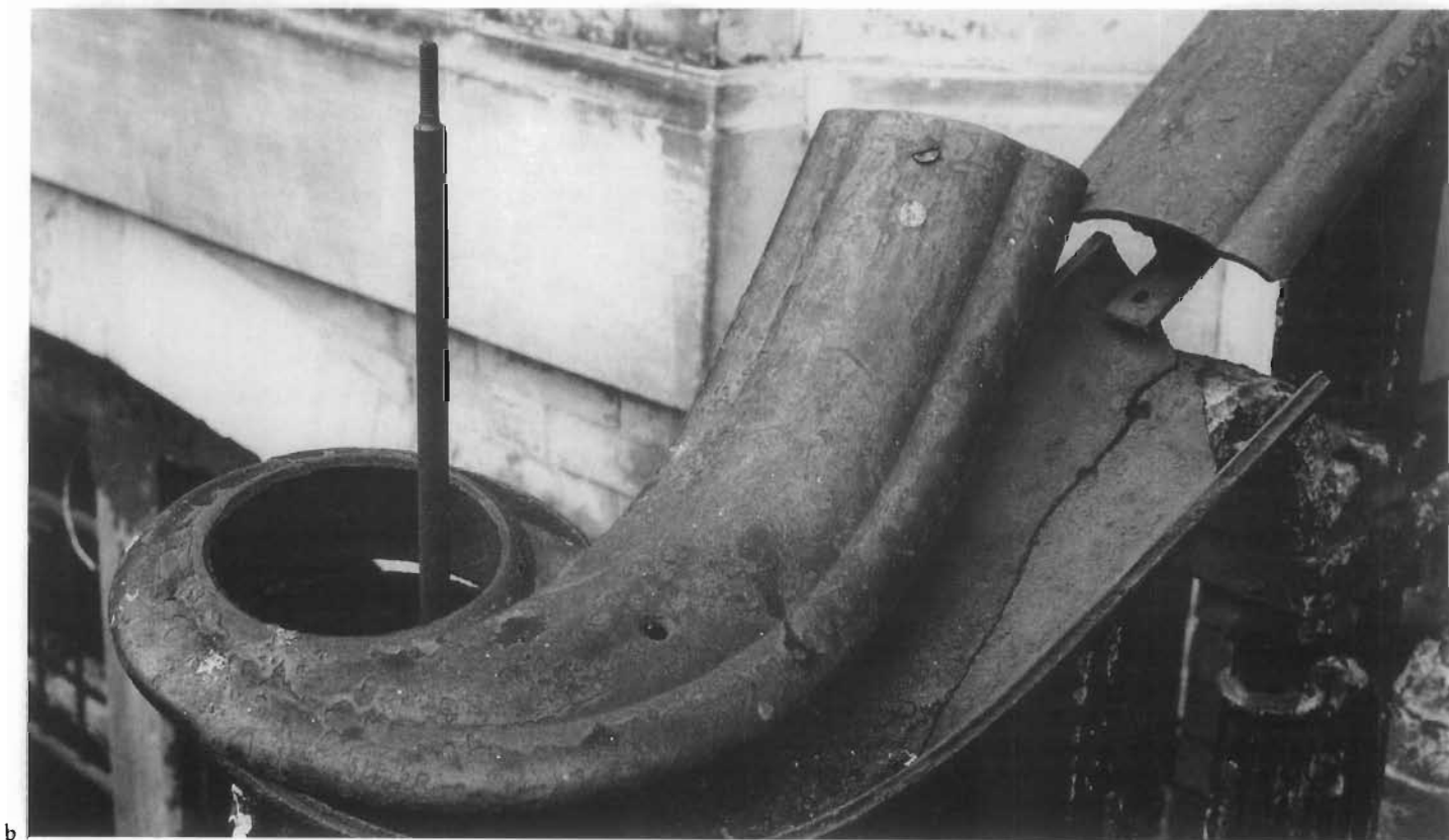
Figure 160. Cast-iron Corrosion, Fracture, and Missing Pieces. (a) The massive newel posts of the stair railings on the entrance of 637 I Street, NW in Washington, D.C., are hollow and are made up of several pieces screwed and bolted together. The newel post to the right side of the stairs is substantially intact. (b) The finial of the left newel post is missing. Note the threaded rod in the center of the newel post used for assembly. Inside the railing, loose rust has collected to a depth of about a half inch. Water seeped into the hollow rail and froze, resulting in the crack. (David W. Look)
