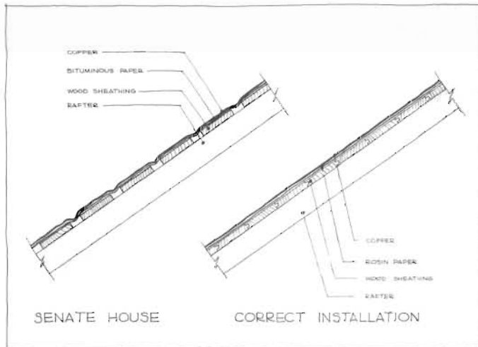
Figure 147. Fatigue Failure. Fatigue failure occurred on the copper roof installed during the 1920s on the Senate House in Kingston, New York. (a) Failure was caused by cyclical expansion and contraction of the copper without adequate provisions for it. Additionally, the copper sheet was too thin and not rigid enough to resist buckling and sagging between the too-widely-spaced roof sheathing. The use of bituminous roofing paper between the copper and sheathing also contributed to the failure; when the paper was heated by the sun, it adhered to the copper, further restricting its movement (see figure 117). (b) The drawing shows the actual roof installation and the correct procedure, which allows for expansion and contraction. (John G. Waite)
