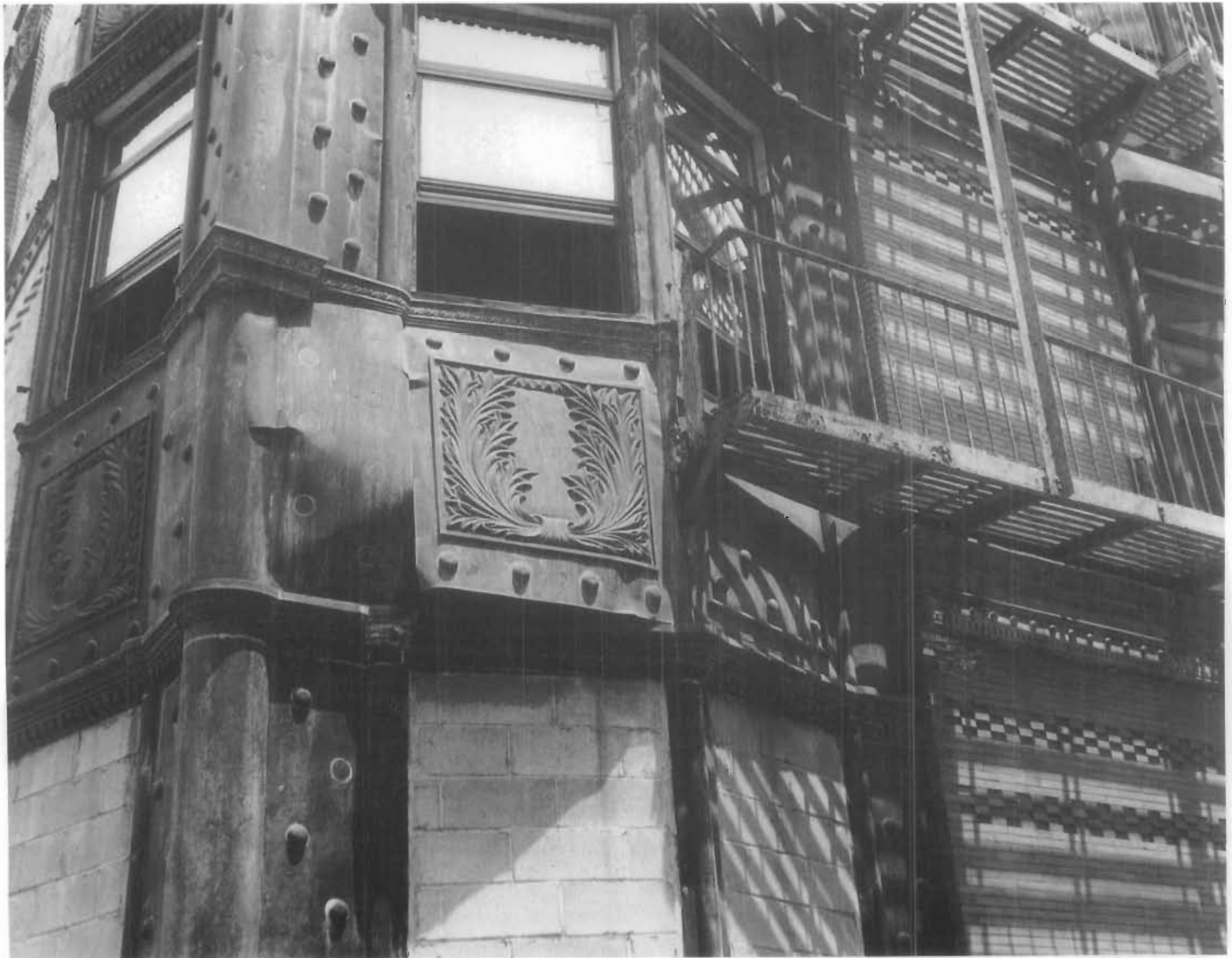
Figure 146. Loose and Damaged Copper Cladding and Deteriorated Steel Fire Escapes. The corner bay of the Hotel Margueret (1889) in Brooklyn Heights, New York, was clad in ornamental panels of pressed sheet copper. Anchors have deteriorated and the wind has lifted the corners. Galvanic action between the noble copper and the baser steel (in the fire escape) has caused the steel to deteriorate. (David W. Look)
