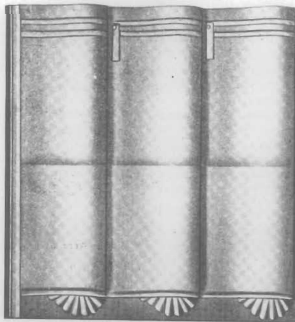
EAVES COURSE PLATE.
