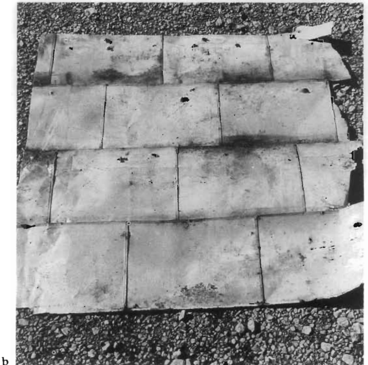
Figure 129. Corrosion Failure of Terneplate Roofing. Hyde Hall, built between 1817 and 1833, near Cooperstown, New York, was roofed with flat-seam terneplate. (a) The plates have deteriorated because of a lack of proper maintenance. Unfortunately, the exposed (top) surface of the terneplate was painted with asphalt coating, which accelerated the corrosion of the roofing. (b) The terneplate also corroded from the underside. When installed, the terneplate was not painted on the underside as it should have been. Condensation formed on the unprotected bottom side of the metal roof and could not evaporate, an ideal situation for corrosion. (John G. Waite)
