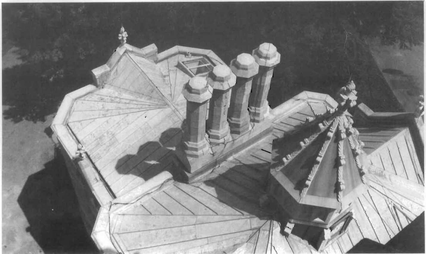
Figure 135. Complete Substitution of Lead-Coated Copper Roofing for Terneplate Roofing. The 1864 wing addition of Lyndhurst, Tarrytown, New York, originally had a terneplate roof. In an attempt to find a more permanent roofing material, a lead-coated copper roof was substituted for the terneplate, duplicating the pattern and sheet sizes of the original roof. In such substitutions, details may have to be redesigned because of differences in expansion and contraction rates and differences in workability of the material. The color of lead-coated copper is not the same as terneplate because terneplate roofing was never left unpainted. Therefore, lead-coated copper roofing substituted for terneplate should also be painted if it seen from normal viewing angles (usually from street level). (John G. Waite)
