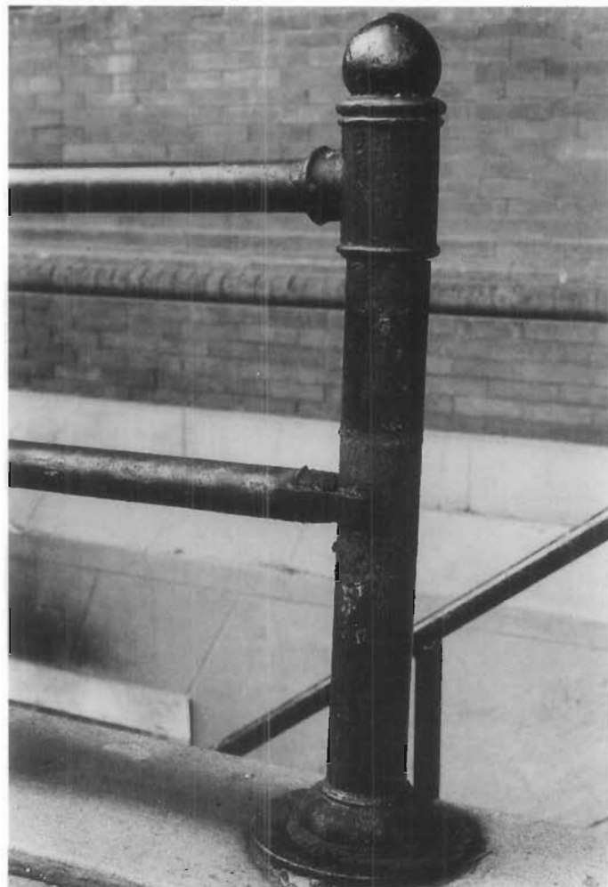
Figure 161. Inappropriate Repairs of Cast Iron. A simple cast-iron pipe railing guards the areaway of the Old Pension Building in Washington, D.C. The collar on the newel post to receive the bottom rail is missing (it probably cracked off from the pressure of expanding rust and/or ice). Unfortunately, a strap was welded to each side instead of repairing or reproducing the collar. (David W. Look)
