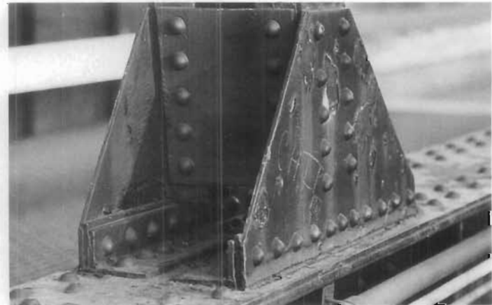
Figure 159. Defective Original Design Detail. Corrosion of the connection between the girder and the built-up truss members has occurred on the former Delaware and Hudson Railroad Bridge, 1884, over the Hudson River between Troy and Green Island, New York, because the connection served as a pocket to trap rain and snow in an area difficult to maintain and protect. This connection is almost impossible to maintain without modification in the design. The connection should be sandblasted, primed immediately, and painted. Since the bottom of the vertical truss member is boxed in, which prevents painting with a brush, the inside of this member could be spray painted. (John G. Waite)
