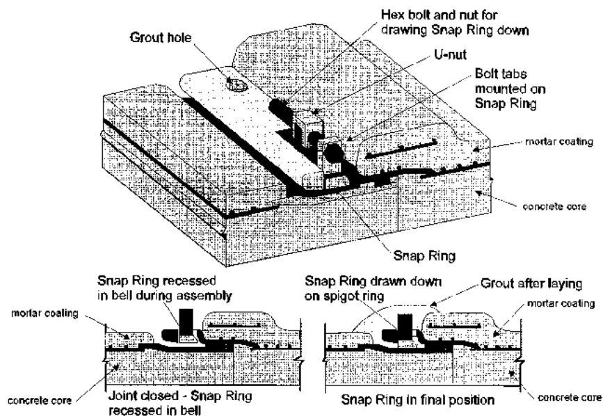
FIGURE A8.10 Snap Ring® restrained joint.
