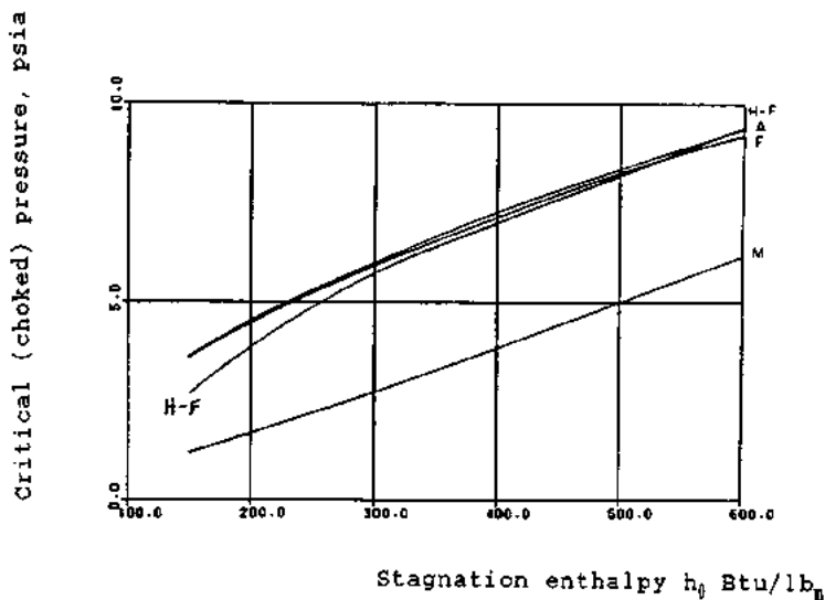
FIGURE B8.47 Predicted critical pressure versus stagnation enthalpy. Mass flux = 50 \text{ lb}_m/(\text{ft}^2 \cdot \text{s}) . (Stone & Webster data.)
