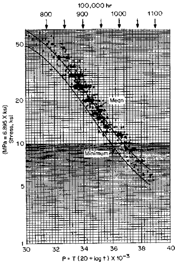
FIGURE A3.21 Variation of Larson-Miller rupture parameter with stress for wrought 1\frac{1}{4} Cr \frac{1}{2} Mo-Si steel. (Evaluation of the Elevated Temperature Tensile and Creep-Rupture Properties of \frac{1}{2} Cr- \frac{1}{2} Mo, 1 Cr- \frac{1}{2} Mo, and 1\frac{1}{4} Cr- \frac{1}{2} Mo-Si Steels, ASTM Data Series Publication DS50.)
