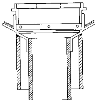
FIGURE B13.55 Example of a thermoplastic double containment floor drain capable of withstanding a 10,000 pound load applied over its cover. ( Orion Fittings, Inc. )
