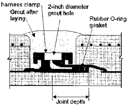
FIGURE A8.11b Embedded cylinder pipe harness clamp restrained joint.
