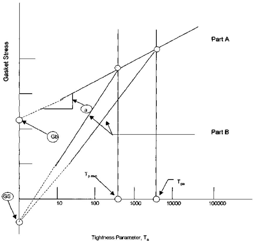
FIGURE A7.17 PVRC idealized tightness curve.
