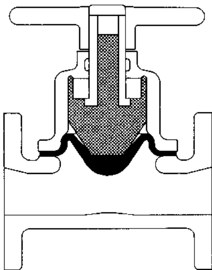
FIGURE A10.27 Straightway-type diaphragm valve.
