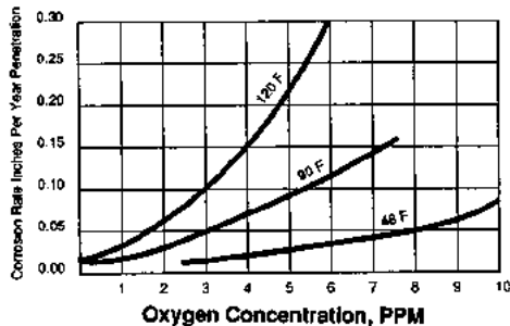
FIGURE B2.3 Effects of oxygen concentration on the corrosion of low-carbon steel in tap water at different temperatures. (Reprinted by permission from Corrosion Basics: An Introduction , National Association of Corrosion Engineers, Houston, 1984, Figure 8.1, p. 149.)
