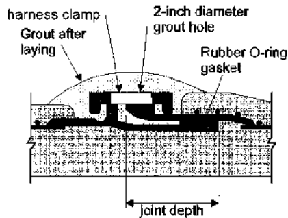
FIGURE A8.11a Lined cylinder pipe harness clamp restrained joint.
