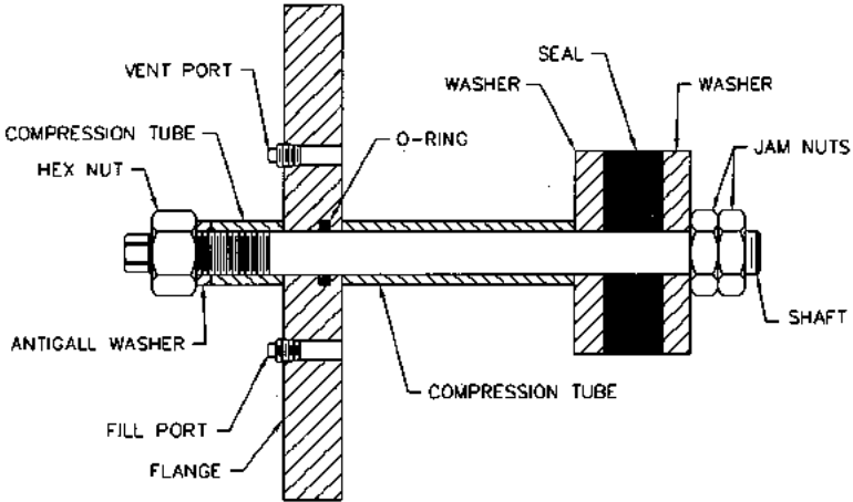
FIGURE B14.3 Flange test plug and flange weld plug. (Courtesy of Expansion Seal Technologies, Harleysville, PA.)
