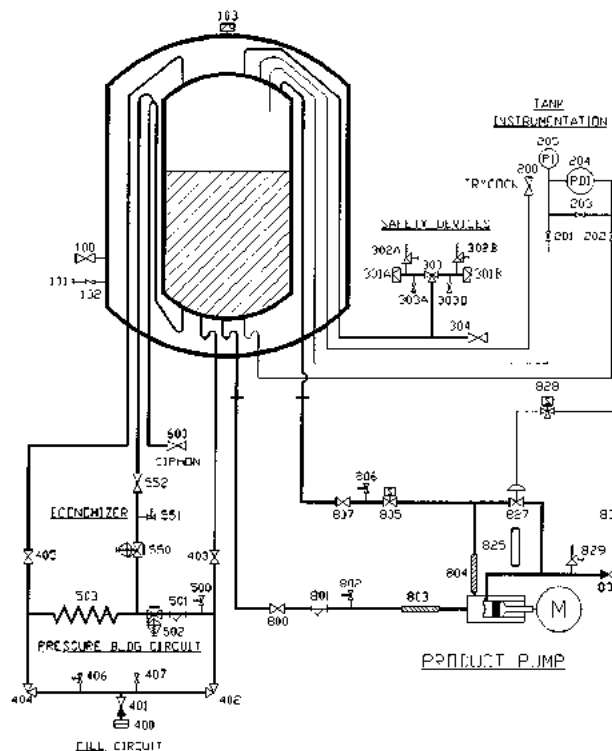
FIGURE C8.12 High-pressure bulk conversion system. (Courtesy of Praxair, Inc.)
