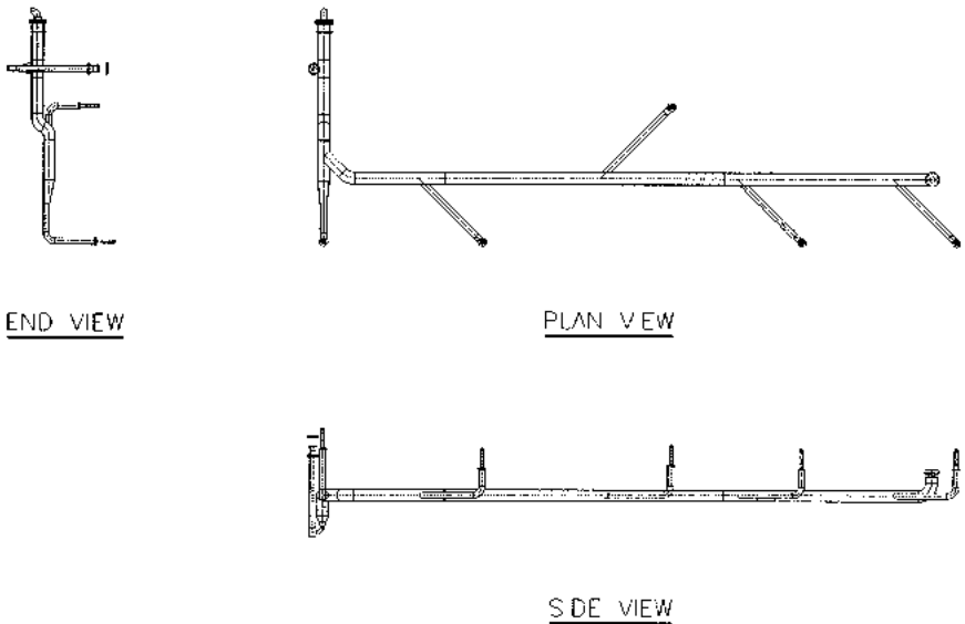
FIGURE B13.65 A typical underground lab-waste header subassembly in a gravity-waste application.
