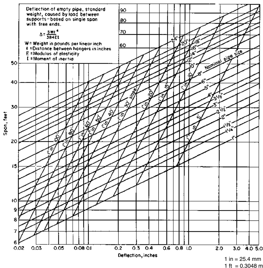
FIGURE B4.18 Deflection of empty pipe.
