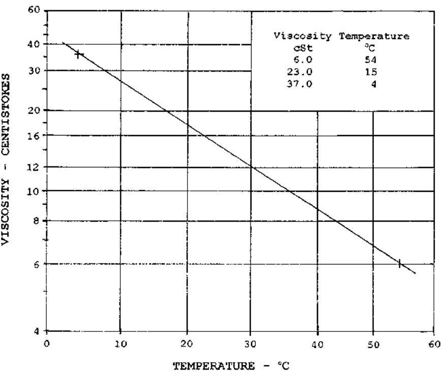
FIGURE C5.3 Example viscosity versus temperature, crude oil.
