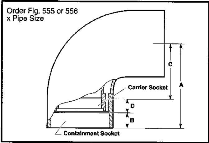
FIGURE B13.27 Restrained fiberglass 90° elbow (U.S. Patent 4,886,305; Fibercast Co.)
