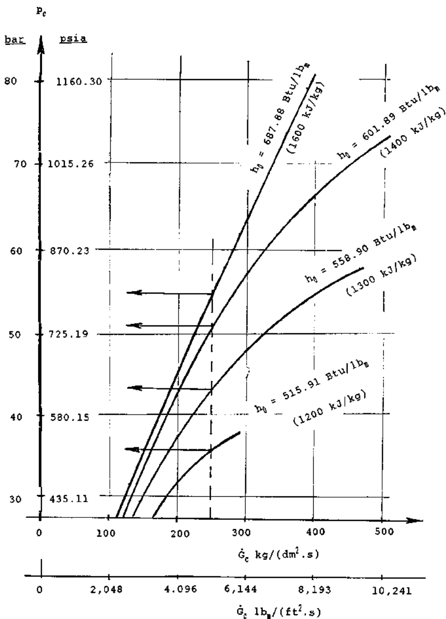
FIGURE B8.46 Critical two-phase flow by Henry-Fauske. (Line for h_0 = 1400 \text{ kJ/kg} , based on results from Table B8.16.)
