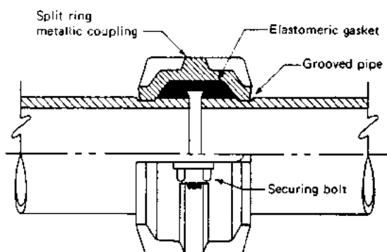
FIGURE C13.8 Grooved joint.
