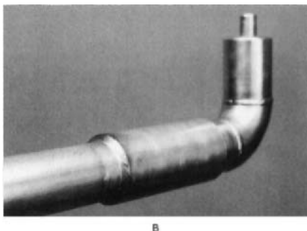
FIGURE B13.78b Shown here is the tubular slip-coupling after it is telescoped into position and welded on both ends to close the gap. (Guardian Division of Eslon Thermoplastics, Inc.)
