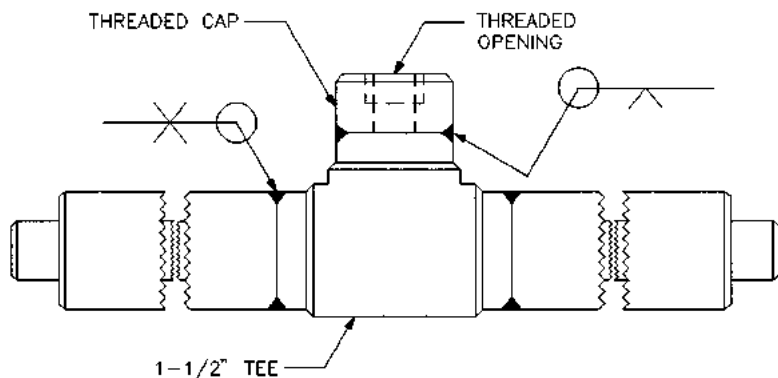
FIGURE B13.98 Illustration of a pressure tap in a secondary-containment pipe for attachment of a pressure gauge.
