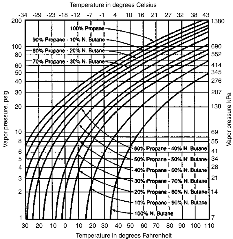
FIGURE C17.6 Vapor pressure produced from different mixtures of propane and butane.
