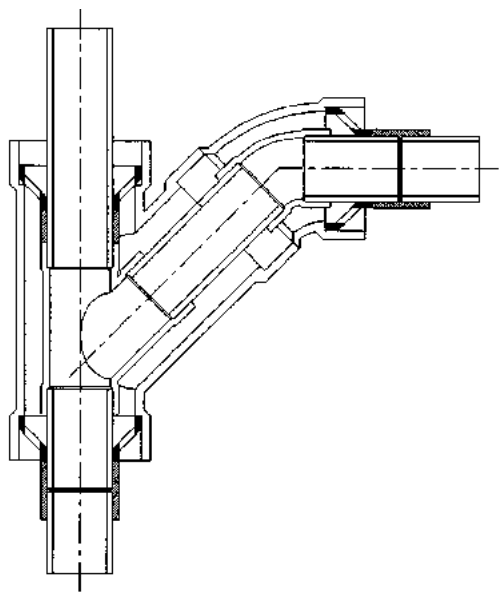
FIGURE B13.46 Rionlock™ thermoplastic restrained long-turn wye using molded code approved carrier fitting. ( Patent Pending; Orion Fittings, Inc. )
