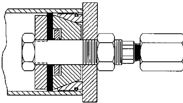
GRIP TIGHT TEST PLUG INSTALLED IN PIPE
