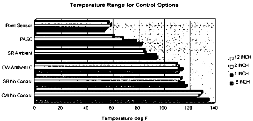
FIGURE B6.18 Temperature range for control options.
