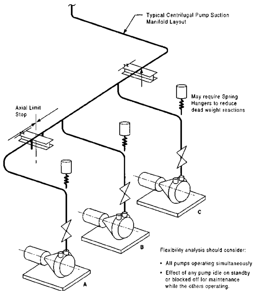
FIGURE C7.17 Typical piping layout for spared pump service.
