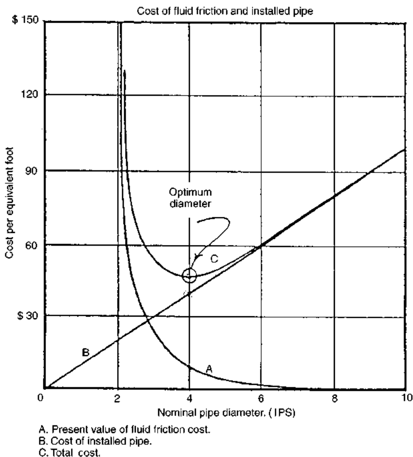
FIGURE C9.3 Cost of fluid friction and installed pipe.
