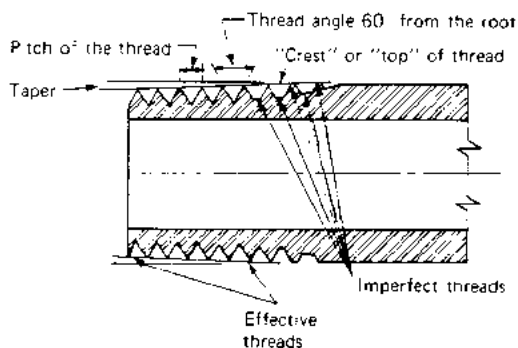
FIGURE C13.4 Screwed joint.
