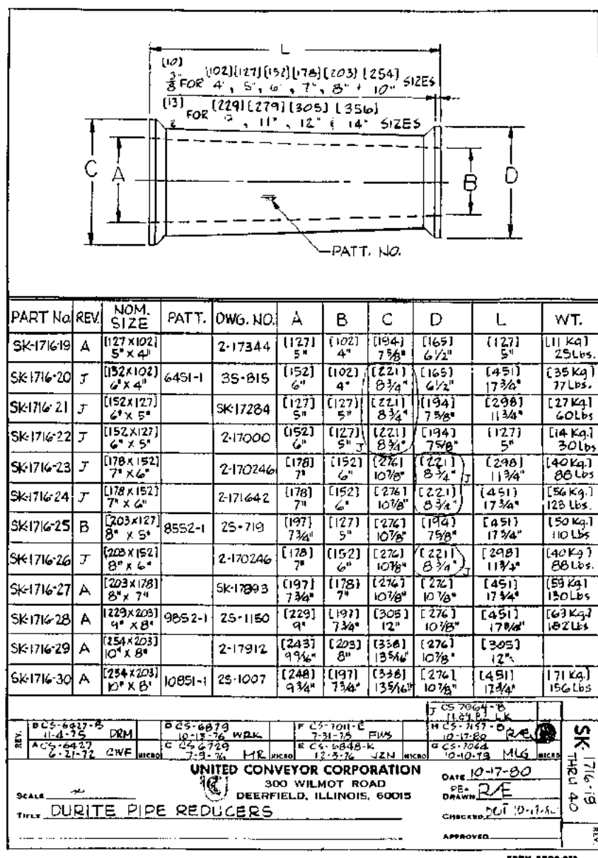
FIGURE C14.9 Durite (UCC) fitting selection drawing, 3 of 4.
