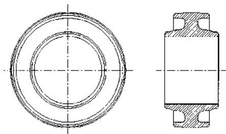
FIGURE B13.15 An example of a homogeneous internal anchor coupling having a solid annulus for compartmentalization purposes. (U.S. Patents #5,141,261 and 4,930,544)
