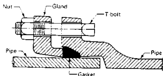
FIGURE C13.7 Mechanical joint.
