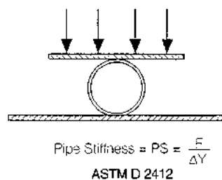
FIGURE D2.4 Simplified load orientation used for determining unit stress and elastic modulus according to ASTM test methods.
