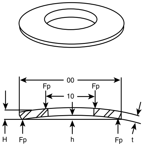
FIGURE A7.8 Section of Belleville spring.
