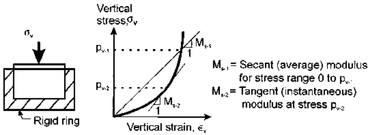
FIGURE D1.15 Constrained modulus, M_p .
