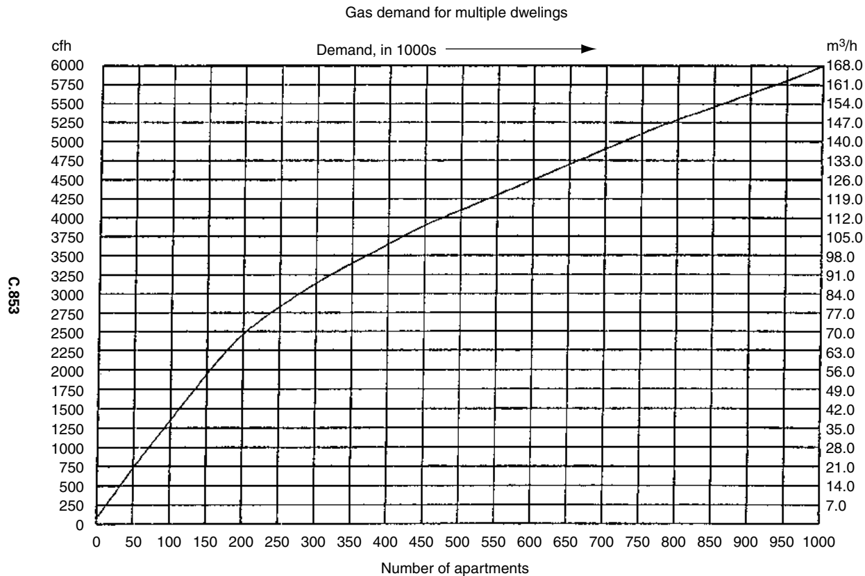
FIGURE C17.2 Gas demand for multiple dwellings.
