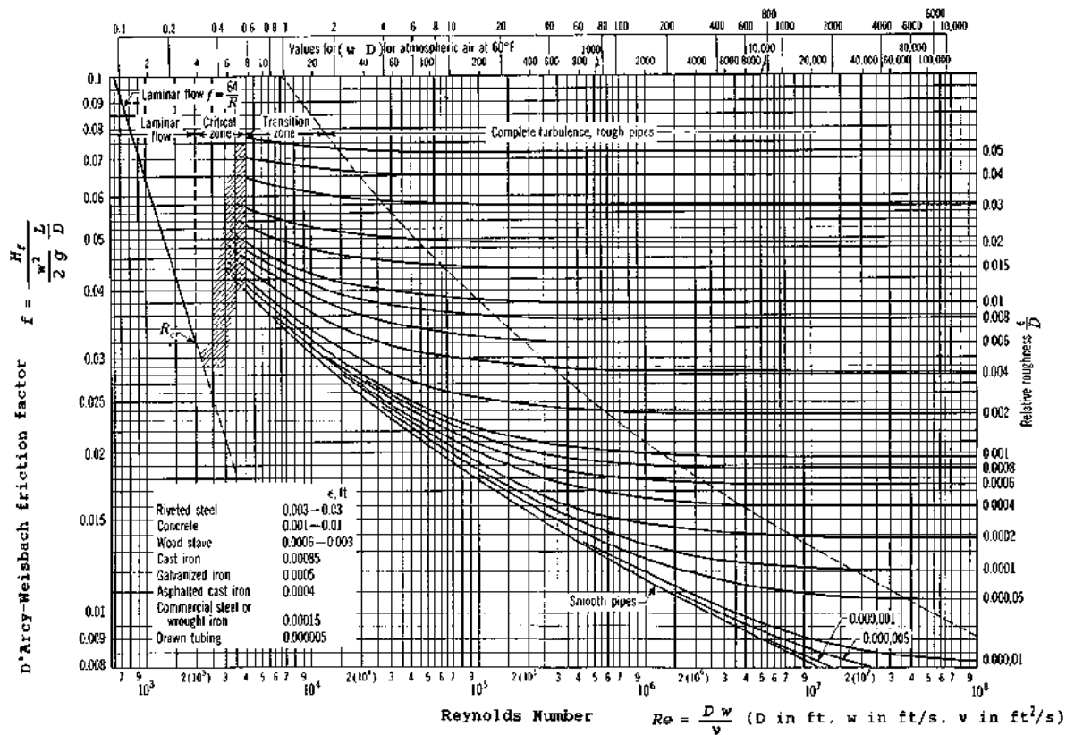
FIGURE B8.5 Moody diagram. (From Ref. 1.)
