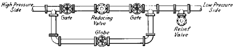
FIGURE C3.11 Pressure-reducing station.
