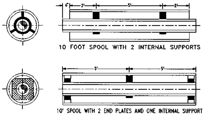
FIGURE B13.3 Example of factory prefabricated 10-ft lengths of piping showing support spacing based on 5-ft spacing between supports for piping intended for staggered joining (top) and simultaneous joining (bottom). ( Orion Fittings, Inc., Kansas City, KS )
