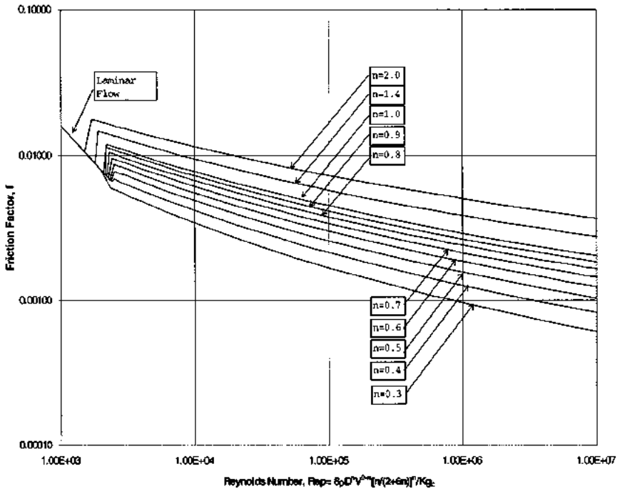
FIGURE C11.8 Friction factor f as a function of Reynolds number for pseudoplastic slurries. Re_p = 8\rho D^n V^{2-n}(n/(2 + 6n))^{1/2}/(Kg_c) where D = pipe ID (ft), V = velocity (ft/s), \rho = density (lb/ft 3 ), K = consistency (lb \cdot s n /ft 2 ), g_c = 32.2 (lb \cdot s/(lb \cdot ft 2 )).
