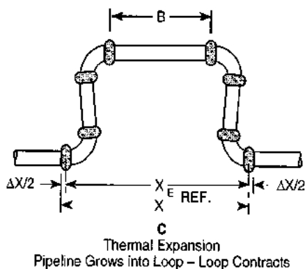
FIGURE A9.21 Thermal expansion loop.
