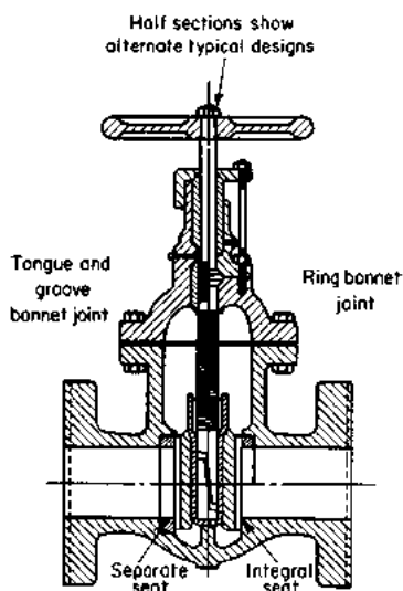
FIGURE A10.7b Double-disc nonrising-stem gate valve.
