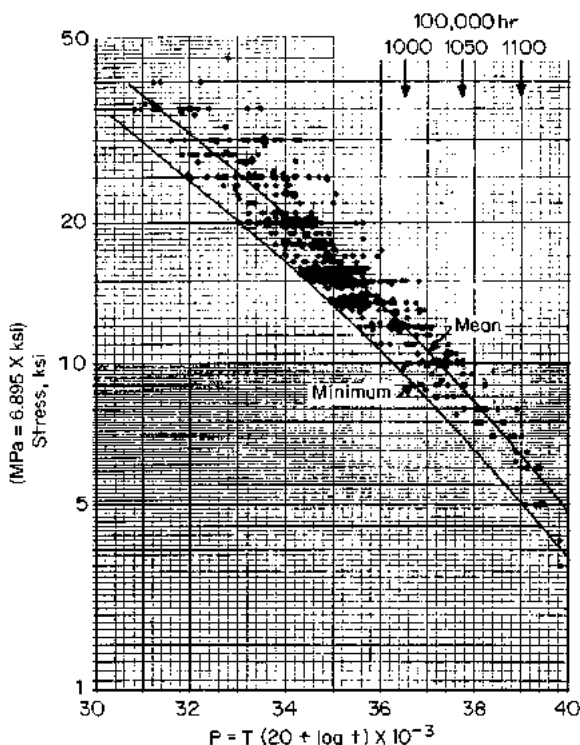
FIGURE A3.22 Variation of Larson-Miller parameter with stress for rupture of annealed 2¼ Cr-1 Mo steel. (Supplemental Report on the Elevated-Temperature Properties of Chromium-Molybdenum Steels, ASTM Data Series Publication DS 652.)
