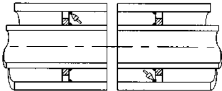
FIGURE B13.85e Weld the interstitial supports to the D of the secondary-containment pipe.
