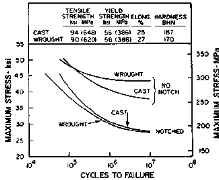
FIGURE A3.11 Fatigue characteristics ( S - N curve) for cast and wrought 1040 steel in the normalized and tempered condition, both notched and unnotched. R. R. Moore rotating beam tests, K_t = 2.2 . ( Atlas of Fatigue Curves , ASM.)
