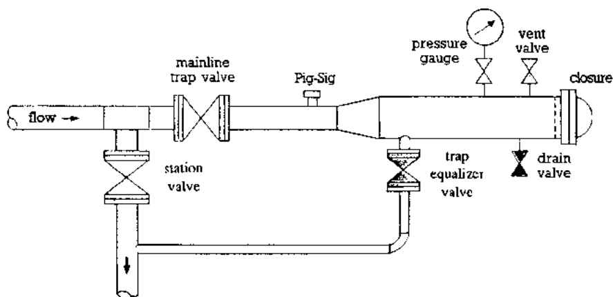
FIGURE C6.15 Launching and receiving scraper traps for gas service. (T.D. Williamson.)
