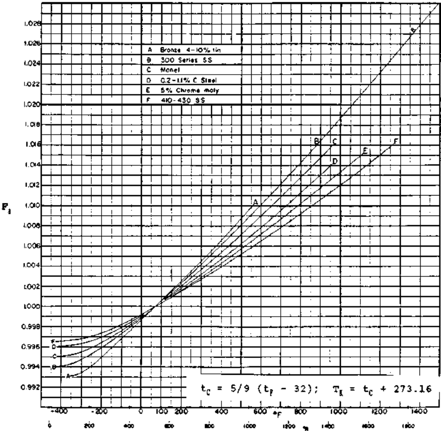
FIGURE B8.22 Area factors, F_A , for the thermal expansion of primary elements. (From Ref. 13.)
