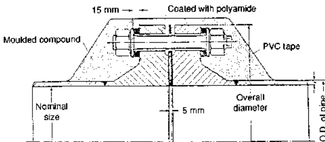
FIGURE C6.19 Insulating flange connection for laying in the ground. (Eisenbau Albert Ziegle KG.)
