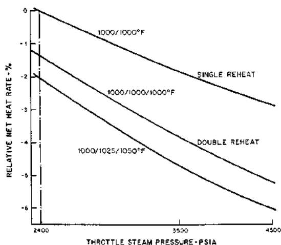
FIGURE C3.7 Effect of steam conditions on heat rate.
