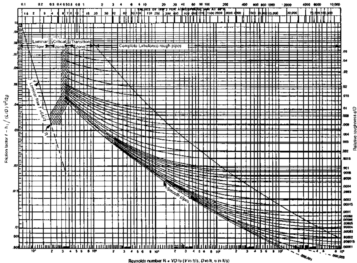
FIGURE C1.10 Moody diagram. Friction factors for any kind and size of pipe. ( Hydraulic Institute. )
