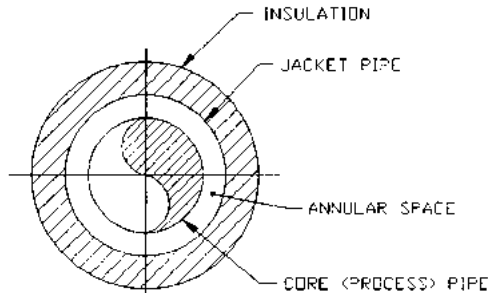
FIGURE C7.11 Heat transfer jacketed pipe.
