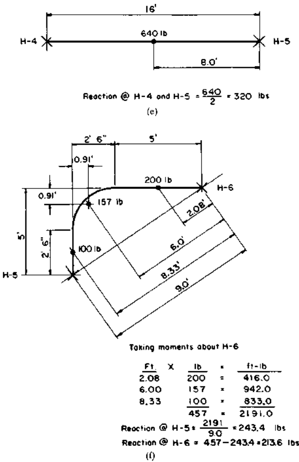
FIGURE B4.25 (e) Distribution of weight between H-4 and H-5. (f) Distribution of weight between H-5 and H-6.
