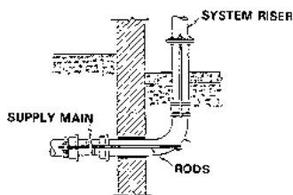
FIGURE C2.11 Typical fire protection riser restraint.
