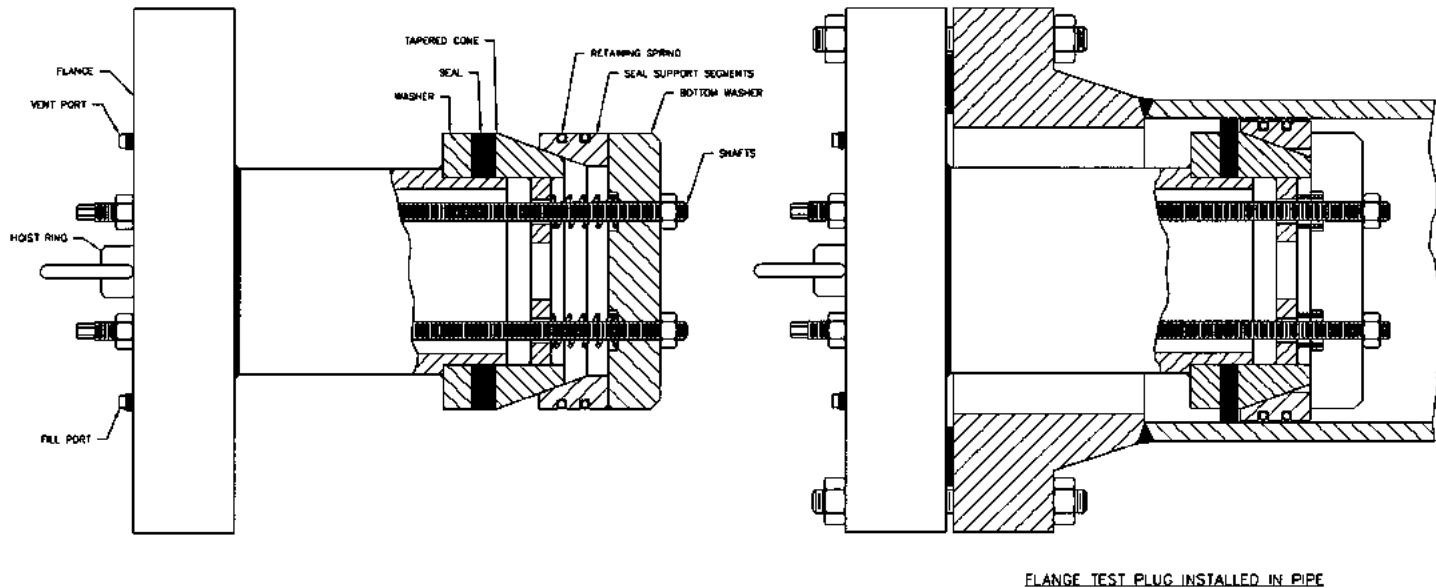
FIGURE B14.8a Special high lift flange test plug. (Courtesy of Expansion Seal Technologies, Harleysville, PA.)
