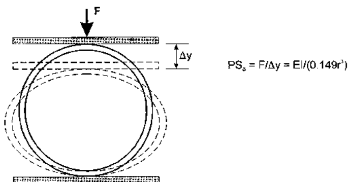
b. Pipe Bending Stiffness (Determined in Parallel Plate Test)
