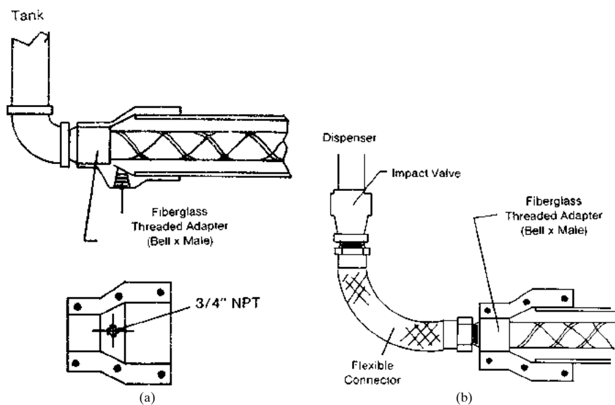
FIGURE B13.7 Examples of clam-shell fiberglass termination fittings: (a) termination concentric reducer with integral drain; (b) termination concentric reducer. (Source: Smith Fiberglass Products, Inc.)
