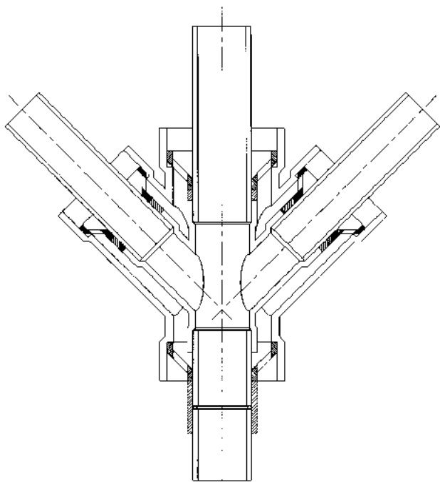
FIGURE B13.52 Rionlock™ thermoplastic restrained 45° double reducing lateral (wy) using molded code approved carrier fitting. ( Patent Pending; Orion Fittings, Inc. )
