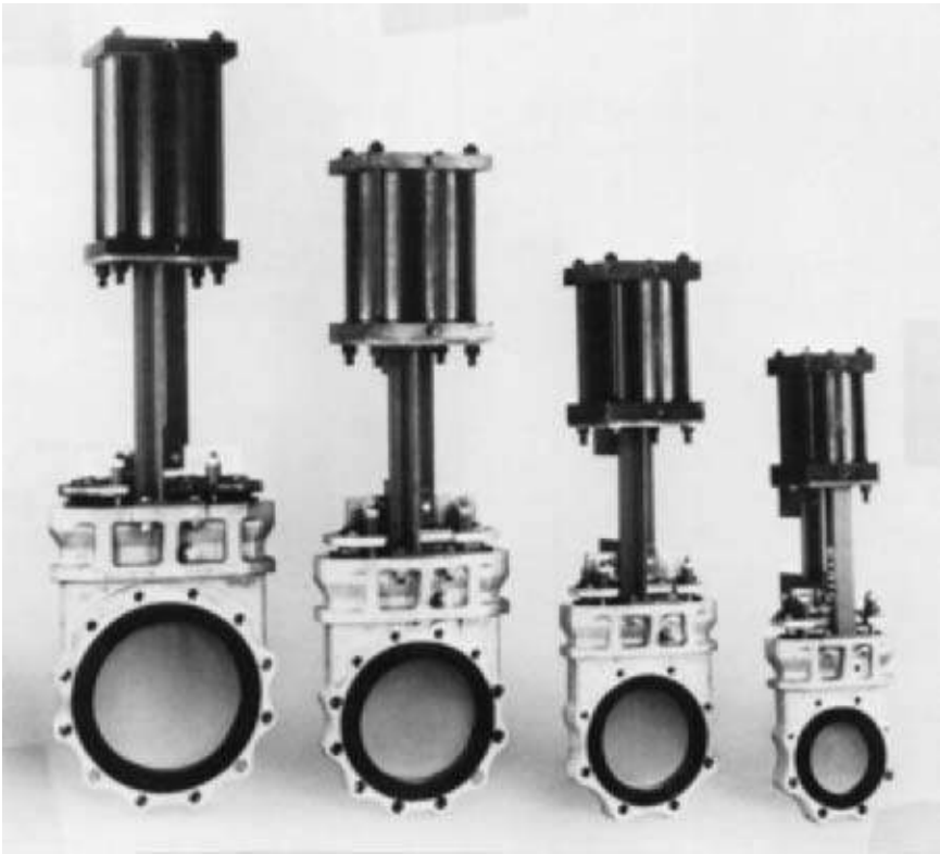
FIGURE C14.14 Knife gates for sluice service photograph (UCC).
