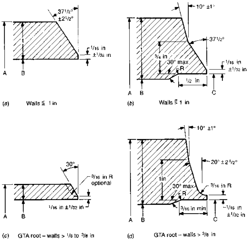
FIGURE A6.15 Typical weld end bevels. (a) Walls \leq 1 in; (b) walls > 1 in; (c) GTA root walls > \frac{1}{8} to \frac{3}{8} in; (d) GTA root walls > \frac{3}{8} in.
