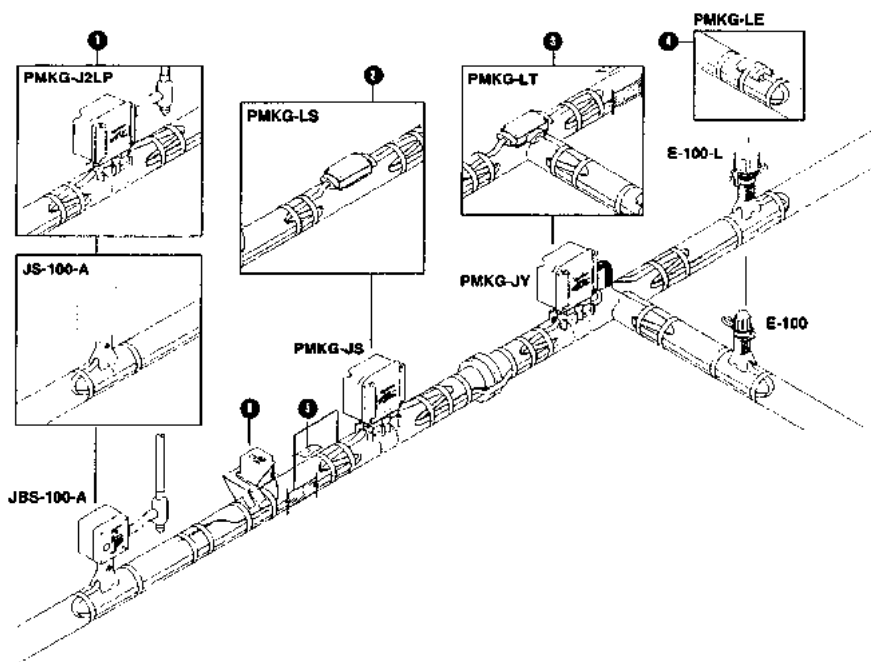
FIGURE B6.16 Component selection guide. (Raychem Design Guide, Raychem Corp., Menlo Park, CA, © 1998.)
