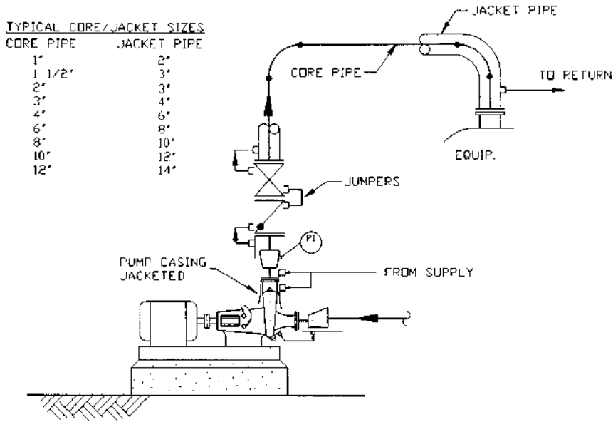
FIGURE C7.12 Jacket liquid phase—circuitry.
