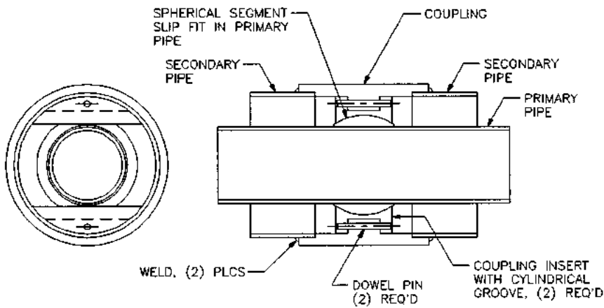
FIGURE B13.26 Illustration of an internally guided ball-type flexibility support. The version shown is designed to use in an all-welded system. Variations are also available that are intended for use in systems with a mechanically joined outer jacket. (U.S. Patent Nos. 5,901,753; 5,862,834 and 5,197,518; Orion Fittings, Inc.)
