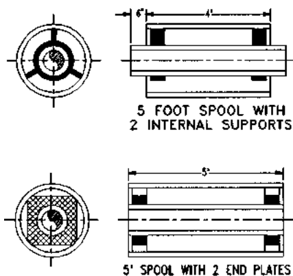
FIGURE B13.4 Example of factory prefabricated 5-ft lengths of piping showing support spacing based on 5-ft spacing. (Orion Fittings, Inc., Kansas City, KS)
