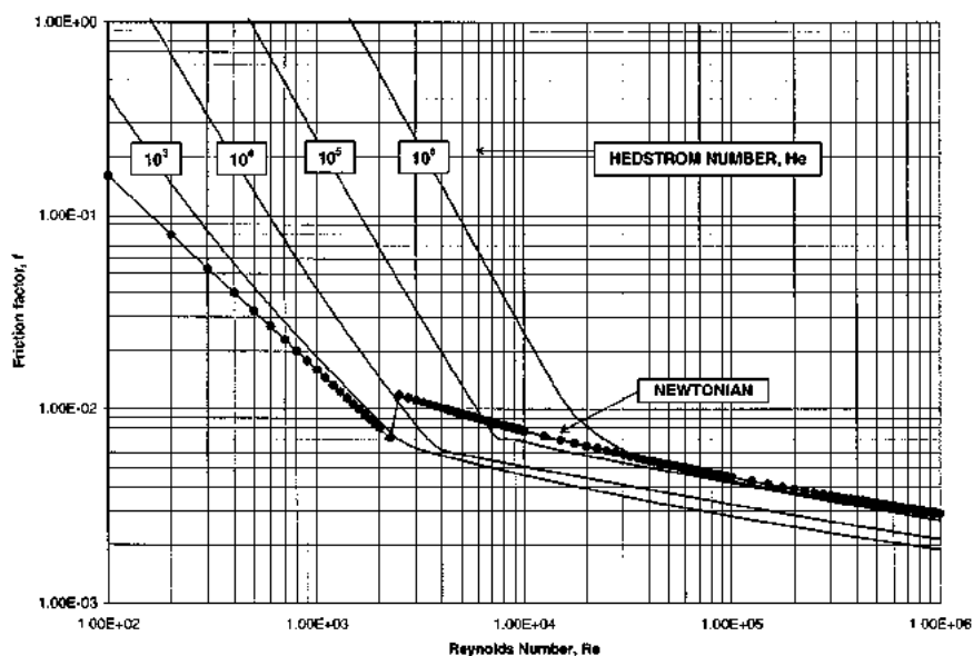
FIGURE C11.7 Friction factor f as a function of Reynolds number for Bingham plastic slurries, Re = \rho D V / (\eta g_c) , He = D^2 \rho \tau_y / (\eta g_c) , where D = pipe ID (ft), V = velocity (ft/s), \rho = density (lb/ft 3 ), \eta = viscosity (lbf-s/ft 2 ), \tau_y = yield stress (lbf/ft 2 ), g_c = 32.2 lb-s/(lbf-ft 2 ).
