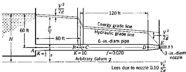
FIGURE C1.11 Hydraulic and energy grade lines.
