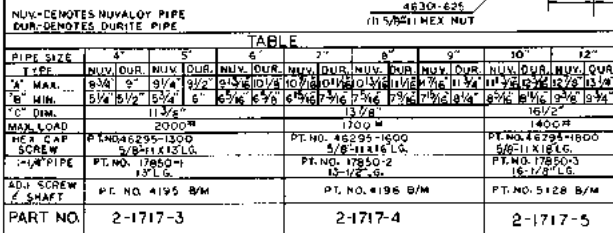
FIGURE C14.21 Roller support.
