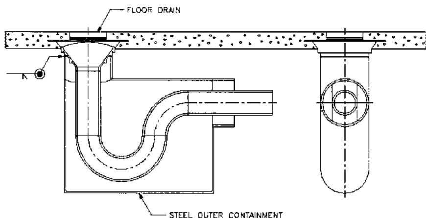
FIGURE B13.63 Fabricated double containment P-trap incorporating a cleanout, where the system uses metallic or thermoplastic butt welding/fusion pattern pressure fittings as the basis to fabricate a non-plumbing-code approved drainage system.
