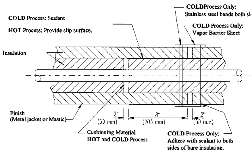
FIGURE B7.8 Cross-section of a contraction control joint.
