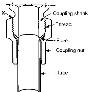
FIGURE C13.11 Piping systems.
