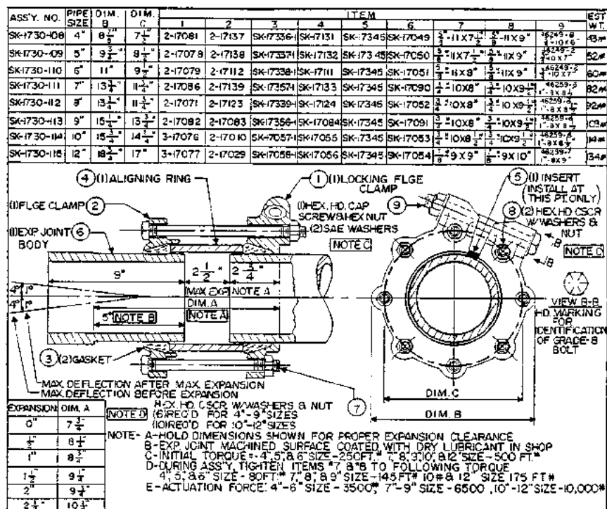
FIGURE C14.17 Cross section of sleeve-type expansion joint (UCC).
