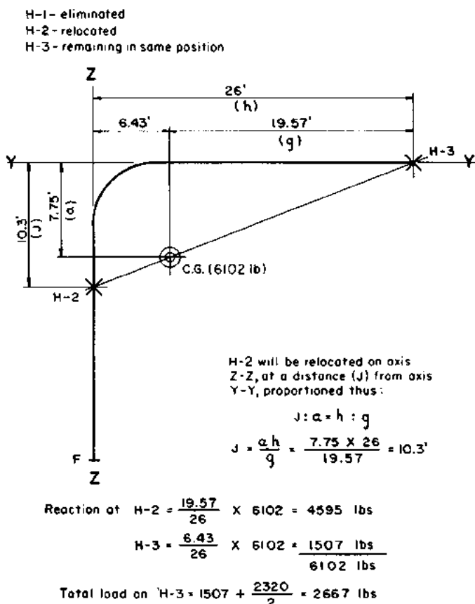
FIGURE B4.21 Hanger load calculations for system of Fig. B4.19 except that one hanger has been eliminated.
