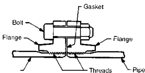
FIGURE C13.9 Flanged joint.
