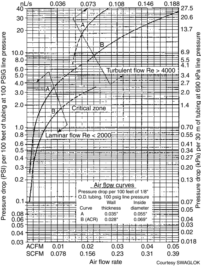
FIGURE C16.6 Compressed-air sizing chart. 1/8 in (3 mm) copper tubing 100 psig [700 kPa].
