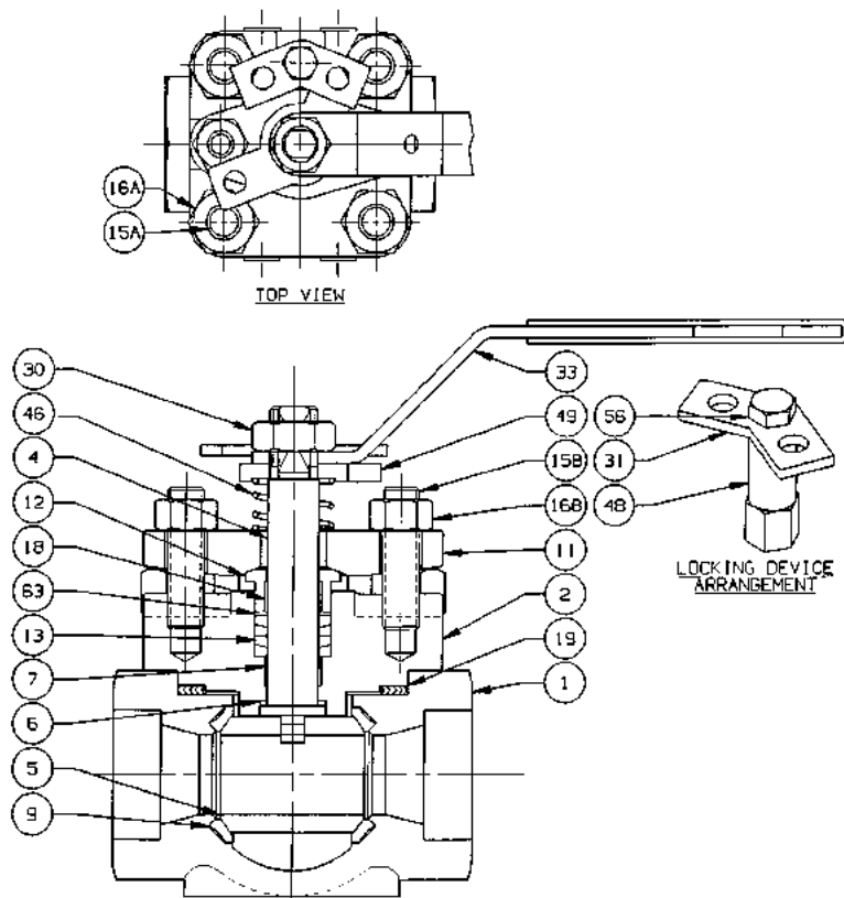
FIGURE A10.23 Ball valves, top entry, regular port, socket weld ends. (Courtesy of Velan.)
