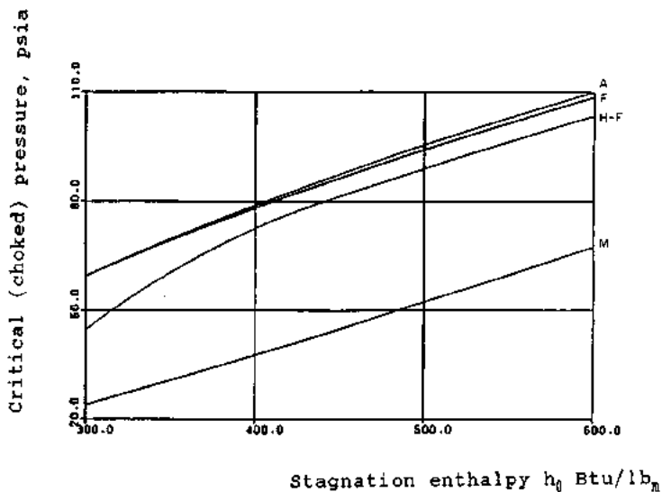
FIGURE B8.48 Predicted critical pressure versus stagnation enthalpy. Mass flux = 600 \text{ lb}_m/(\text{ft}^2 \cdot \text{s}) (Stone & Webster data.)
