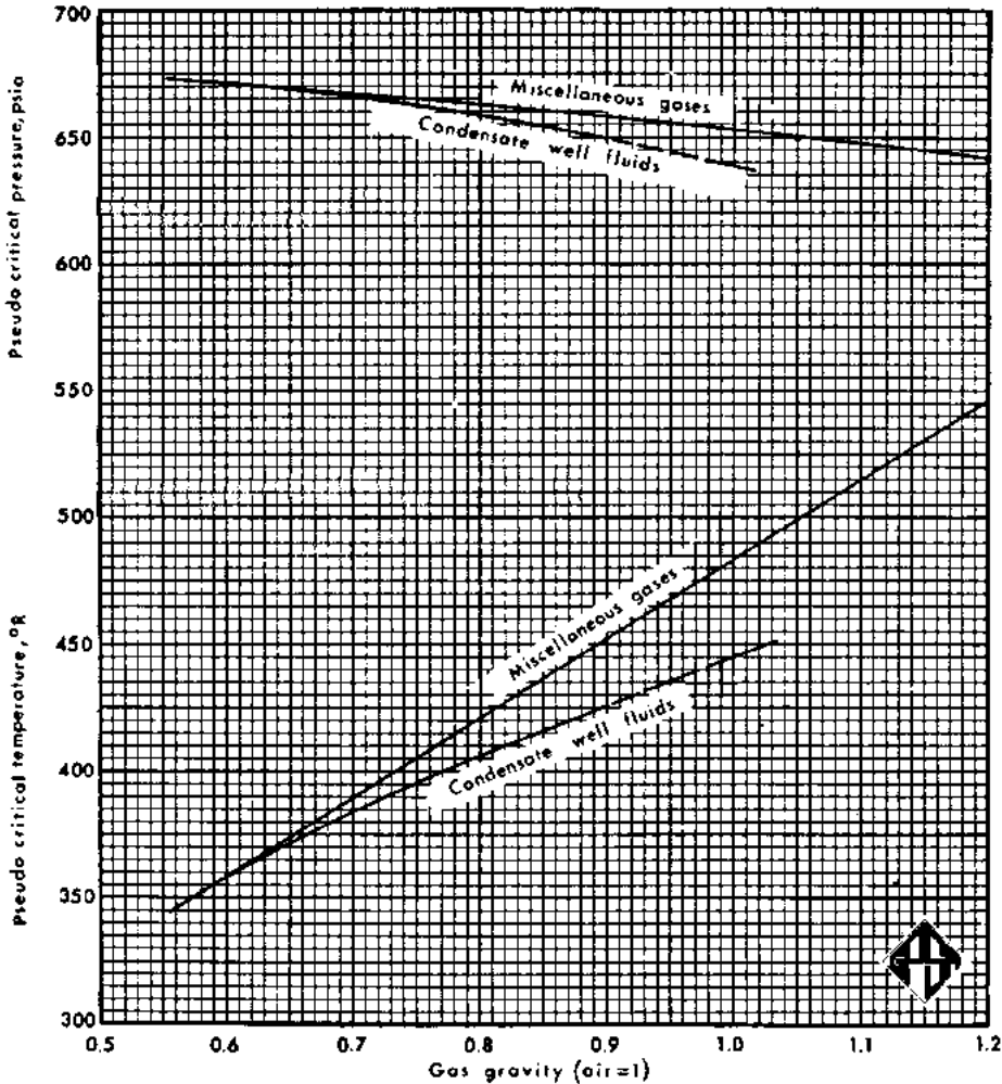
FIGURE C6.3 Pseudocritical properties of natural gases. (Gas Processors Suppliers Association Engineering Data Book.)
