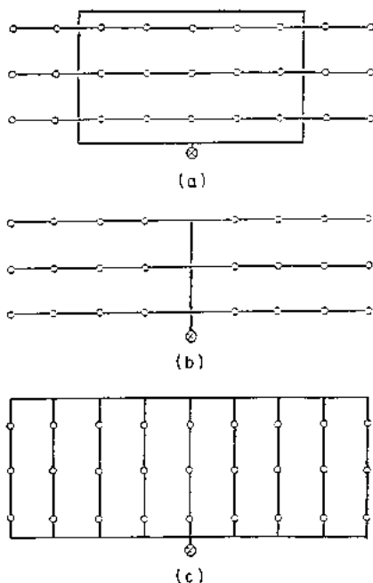
FIGURE C2.10 Typical sprinkler system piping layouts: (a) grid; (b) tree; (c) loop.
