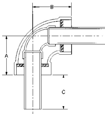
FIGURE B13.34 Typical thermoplastic 90° elbow combination for parts using socket-type joining systems whereby the carrier elbow is a single 90° elbow. ( Orion Fittings, Inc. )
