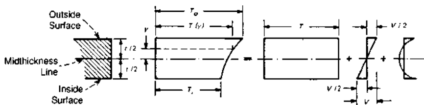
FIGURE B4.4 Decomposition of temperature distribution range. (Figure NB-3653.2(b)-1, Section III, Division I, ASME B & PV Code, 1989. Courtesy of ASME.)
