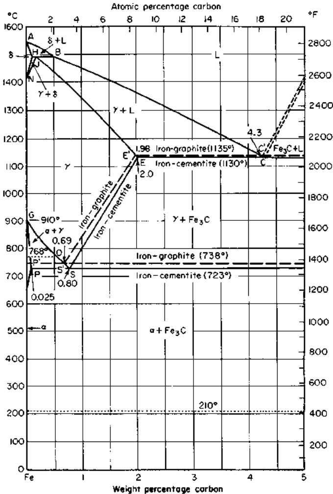
FIGURE A3.18 Iron-carbon equilibrium diagram.
