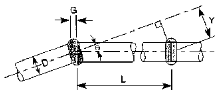
FIGURE A9.15 Angular movement.
