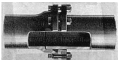
FIGURE A2.30 Mechanical (gland-type) joint for cast-iron pipe.
