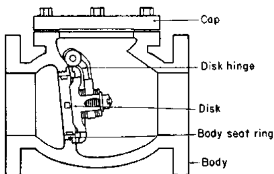
FIGURE A10.14 Swing check valve.
