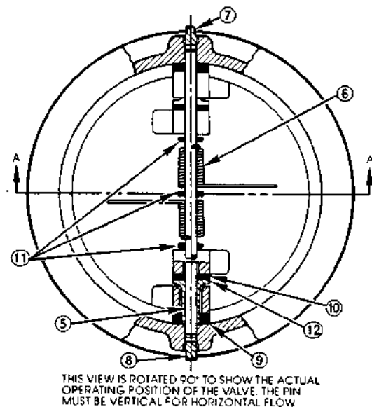
FIGURE A10.18 Folding-disc check valve.
