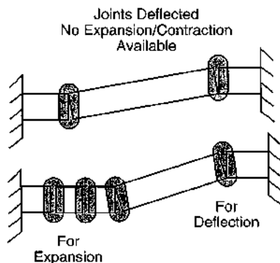
FIGURE A9.18 Accommodating piping expansion and deflection.
