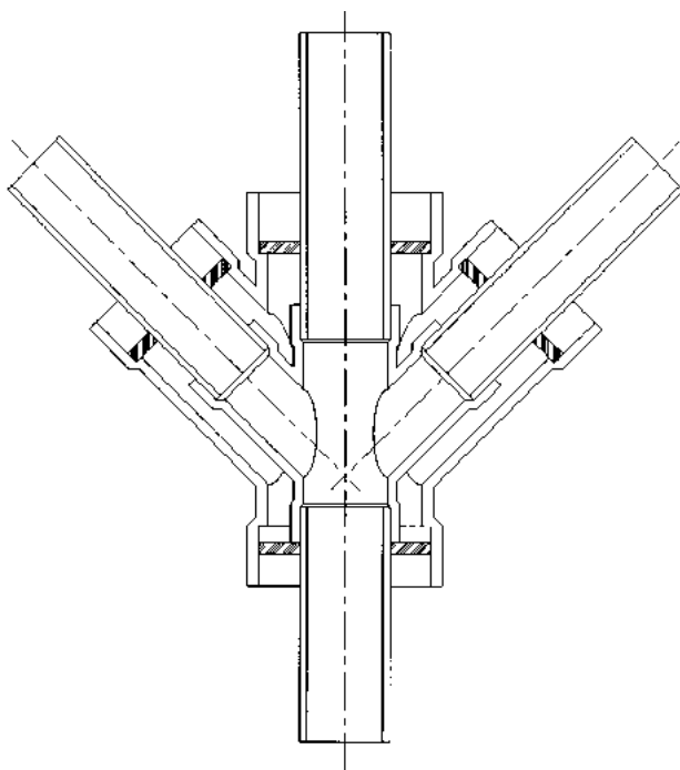
FIGURE B13.51 Example of thermoplastic 45° double reducing lateral (wye) using molded code approved carrier fitting. ( Orion Fittings, Inc. )
