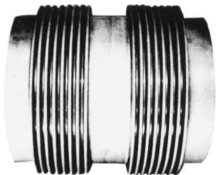
FIGURE A2.13 Metal bellows expansion joint.
