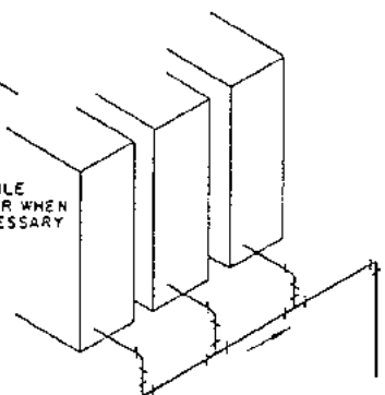
C MULTIPLE EVAPORATORS ON SAME LEVEL - COMPRESSOR BELOW
