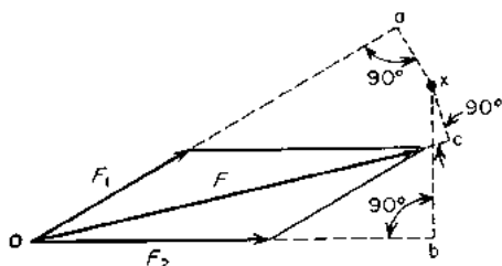
FIGURE A1.24 Vectors and moments.
