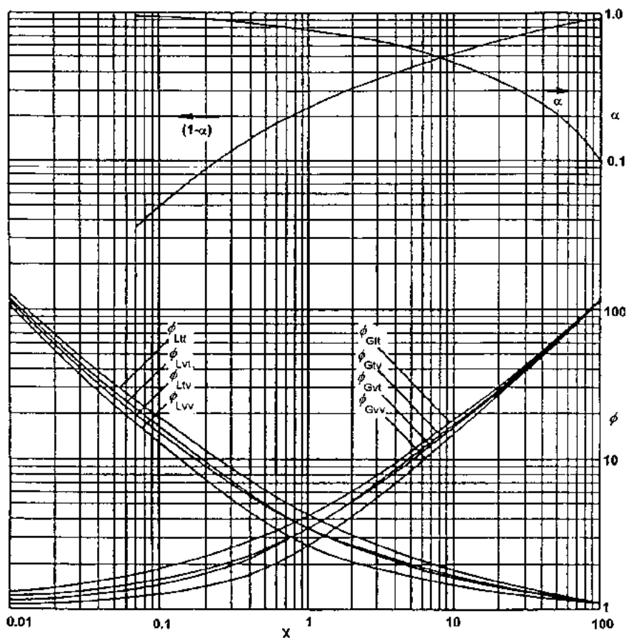
FIGURE C8.5 Lockhart-Martinelli correlation.
