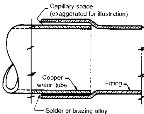
FIGURE C13.5 Soldered joint.
