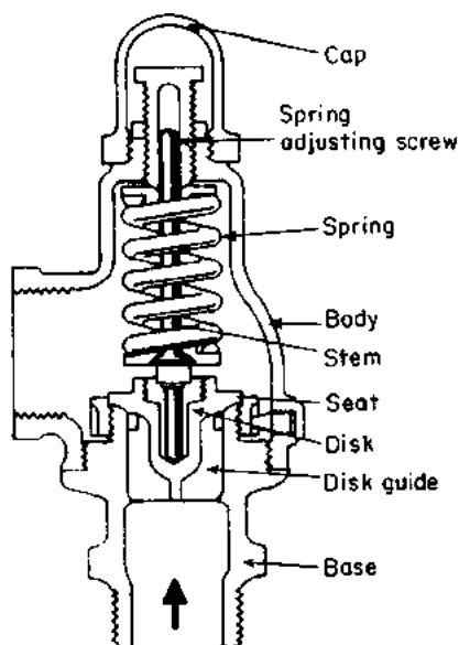
FIGURE A10.33 Relief valve opens when line pressure exceeds preset loading on the spring.
