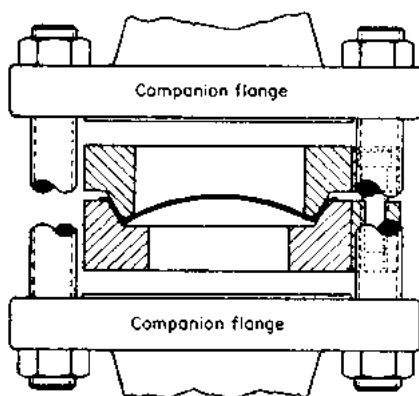
FIGURE A10.4 The rupture disc, a type of relief device.
