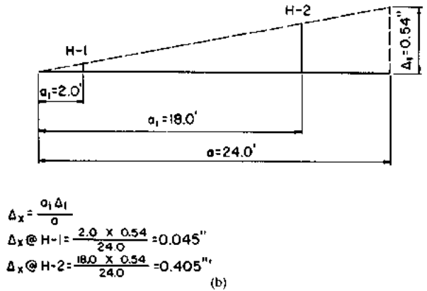
FIGURE B4.26 (a) Deflections of vertical leg of Fig. B4.24. (b) Determination of deflections at H-1 and H-2 of Fig. B4.24.
