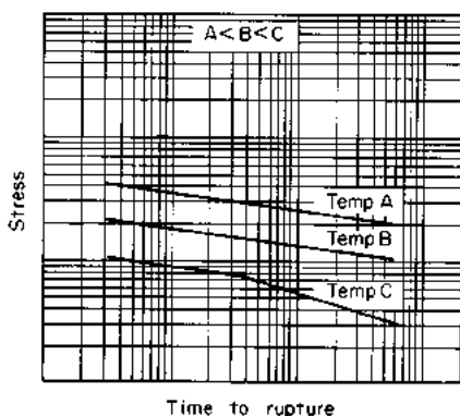
FIGURE A3.14 Typical stress-to-rupture curves.
