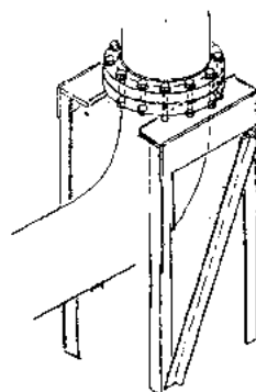
FIGURE D2.9 Typical support details. Pipe can move laterally and axially. (Illustrations courtesy of Smith Fiberglass Products, Inc., Ameron Fiberglass Pipe Systems, and Fibercast Co.)
