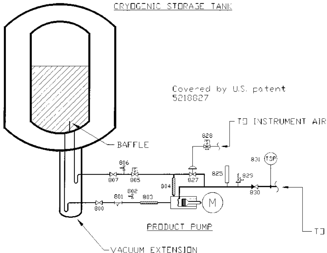
FIGURE C8.13 Thermosiphon prime system for cryogenic pumps. (Courtesy of Praxair, Inc.)
