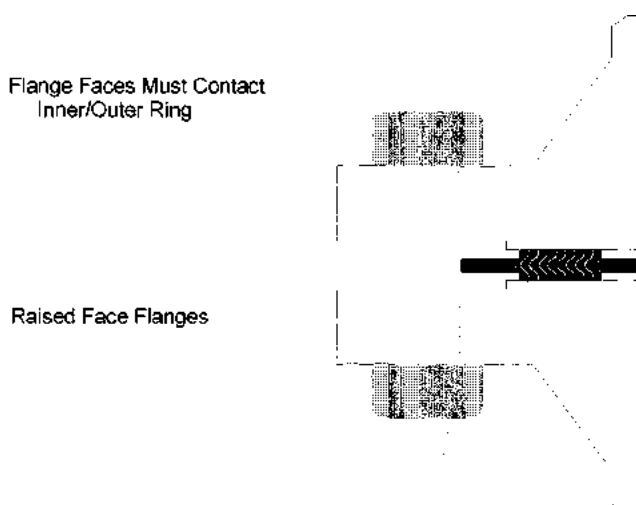
FIGURE A7.10 Typical flange gasket arrangement.
