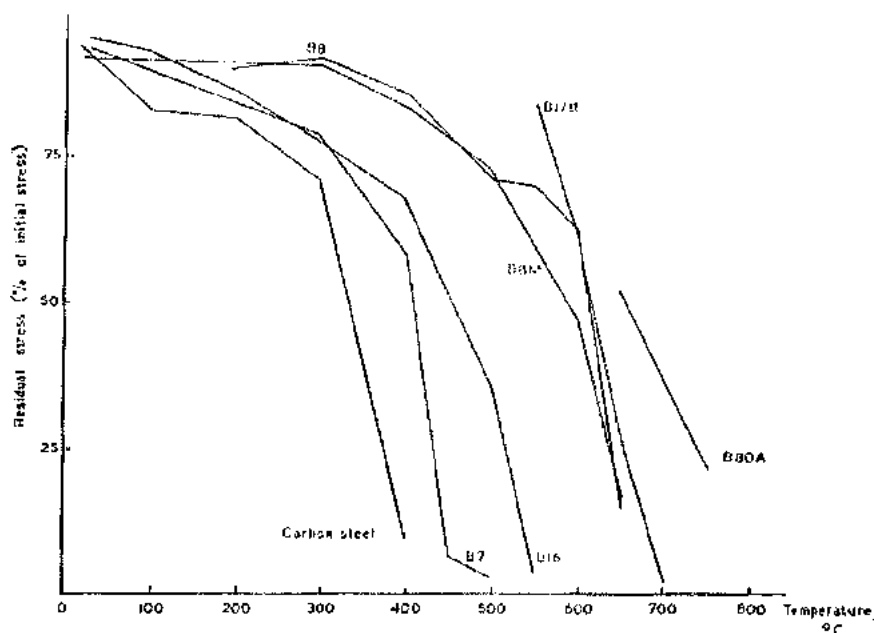
FIGURE A7.18 Stress relaxation behavior of various bolting materials showing percentage of initial stress retained at 1000 hours.
