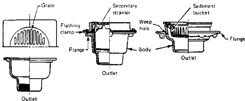
FIGURE C13.15 Typical floor drains.
