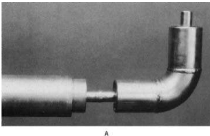
FIGURE B13.78a Illustration of a gap in a double-containment pipe. (Source: Guardian division of Eslon Thermoplastics, Inc.)
