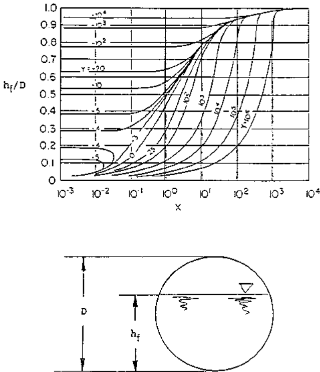
FIGURE B8.36 Equilibrium liquid level as a function of the dimensionless groups X and Y . (From Ref. 26.)
