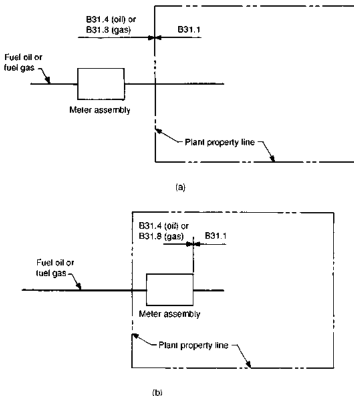
FIGURE A4.3 Jurisdiction of ASME B31.1, B31.4, and B31.8 Over Fuel Gas and Fuel Oil Piping.
