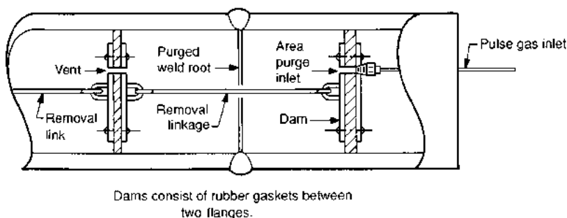
FIGURE A6.20 Typical shop purging arrangement.
