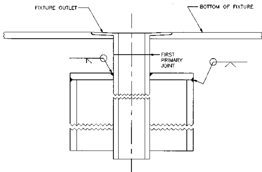
FIGURE B13.60 Configuration for fixture outlets where the first carrier joint is above the level of the secondary containment jacketing. In this type of arrangement, a leak at this joint could escape around the secondary containment pipe.
