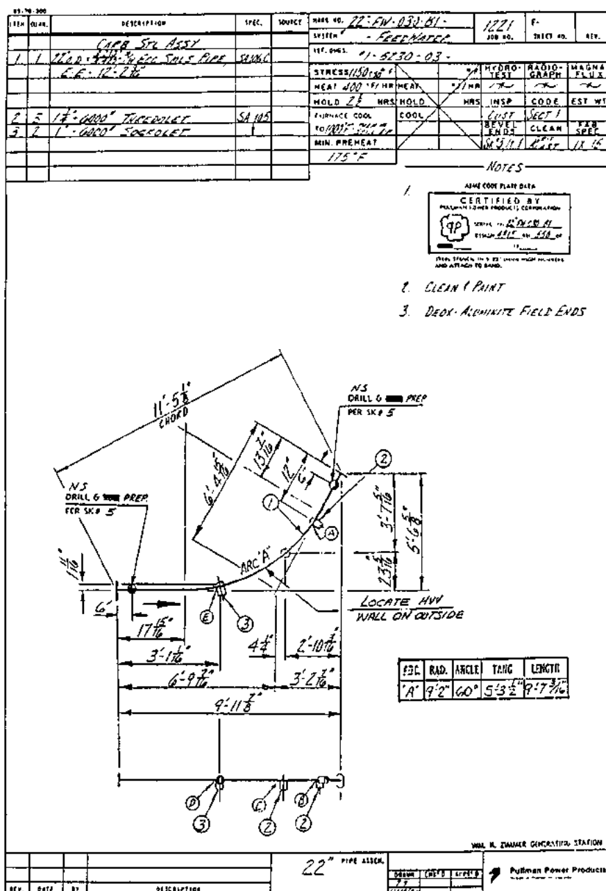
FIGURE A6.3 Dimensioning a bend. (Pullman Power Products Corporation)
