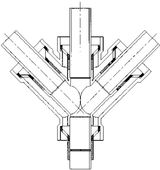
FIGURE B13.50 Rionlock™ thermoplastic restrained 45° double lateral (wy) using molded code approved carrier fitting. ( Patent Pending; Orion Fittings, Inc. )
