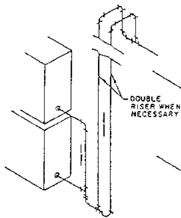
B ALTERNATE FOR MULTIPLE EVAPORATORS STACKED ON SAME LEVEL - COMPRESSOR ABOVE ARRANGEMENT A PREFERRED
