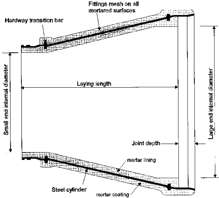
FIGURE A8.6 Typical concentric reducer fitting.
