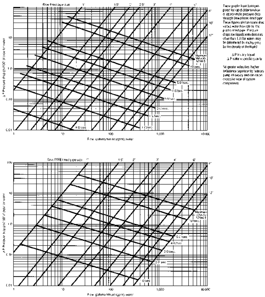
FIGURE B12.7 Pressure-drop curves for PP, PVDF, and PTFE-lined pipe. (Courtesy of Crane Resistoflex).
