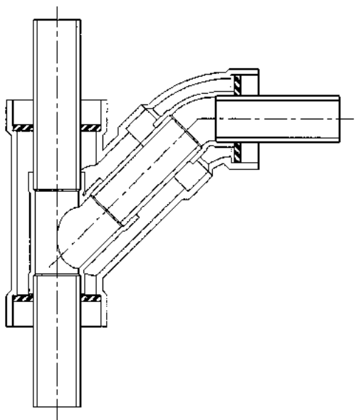
FIGURE B13.45 Example of thermoplastic long-turn wye using molded code approved carrier fitting. ( Orion Fittings, Inc. )
