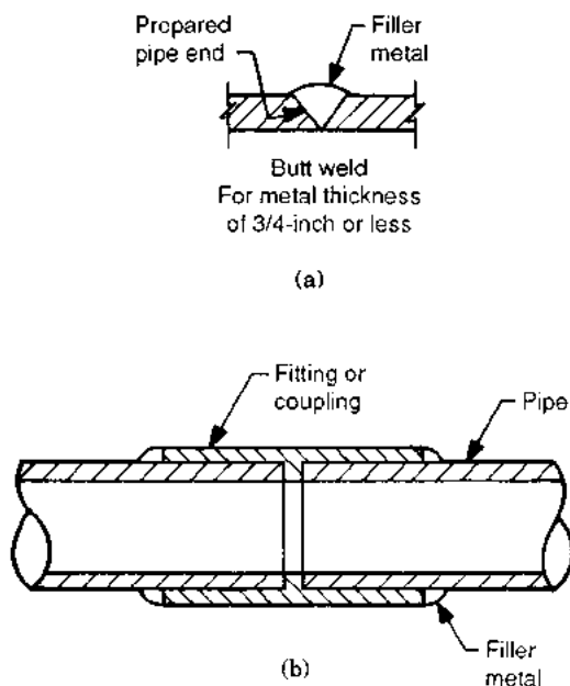
FIGURE C13.10 (a) Butt-weld joint. (b) Socket weld joint.
