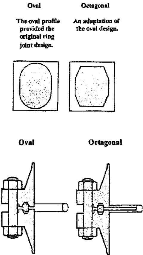
FIGURE A7.6 Style R (oval and octagonal) and RX gaskets.
