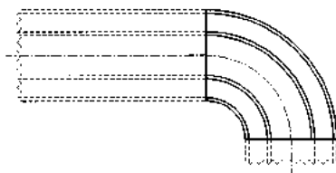
FIGURE B13.30 Example of an elbow where the inner and outer radii are equal throughout their curved portion.
