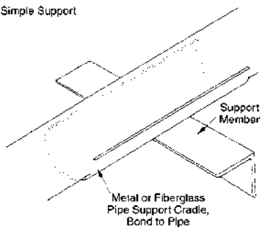
A. Simple Support
