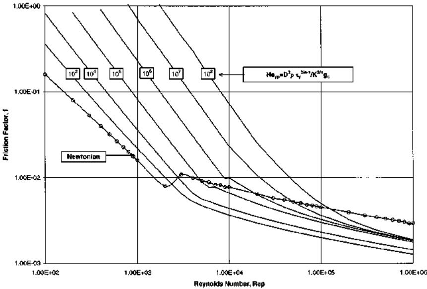
FIGURE C11.9a Friction factor f as a function of Reynolds number for yield pseudoplastic slurries for n = 0.7 , He = [D^3 \rho \tau_y (t_s/K)^{2n-2}] / (K^2 g_c) , Re = 8 \rho D^n V^{2-n} [n / (2 + 6n)]^n / (K g_c) , where D = pipe ID (ft), V = velocity (ft/s), \rho = density (lb/ft 3 ), K = consistency (lb \cdot s n /ft 2 ), \tau_y = yield stress (lb/ft 2 ), g_c = 32.2 lb \cdot s/(lb \cdot ft 2 ).
