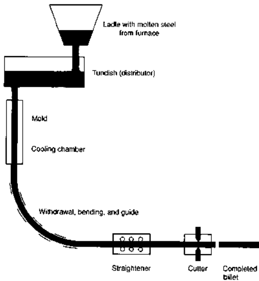
FIGURE A5.2 Continuous casting process.
