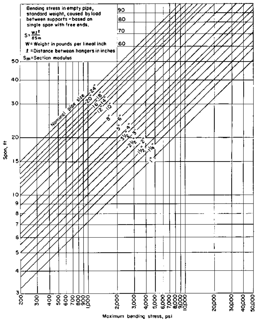
FIGURE B4.16 Bending stress in empty pipe.
