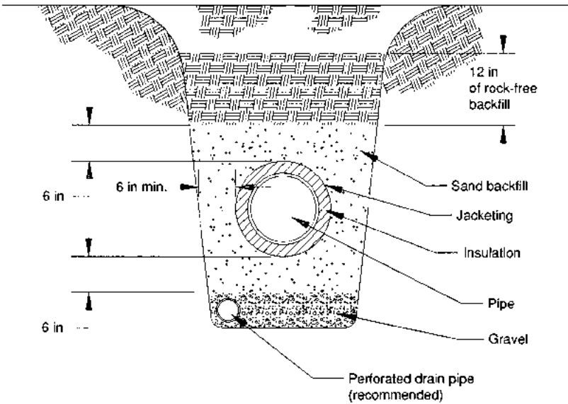
FIGURE B7.10 Backfill detail.
