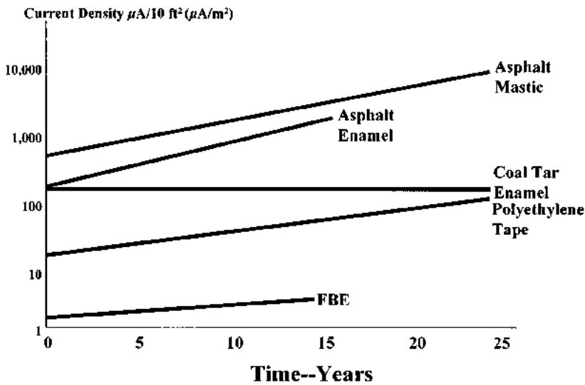
FIGURE B10.1 Lifetime pipeline costs are significantly impacted by the amount of cathodic protection current required to protect the pipe. FBE coatings provide an operational cost savings. 15
