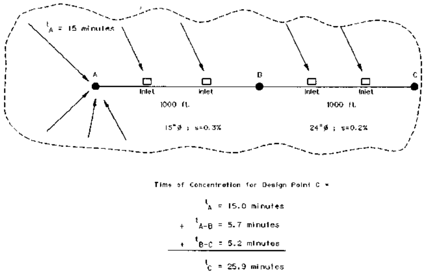
FIGURE C12.2 Calculation of time of concentration.
