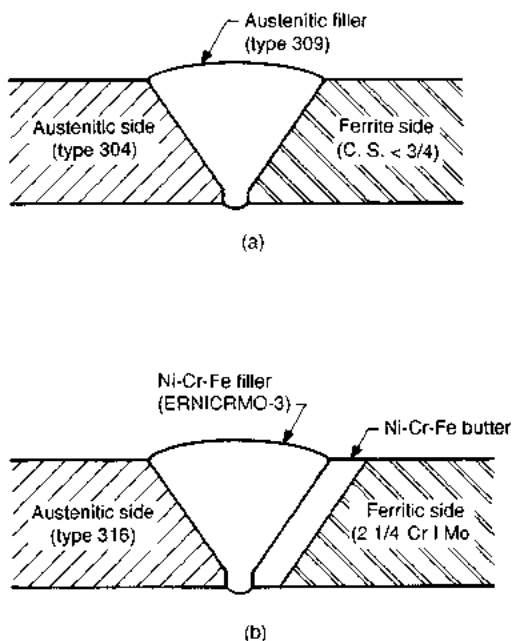
FIGURE A6.21 Dissimilar metal welds. (a) For moderate temperature service; (b) for high-temperature services or where stress relief on the ferritic side is required.
