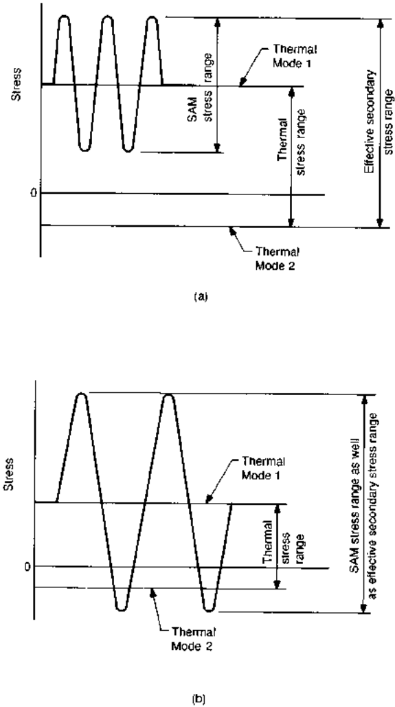
FIGURE B4.11 Effective secondary stress range.
