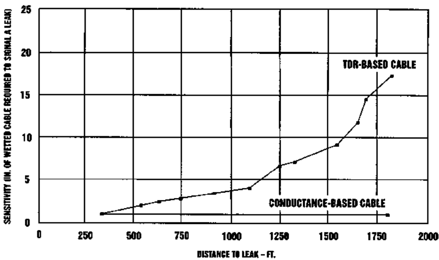
FIGURE B13.89 Sensitivity of a typical TDR-based cable based on the length down the cable where a leak occurs. (Source: Based on test data supplied by Raychem Corp.)
