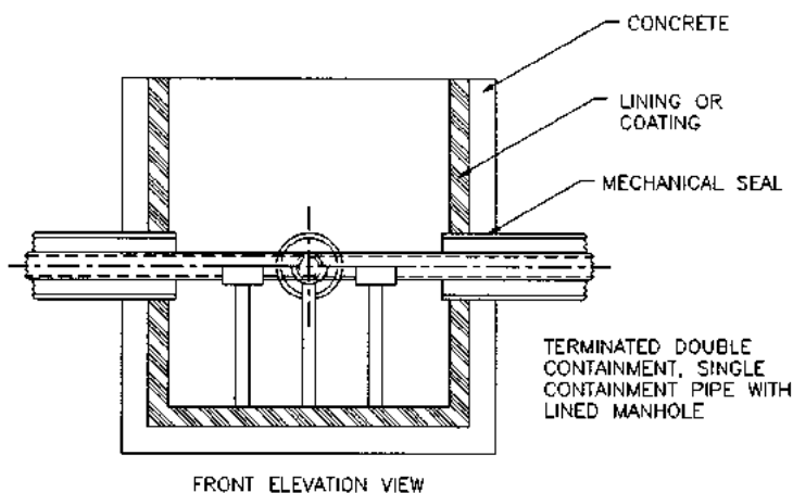
FIGURE B13.71b Front elevation details for MH01 from Fig. B13.69.
