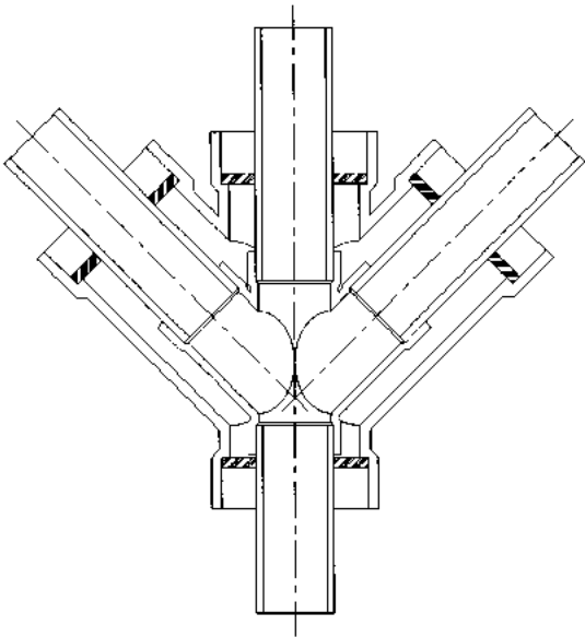
FIGURE B13.49 Example of thermoplastic 45° double lateral (wy) using molded code approved carrier fitting. ( Orion Fittings, Inc. )
