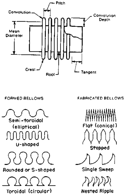
FIGURE B4.6 Bellows expansion joints.
