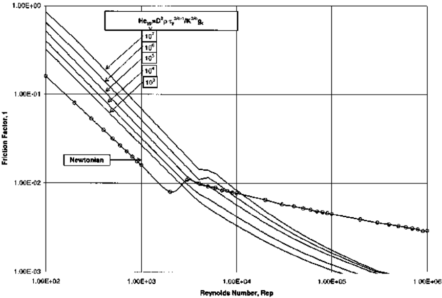
FIGURE C11.9c Friction factor f as a function of Reynolds number for yield pseudoplastic slurries for n = 0.3 , He = [D^2 \rho \tau_y (t_y/K)^{2n-2})]/(K^2 g_c) , Re = 8 \rho D^n V^{2-n} [n/(2 + 6n)]^n / (K g_c) , where D = pipe ID (ft), V = velocity (ft/s), \rho = density (lb/ft 3 ), K = consistency (lb \cdot s n /ft 2 ), \tau_y = yield stress (lb/ft 2 ), g_c = 32.2 (lb \cdot s/(lb \cdot ft 2 )).
