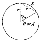
FIGURE A1.25 Length of arc and chord.
