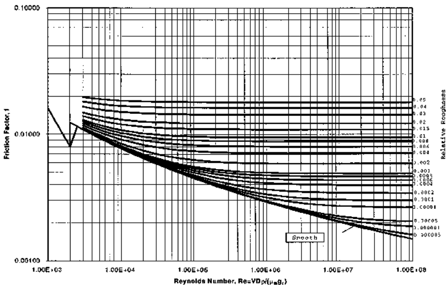
FIGURE C11.6 Friction factor f as a function of Reynolds number for newtonian slurries, where D = pipe ID (ft), V = velocity (ft/s), \rho = density (lb/ft 3 ), \mu = viscosity (lb·s/ft 2 ), g_c = 32.2 \text{ lb·s/(lb·ft}^2\text{)} .
