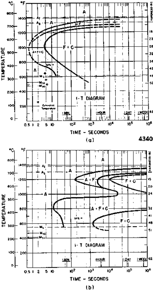
FIGURE A3.19 Isotherm transformation diagrams for AISI 1050 (a) and AISI 4340 (b). (From I-T Diagrams, United States Steel, ©1963.)
