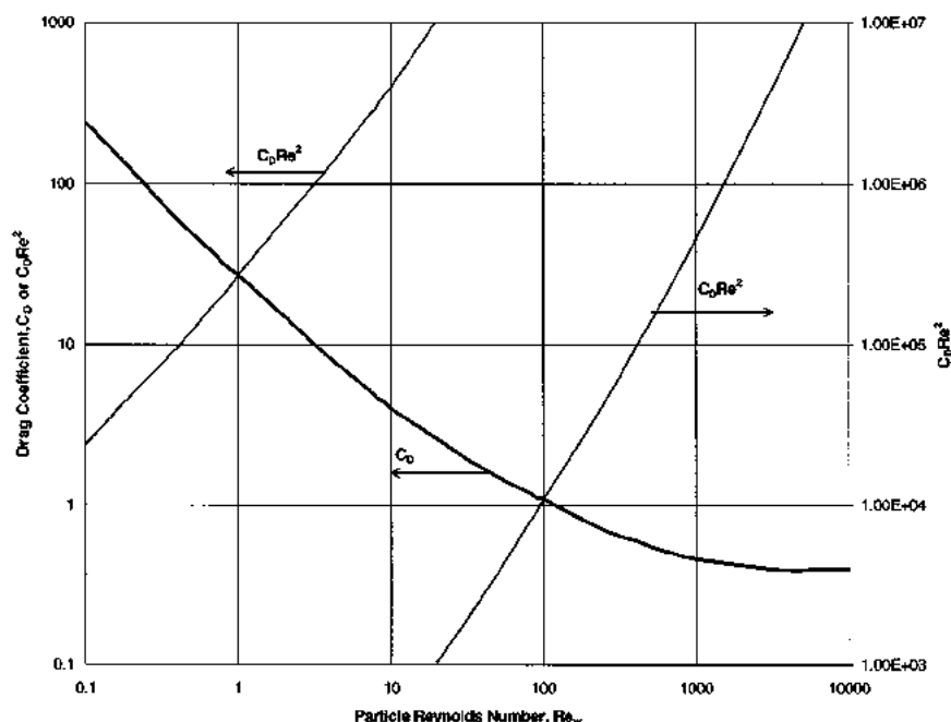
FIGURE C11.13 Drag coefficient C_D of spherical particles settling in liquid. C_D = 4gd(\rho_s - \rho_l)/[3W_o^2\rho_l] , where d = particle diameter (ft), w_o = settling velocity (ft/s), g = acceleration due to gravity (32.2 ft/s 2 ), \rho_s = particle density (lb/ft 3 ), \rho_l = liquid density (lb/ft 3 ).
