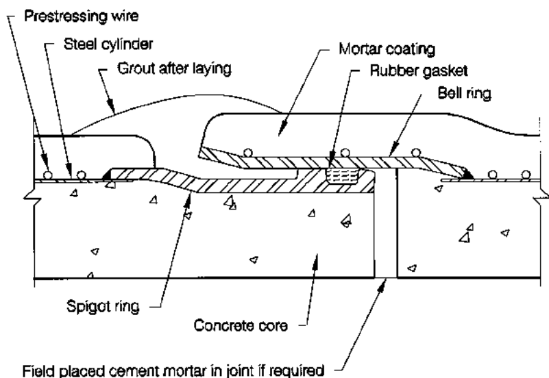
FIGURE B9.1 Mortaring of interior joint recess for prestressed concrete cylinder pipe.
