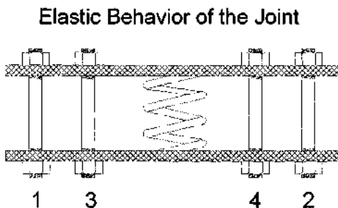
FIGURE A7.15 Elastic behavior of simplified 4-bolt flange.
