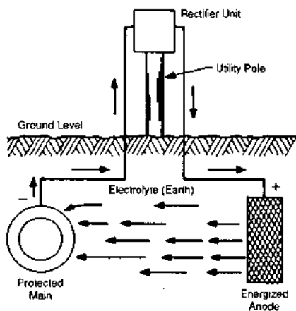
FIGURE C6.18 Additional current for cathodic protection requires use of a rectifier. ( Pipeline & Gas Journal , February 1984.)
