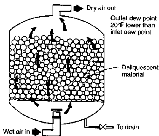
FIGURE C15.8 Solid-type desiccant dryer.
