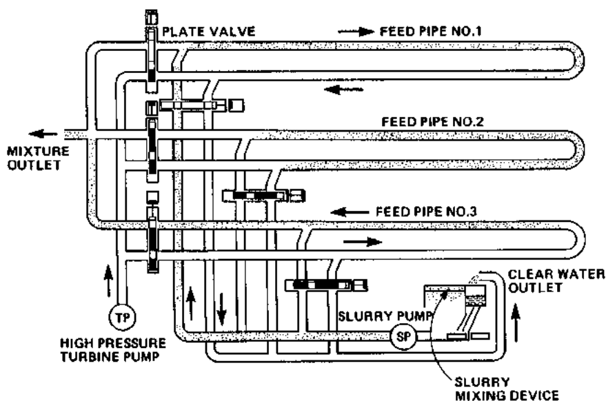
FIGURE C11.21 Sketch of a hydrohoist.
