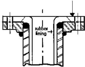
FIGURE B11.11 Flange face rubber lining.
