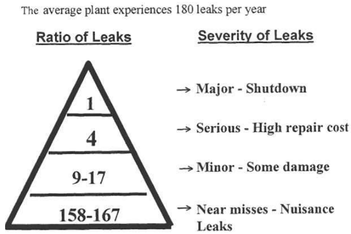
FIGURE A7.1 Industry leak study (PVRC Study, July 1985).
