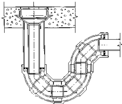
FIGURE B13.58 Example of a thermoplastic double containment floor drain with factory pre-assembled P-trap outlet. ( Orion Fittings, Inc. )
