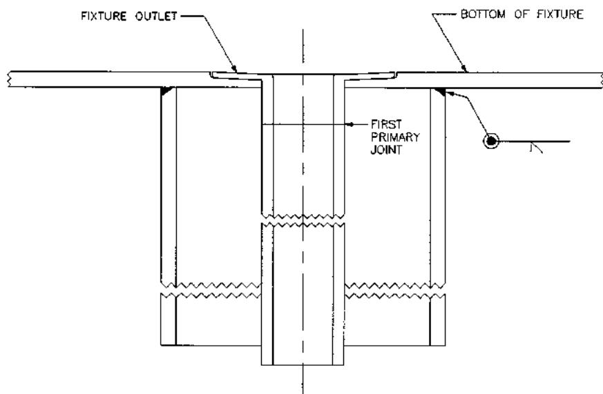
FIGURE B13.59 Configuration for fixture outlets where the first carrier joint is below the level of the secondary containment jacketing.
