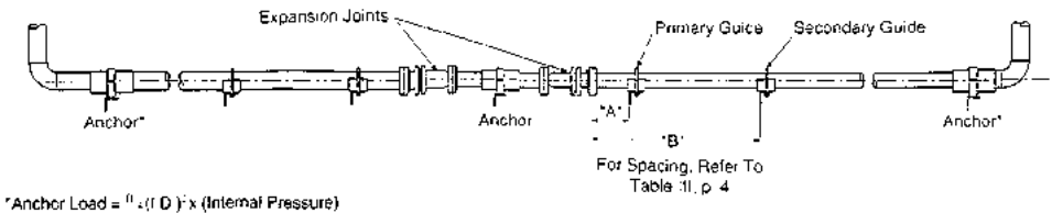
FIGURE D2.14 Typical expansion joint installation.
