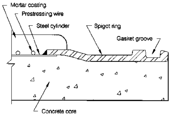
FIGURE A8.1 Spigot ring.
