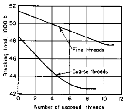
FIGURE A2.21 Comparison of proof strength of fine and coarse threads, SAE Grade 5, ¾-in bolts.
