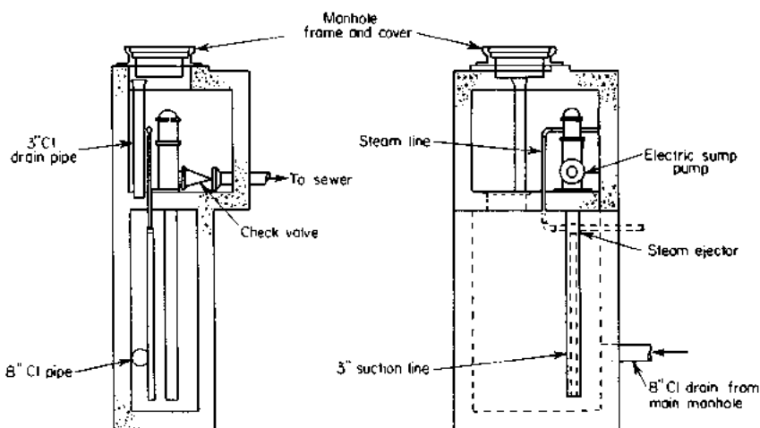
FIGURE C3.17 Manhole for sump pump.
