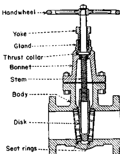
FIGURE A10.2 Nonrising stem gate valve for 250-psig steam service.
