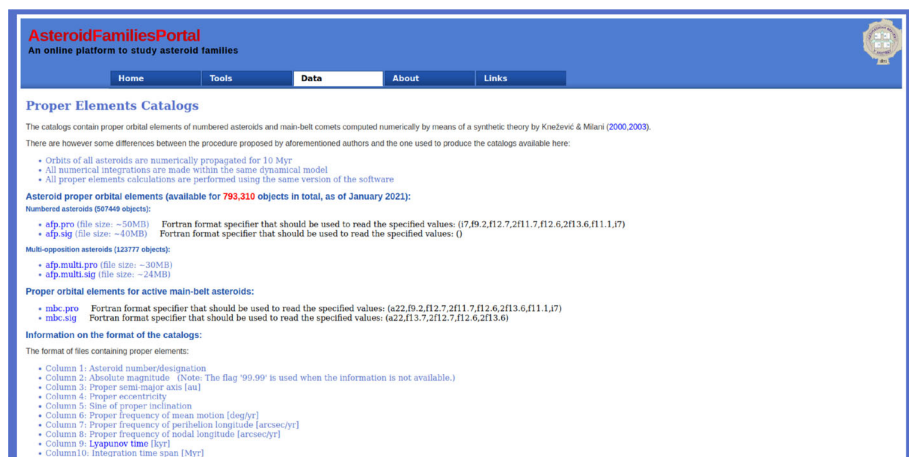
Fig. 2 Snapshot of the Proper Elements page at the Asteroid Families Portal. The page is available at: http://asteroids.matf.bg.ac.rs/fam/properelements.php
