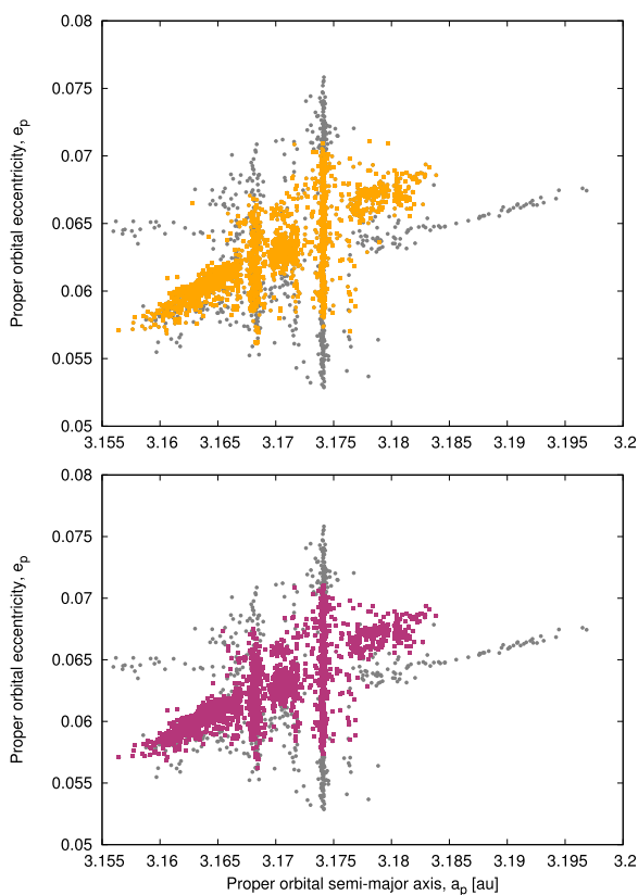
Fig. 1 Identification of Veritas family members using different methods and different catalogues. In both panels, grey circles represent the family members identified by the classical HCM approach applied to the catalogues containing \sim 793\text{k} objects, respectively, and using the cut-off of 18\text{ m s}^{-1} . Orange (upper panel) and magenta (lower panel) squares represent the members attached to the family from the more extensive catalogue, to the members initially identified with the classical HCM at 18\text{ m s}^{-1} applied to the smaller catalogue with \sim 507\text{k} records. The upper panel (orange squares) are objects attached by the ExtraTrees ML-based algorithm with a hyperparameter ( number of estimators ) equal to 41 (Carruba et al. 2020a). In the lower panel (magenta squares) are shown members attributed to the family with the single 18\text{ m s}^{-1} step HCM approach (Milani et al. 2014)
