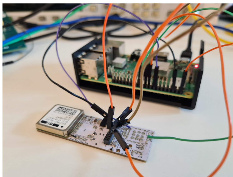
Figure 26: Assembled PCB connected to a Raspberry Pi micro controller . There is another Raspberry Pi micro controller emulating a PEV that is not seen in the picture.
