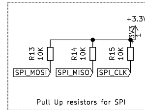
Pull Up resistors for SPI
