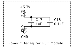
Power filtering for PLC module
