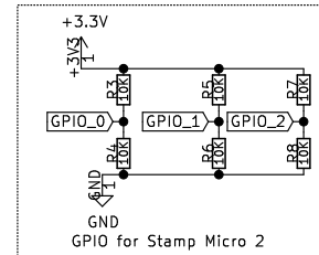
GPIO for Stamp Micro 2
