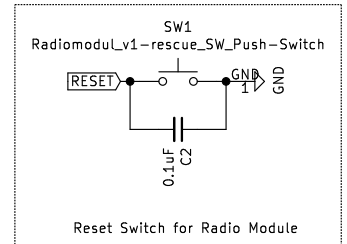
Reset Switch for Radio Module
