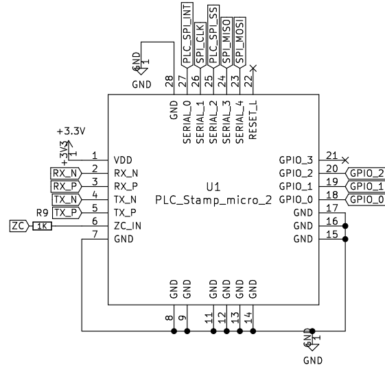
PLC Module with QCA7000
