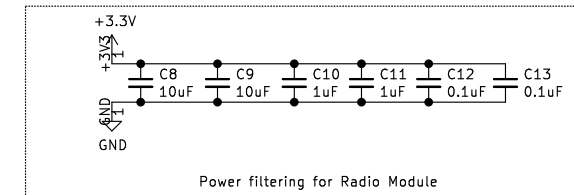
Power filtering for Radio Module
