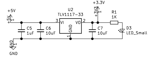
5V to 3.3V LDO
