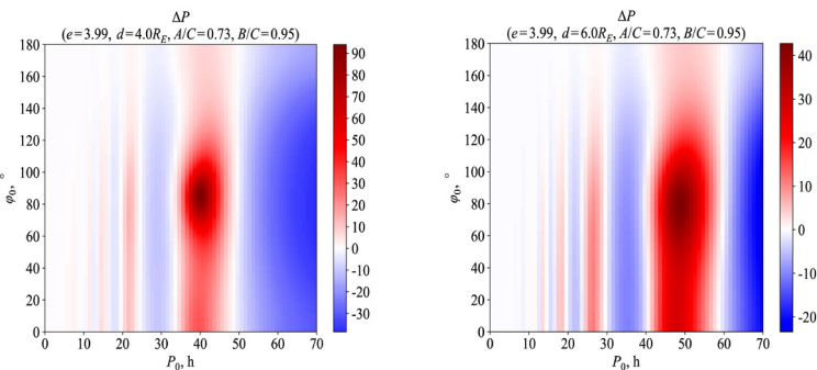
Fig. 2. The dependencies of the value \Delta P (in hours) of the change in the rotational period of the asteroid due to its close encounter with Earth on the initial values of the rotational period P_0 and the angle \varphi_0 between the rotational axis and the orbital plane for different values of the pericentric distance d . A/C and B/C are ratios of the main central moments of inertia of Apophis [7].
