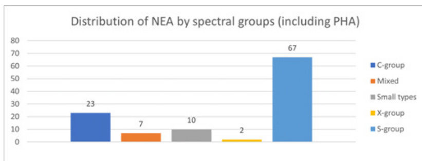
Fig. 2. Distribution of NEA by spectral groups (including PHA)
