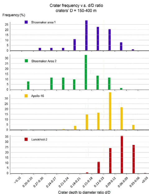
Fig. 1. Histograms of the relative depth ( d/D ) values for craters of the Shoemaker floor Areas 1 and 2 and the Apollo-16 and Lunokhod-2 sites
