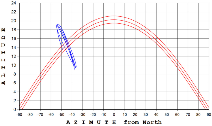
Fig. 4. The apparent motion graph of Sun and Earth across the lunar sky in the period October – December 2021 for the main landing site
