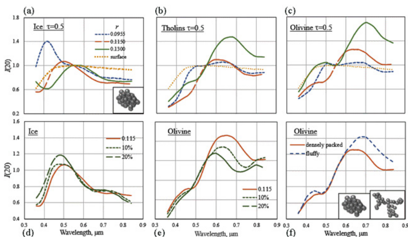
Fig. 2. Model RS of a conditional primitive asteroid (having a mean surface spectral characteristics with geometric albedo of 0.07 at 0.56 \mu\text{m} and a typical phase angle of 20°) enveloped by a thin DE (at optical thickness of 0.5) composed of aggregate particles with submicron constituents (their sizes are given in the right upper or bottom corners of the pictures) and different composition (water ice, tholins, and olivine) [4–5]
