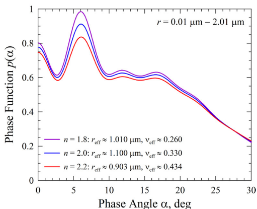
Fig. 1. Phase function p(\alpha) of poly disperse particle systems of the sulfuric-acid sphere simulated at \lambda = 0.365 \mu\text{m} using the Mie theory
