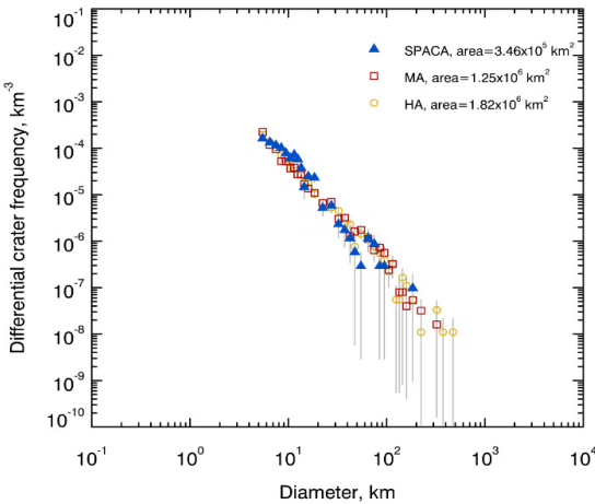
Fig. 2. CSFD analysis for craters with diameters over 5 km in the three SPA interior compositional zones
