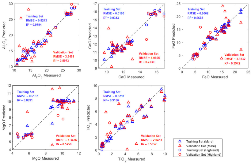
Fig. 2. Scatter plots of five major oxides
