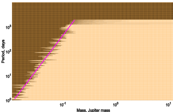
Fig. 1. An example of a single detectability window with the boundary between “detectable” and “undetectable” planets
