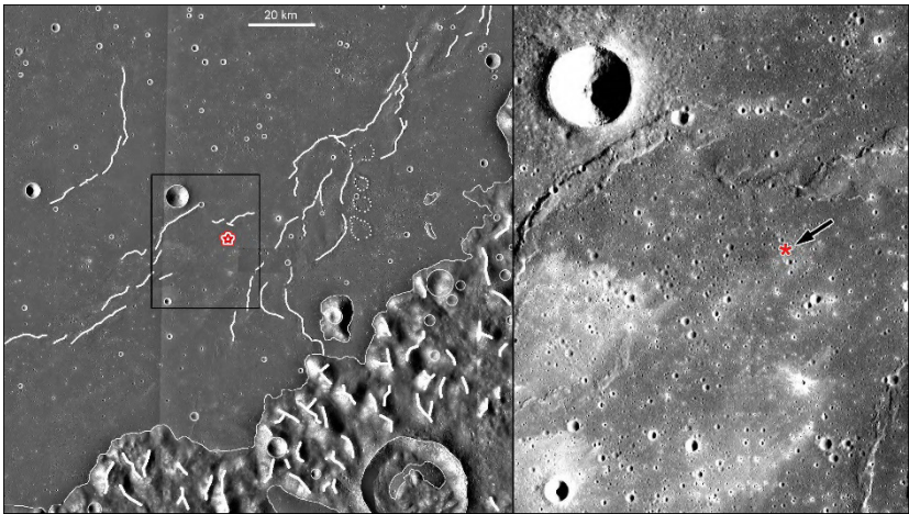
Fig. 2. The vicinity of the Luna-24 site seen on the LROC WAC mosaic. The black box outlines the area shown on the right (left). : Portions of the Kaguya Terrain Camera mosaics, morning version. Crater Fahrenheit (6 km diameter) is in the upper left. Red stars show the landing site (right)
