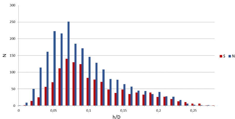
Fig. 1. Graphs of the dependence of the number of craters on the ratio of h/D in the northern and southern polar regions of the Moon
