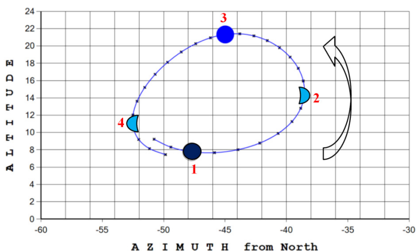
Fig. 1. The apparent motion graph of Earth across the lunar sky in July 2023 in the topocentric horizontal coordinate system for the main landing site. Black crosses indicate the position of the Earth’s disk with an interval of one day. The red numbers indicate the degree of illumination: 1 — “new Earth” on July 3; 2 — the first quarter on July 10; 3 — “full Earth” on July 18; 4 — the last quarter on July 26. The arrow shows the direction of movement. The coordinates are signed in degrees
