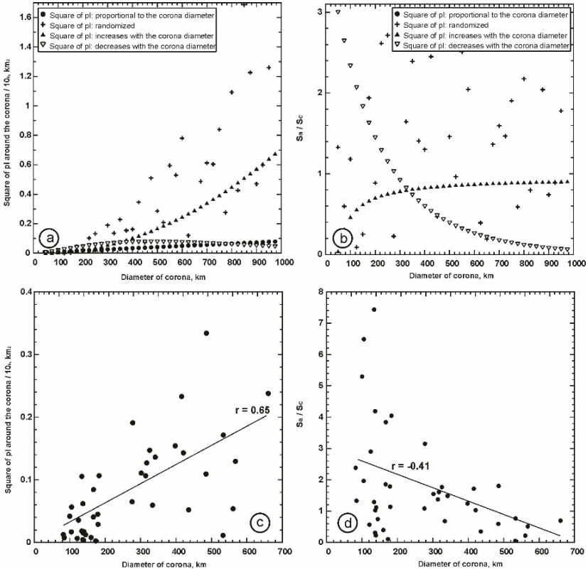
Fig. 1. Models of possible relationships between the corona areas and areas of lobate plains sourced by coronae
