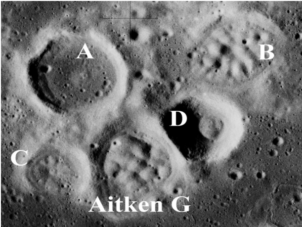
Fig. 1. General view of the Aitken crater floor in the area of the “bulbous fields”. The conditional unofficial names of the four craters, which are used within the text of these theses, are indicated in capital letters. Aitken G crater is the generally accepted official name on lunar maps
