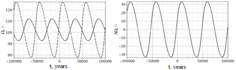
Fig. 1. Dependence of the change in the longitude of the ascending node for Jupiter (solid line) and Saturn (dashes), representing the secular precession of the orbital planes of the giant planets under the action of mutual perturbation ( left ); the difference in the longitudes of the nodes of Jupiter and Saturn’s orbit as a function of time ( right )
