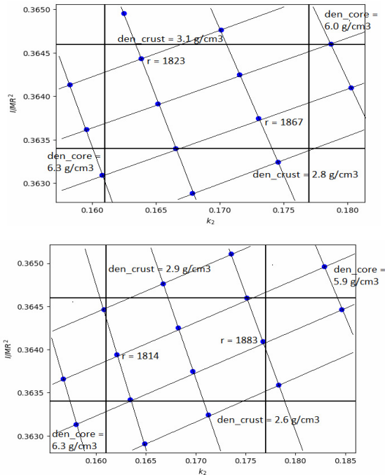
Fig. 1. The selection of the models: the horizontal solid lines indicate admissible values of the moment of inertia, the vertical solid lines — of Love number k_2 . \text{Fe\#} = 0.18 on the top, \text{Fe\#} = 0.20 on the bottom
