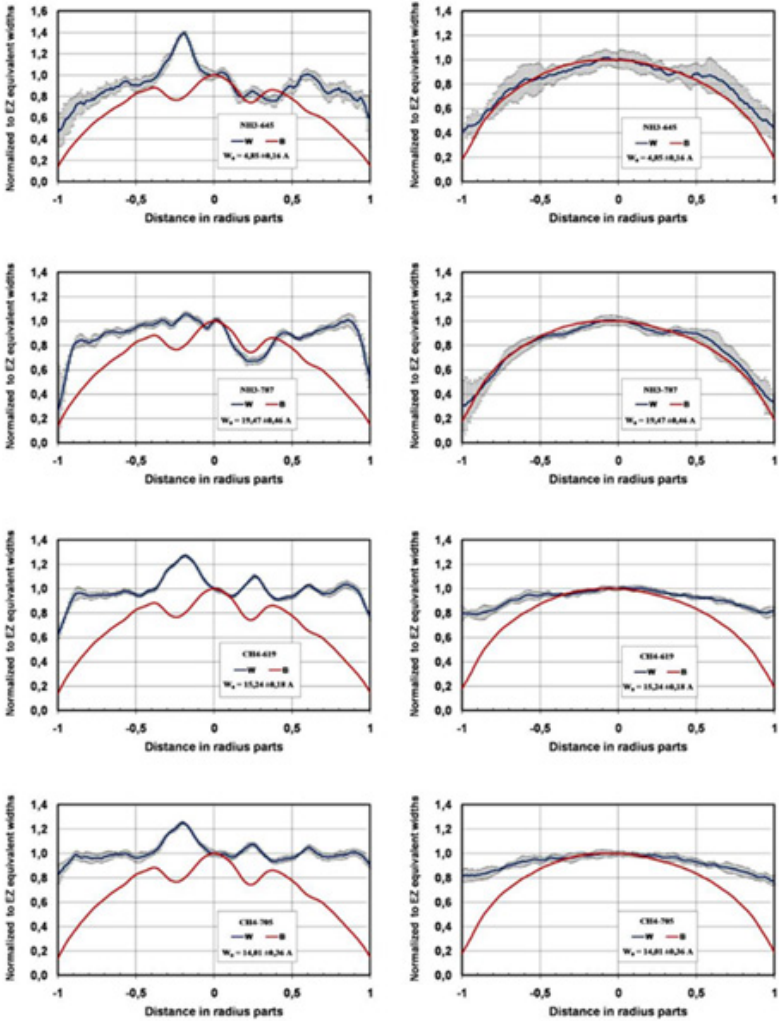
Fig. 1. Comparison of relative intensities of CH 4 and NH 3 absorption bands and brightness profiles observed in the continuous spectrum along Jupiter's central meridian and equator.
