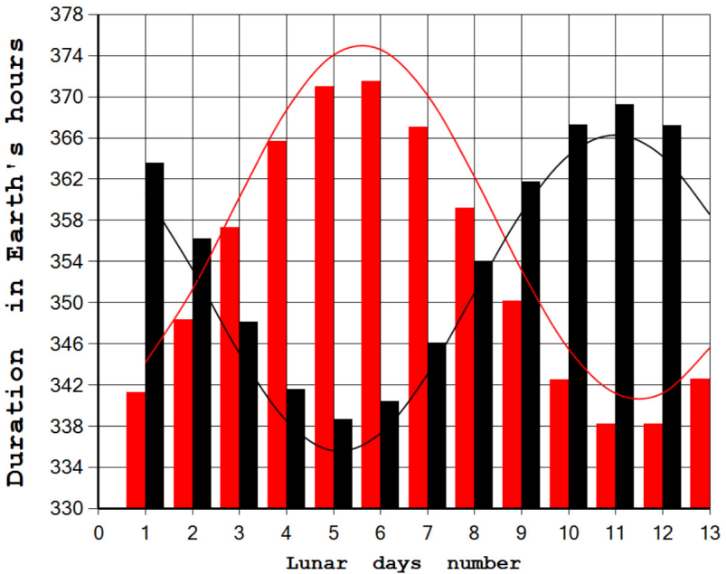
Fig. 5. The duration of the lunar day and night in hours for the main landing site is from August 2023 to August 2024. Red is day, black is night
