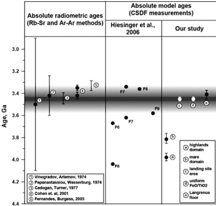
Fig. 2. Comparison of the radiometric ages of particles in the Luna-16 sample and collection of the results of the AMA determinations in different parts of Mare Fecunditatis
