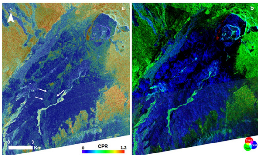
Fig. 1. Kilauea region shown here in a) circular polarization Ratio (CPR) and b) NNED images. These polarimetric products are generated from RISAT-1A C-band SAR data at a resolution of 7 m/pixel. The CPR image is stretched to a colour scale and overlaid on HV-pol data and the colour wheel in the decomposition image (b) highlights the colours for each scattering regime (red: even bounce; blue: single (odd) bounce; green: volume/diffuse scattering). Notice the December 1974 pāhoehoe flows (indicated with arrows in (a)) that have a CPR contrast with the background and are not readily visible from other polarization images
