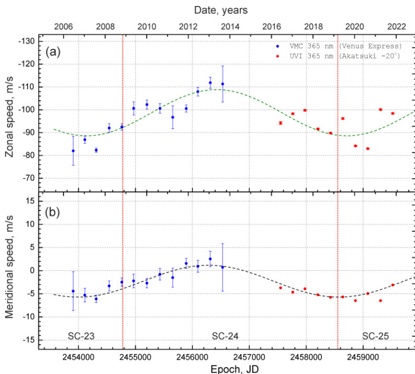
Fig. 1. Long-term variations of the mean zonal (a) and meridional (b) wind speed at 20 \pm 2.5^\circ S at around noon ( 12 \pm 1 h LT) derived from VMC/ Venus Express (blue) and UVI/ Akatsuki (red) images. Error bars correspond to 99.6 % confidence interval ( 3\sigma_{\bar{x}} ). The zonal wind component is negative, indicating east-west retrograde circulation. The negative sign of the meridional speed corresponds to north-south motions.
