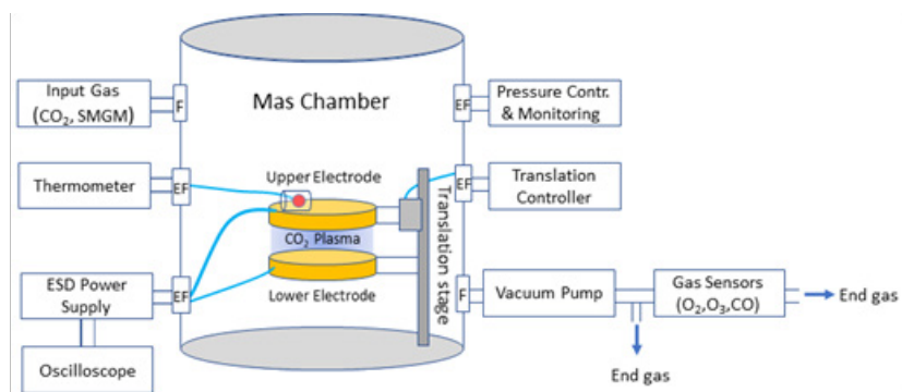
Fig. 1. Experiment setup of ESD CO 2 glow discharge for the study of chemical reaction under simulated Martian conditions (F: Flange; EF: Electrical feedthrough; SMGM: Simulated Martian Gas Mixture)
