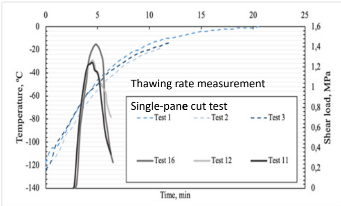
Fig. 2. Graph of thawing samples with 10 % water content and test results of 3 samples at a normal load of 0.1 MPa
