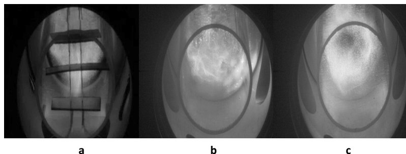
Fig.2. Video frames (exposition \sim 1 \mu\text{s} ) from the high-speed camera Phantom VEO 710L obtained \sim 20 \text{ ms} after the microwave pulse: a — Tsarev meteorite; b — LMS-1D regolith simulant with 10 % Mg; c — ilmenite.
