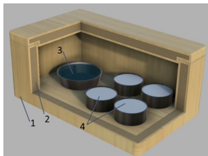
Fig. 1. Scheme of preparing samples for testing: 1 — hardboard box, 2 — heat insulator, 3 — liquid nitrogen, 4 — samples in metal rings
