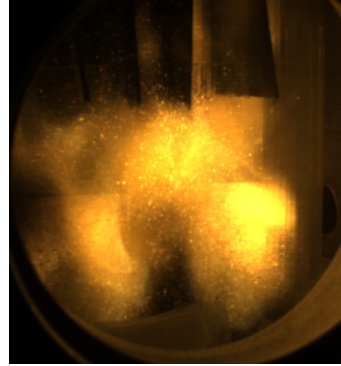
Fig. 3. View of particle cloud in plasma chemical reactor
