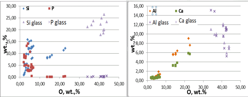
Fig. 2. Contents of various elements in iron submicrospherules with respect to oxygen, for a basalt glass target. Purple markers are responsible for the content of these elements in the glass, which is the matrix for these nanospheres
