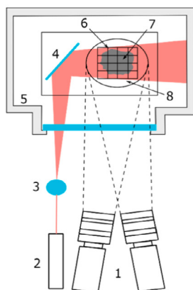
Fig. 1. Picture and scheme (top) of the experimental setup for investigating the dust particles trajectories: 1 — CMOS cameras, 2 — laser, 3 — beam expander, 4 — mirror, 5 — vacuum chamber, 6 — steel mesh, 7 — dust particles, 8 — conductive substrate
