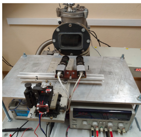
Fig. 1. Picture and scheme (top) of the experimental setup for investigating the dust particles trajectories: 1 — CMOS cameras, 2 — laser, 3 — beam expander, 4 — mirror, 5 — vacuum chamber, 6 — steel mesh, 7 — dust particles, 8 — conductive substrate
