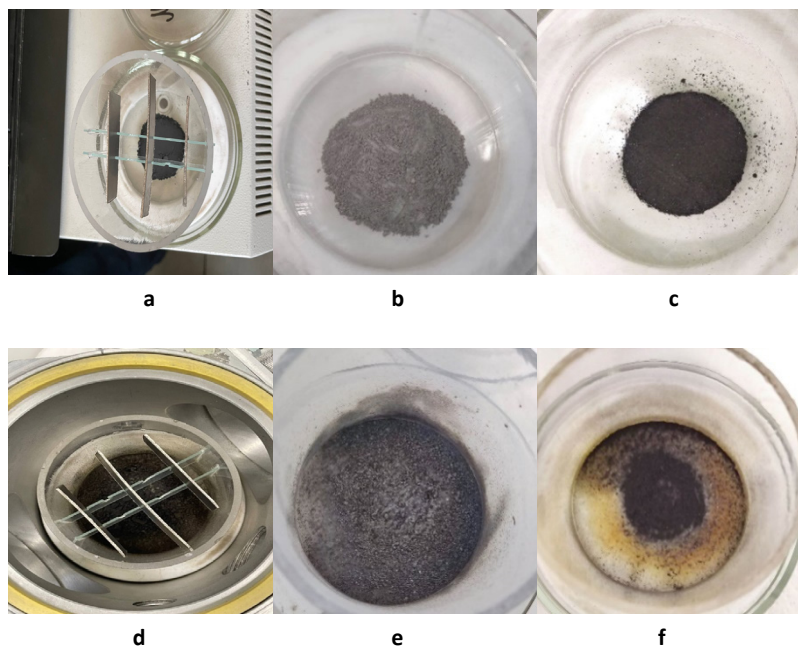
Fig. 1. The samples before (a–c) and after (d–f) the experiments: a, d — Tsarev meteorite; b e — LMS-1D regolith simulant with 10 % Mg; c f — ilmenite
