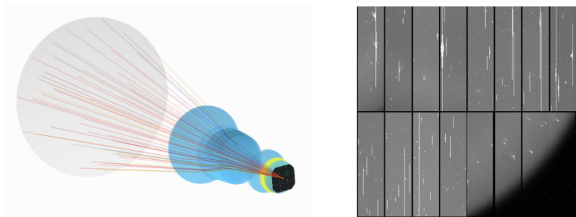
Fig. 1. PHOSIM simulated optical design of WFST ( left ); The simulated 90s exposure time of a CCD from the WFST FOV edge ( right )
