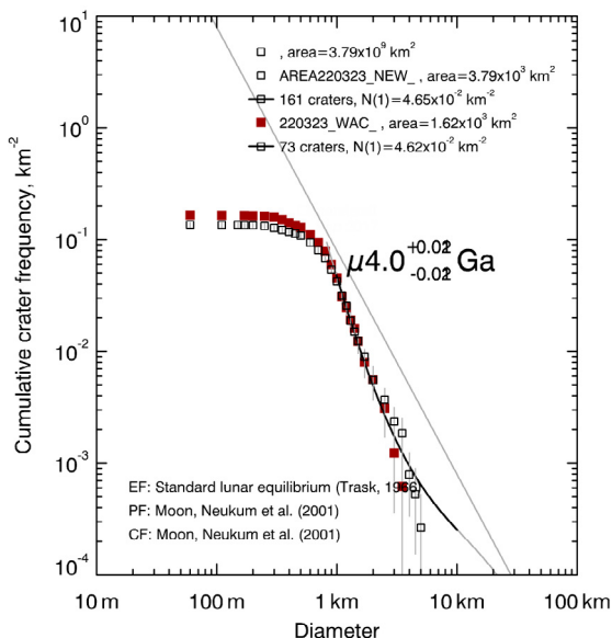
Fig. 2. Size-frequency distribution of superposed primary craters: black-white squares - on the floor of the Plaskett, red squares - on the floor part of the Plaskett on which the LRO WAC mosaic is informative
