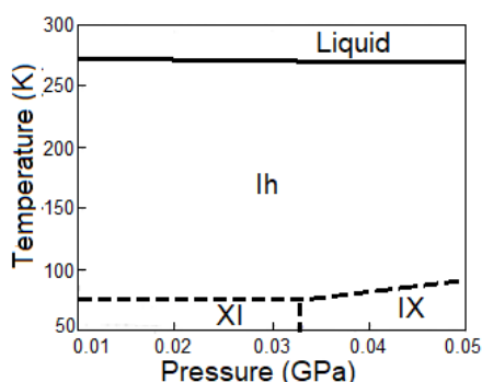
Fig. 1. Low-pressure and the low-temperature part of the phase diagram of ice XI [10]
