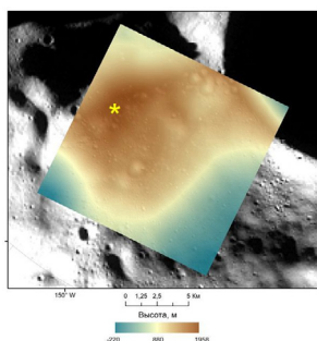
Fig. 3. Digital elevation models of sites #2 by data on LRO spacecraft (NASA) [7]. The asterisk shows the location of the temp. estimate in the lunar soil
