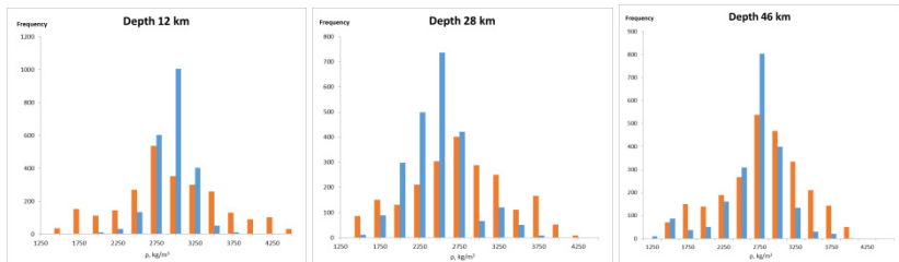
Fig. 2. Histograms of frequencies of values of a priori (orange) and a posteriori (blue) density function for depths of 12, 28 and 46 km
