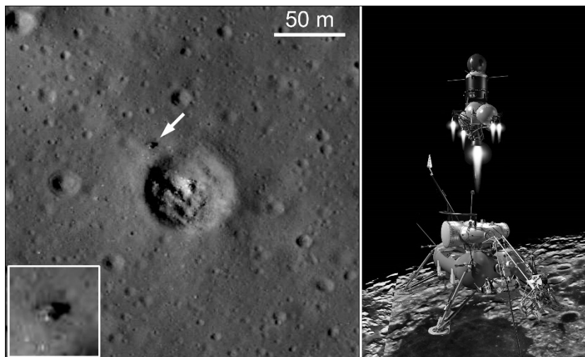
Fig. 1. Surface of Mare Crisium at the Luna-24 site; portion of LROC NAC image M119449091RE. Arrow shows the lander at the rim of crater Lev, see also inlet (left). Artistic representation of the Luna-24 liftoff, rendered from the image provided by http://russianspaceweb.com/luna24.html (right)
