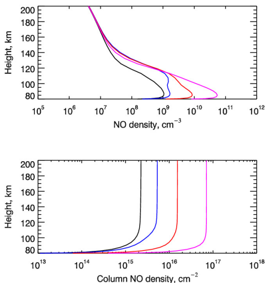
Fig. 1. (top panel) Height profiles of the NO number density calculated in the odd nitrogen chemistry model without (black line) and with taking into account the input of the suprathermal N(4S) atoms through the reaction Nh(4S) + O_2 \rightarrow NO + O . Height profiles of NO number density were calculated for the considered Cases A ( E_0 = 1 keV, blue lines), B ( E_0 = 2 keV, red lines), and C ( E_0 = 5 keV, magenta lines) of the auroral electron precipitation. (bottom panel) Height profiles of NO column densities calculated in the odd nitrogen chemistry model without (black line) and with taking into account the input of the suprathermal N(4S) atoms. The color palette is the same as at the top one.
