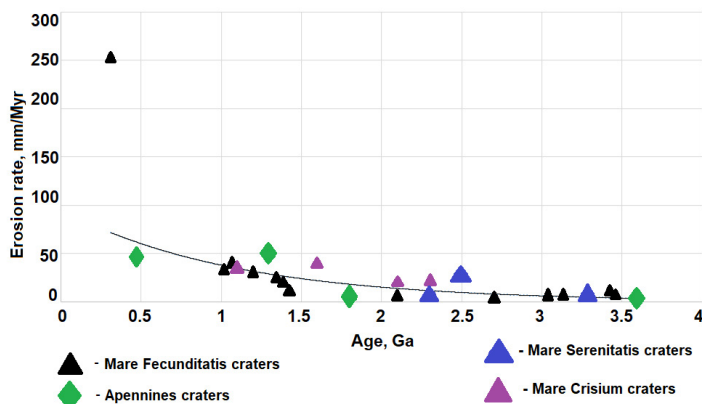
Fig. 3. Erosion rates on craters inner slopes
