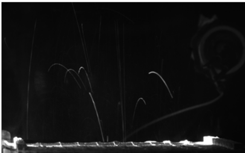
Fig. 2. Visualization of the levitation of Lunar Regolith Analogue particles
