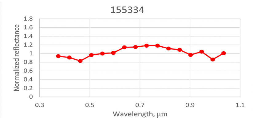
Fig. 1. An example of the final asteroid reflectance spectrum for asteroid 155,334
