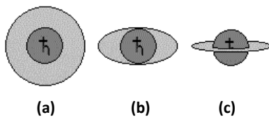
Fig. 2. Evolution of Saturn's protoplanetary cloud into disk-shaped dense rings under the action of the gravitational, centrifugal and magnetic forces: (a) \rightarrow (b) \rightarrow (c)
