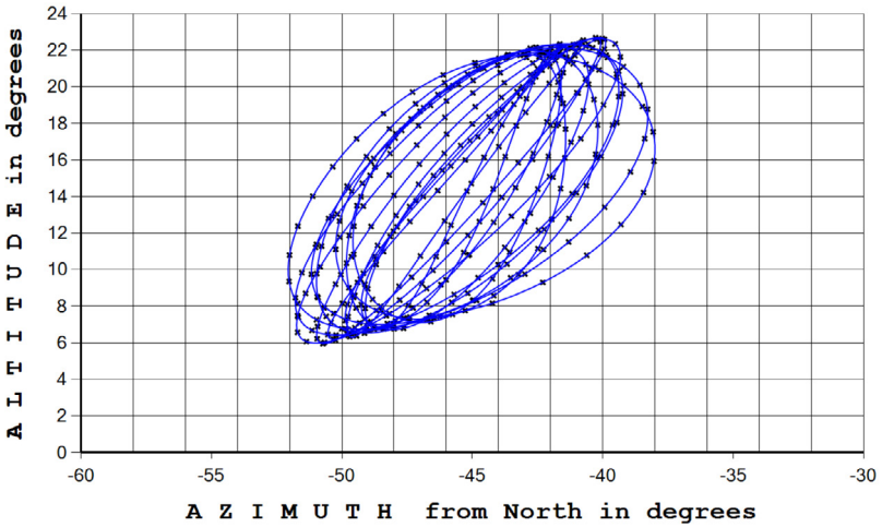
Fig. 2. The apparent motion graph of Earth across the lunar sky during the year (August 2023 – August 2024) at the main landing site
