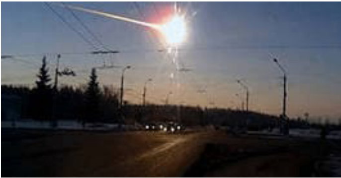
Fig. 1. This is a photograph [5] of the Coulomb explosion [3] that breaks the 2013 Chelyabinsk meteoroid to ions and electrons. This phenomenon is clearly electrical in nature, like the sparking of contacts in a trolleybus or tram, or a cathode spot that “spits out pieces” of the cathode (see [3–4] for more details)
