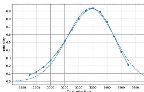
Fig. 5. Probability distribution of Venus' core radius' values. By fitting the highest values to a Gaussian, we get the estimate R_c = 3285 \pm 168 km
