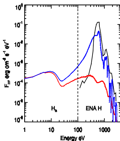
Fig. 1. The calculated energy spectra of the fluxes of suprathermal hydrogen atoms ( 1\text{eV} < E < 100\text{ eV} ) and ENA H ( E > 100\text{ eV} ) at a distance of 8.0R_p from the center of the exoplanet \pi Men c are presented. Blue line represents the downward flux of energy of hydrogen atoms, red one represents the upward flux.
