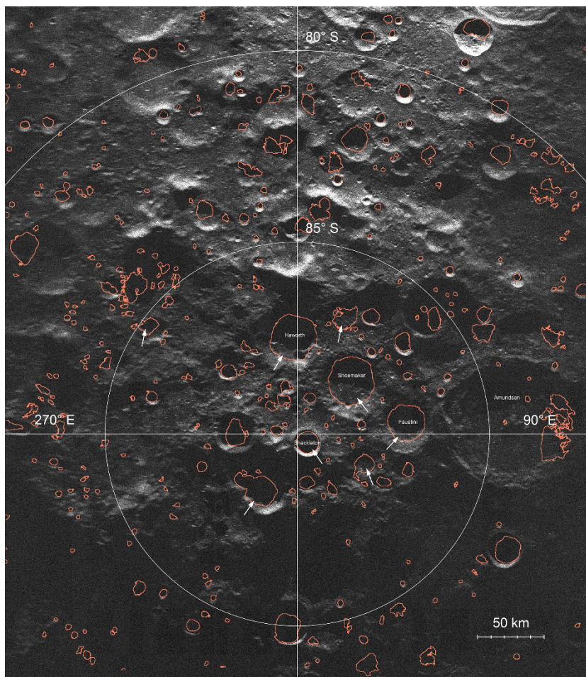
Fig. 1. Opposite-sense circular polarization radar backscatter image of the south polar region of the Moon in orthographic projection. PSRs are circled in red [6], while white arrows indicate several areas visible to the radar
