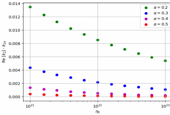
Fig. 2. The increase of Love number k_2 due to anelasticity (in the crust the viscosity is taken \eta_o , in the olivine mantle 10^{-2}\eta_o , in the \beta -layer 10^{-1}\eta_o , in the \gamma -layer \eta_o )
