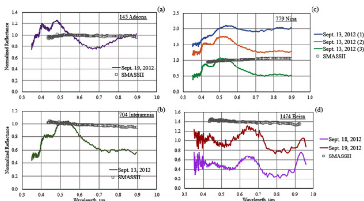
Fig. 1. The RS of four main-belt primitive asteroids, 145 Adeona, 704 Interamnia, 779 Nina, and 1474 Beira, obtained in September 2012, are shown together with their typical ones in standard (calm) conditions from the SMASSII database. We supposed that the detected features may be signs of a thin dust exosphere induced by sublimation of H 2 O ice around the asteroids at a high subsolar temperature near perihelion and in the period of high solar activity (e.g., [3–4]).
