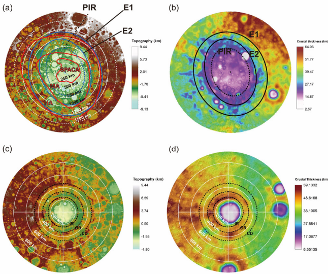
Fig. 1. Topography and Crustal Thickness maps for SPA and Orientale. E1, E2 and PIR in (a) and (b) refer to the two ellipses from [6] and the potential location of SPA inner ring, respectively. The compositional zones in red outlines are from [3]. IR, OR and CD in (c) and (d) refer to the Inner Rook ring, Outer Rook ring and Cordillera ring of the Orientale basin, respectively
