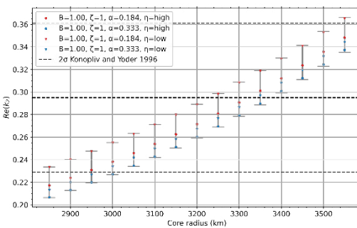
Fig. 3. k_2 values of our Venus' models. Bars represent the variation of k_2 due to the uncertainty in viscosity, \alpha , \zeta and B. Dashed lines represent the measured value 0.295 \pm 0.066 [2]
