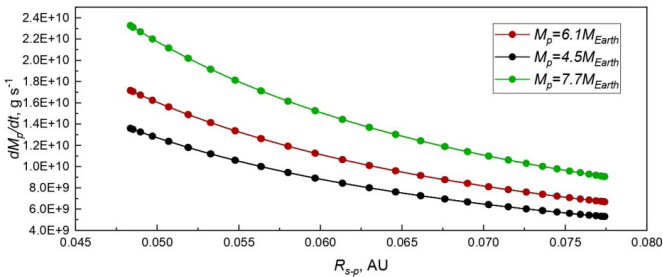
Fig. 1. The dependence of the mass loss rate of the planet's atmosphere on the star-planet distance for sub-neptune HD 207496b assuming different values of the planet's mass [4]
