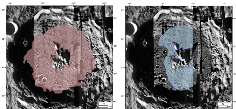
Fig. 1. LROC WAC mosaic partially overlaid with LROC NAC images to interpret craters. On the left, the area of the floor of the Plaskett is bounded in translucent pink, on the right, in translucent blue, the part of the floor is shown, on which the LRO WAC mosaic is informative for CSFD of the floor
