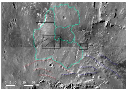
Fig. 1. Morphological units: (1) Peripheral valleyed unit; (2) Northern light unit; (3) Center dark unit; (4) Impact ejection from Holden crater; (5) Eberswalde crater; (6) Bigbee crater; (7) Holden crater. The red and blue dotted lines represent the remnant Bigbee and Holden crater ring, respectively (CTX images)
