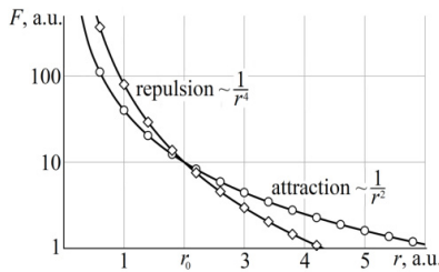
Fig. 3. Dependence of the repulsion and attraction forces on distance between particles
