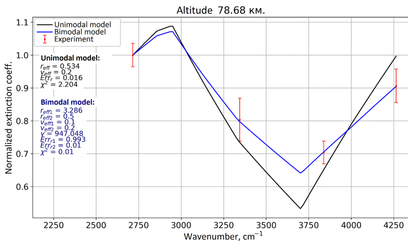
Fig. 1. Normalized extinction coefficient spectrum for unimodal (black), bimodal (blue) models and experiment (red). Observation 2007.08.20. Altitude 78.68 km. Implementation of the second mode allows much more accurate experimental data approximation for this measurement
