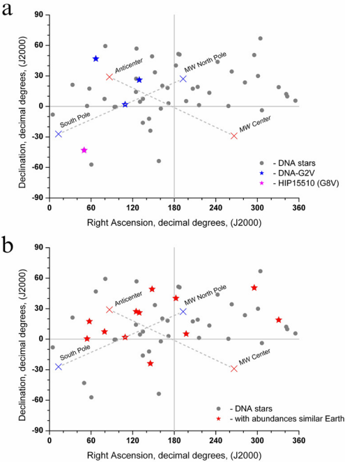
Fig. 1. (a) Three stars belong to the G2V spectral class, as our Sun, were shown by blue and one star, closest to the solar system, which belongs to the other G8V class, were presented by purple color; (b) The T-stars, which have abundances similar to the solar system, were presented by red colors. On both figures as background, the 48 DNA stars, in the spectrum of which C, N, O and P elements were found is drawn by grey color
