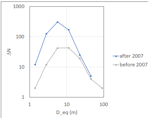
Fig. 1. Differential number DN of “new” impact craters in diameter bins 1 to 2 m, 2 to 4 m, etc. for cataloged ~1800 “new” craters ([2] plus author’s data). The “boundary” year 2007 is chosen to have approximately same number of craters in equivalent diameter bins 16 to 32 m and 32 to 64 m
