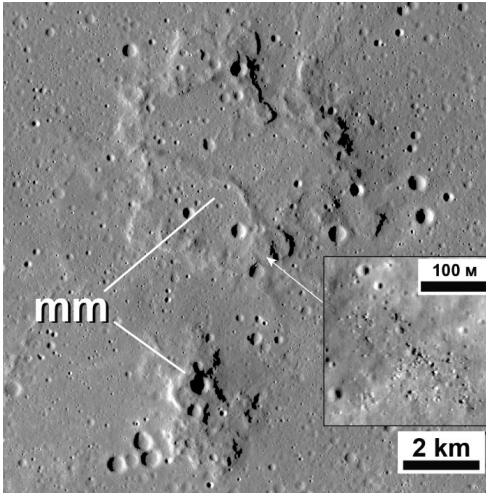
Fig. 3. Western Fecunditatis Mare Mesas. Mosaic of the Kaguya images (inset: LROC NAC image_)
