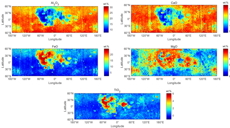
Fig. 3. Maps of five lunar global major oxides by our approach (60° N ~ 60° S).
