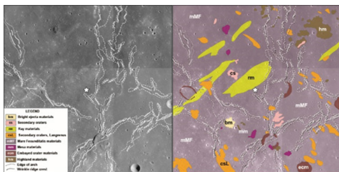
Fig. 1. Geological map of the Luna-16 landing site and its immediate surroundings
