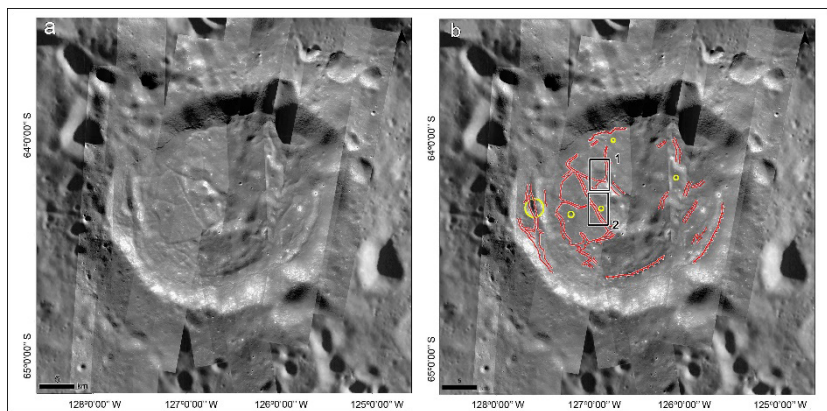
Fig. 1. Mosaic of LROC NAS images showing the considered crater (a); the same with shown on the floor gullies and scarps (red) and prominent craters (yellow) (b). Black rectangles outline areas shown in Fig. 2 and 3.
