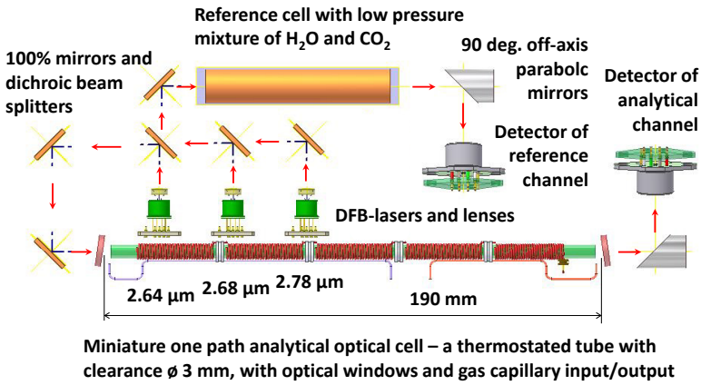
Fig. 1. DLS-L optics layout
