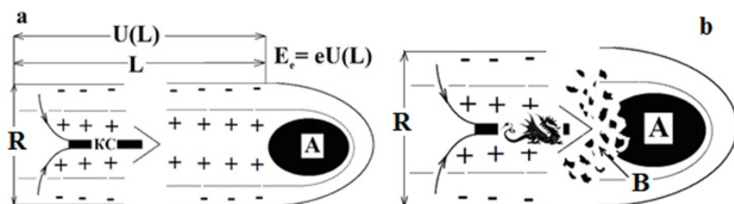
Fig. 2. Two-dimensional scheme: a — a Vysikaylo' railgun with a space charge operating on Coulomb (polarization) forces [3–4], and not on Lorentz forces (as in the Artsimovich railgun). “+” and “–” — represent the separation of the space charge (polarization) of the plasma behind a rapidly moving object — A in the medium. Behind body A, a cumulative jet (CJ) of electrons is formed in a positively charged plasma column, converting the potential energy of polarization (the kinetic energy of the meteoroid) into energy CJ; b — a new cumulative-plasma mechanism of fractal fragmentation of meteoroids, initiated by Coulomb explosions. This mechanism was proposed by the author in [3–4]. A is a fast moving object in an electronegative medium. B — exploding fragments that form a jet engine behind object A and simultaneously destroy it from behind, thereby supplying the engine with a new high-energy “fuel” with an energy of 200 eV per atom of already solid fuel (at a meteoroid speed \sim 20 km/s).
