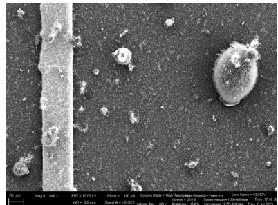
Fig. 5. Micrographs of particles deposited on the surface of the solar panel
