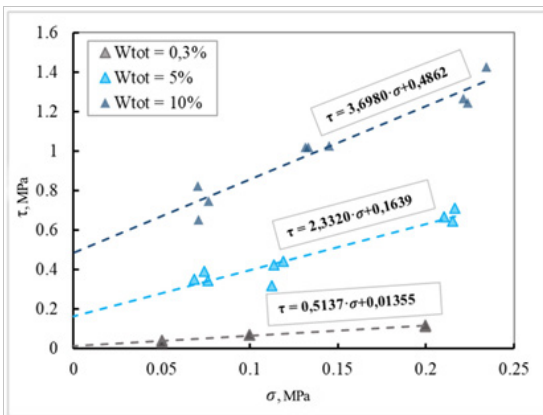
Fig. 3. Test results for samples with a density of 1.75 \text{ g/cm}^3 and various water contents
