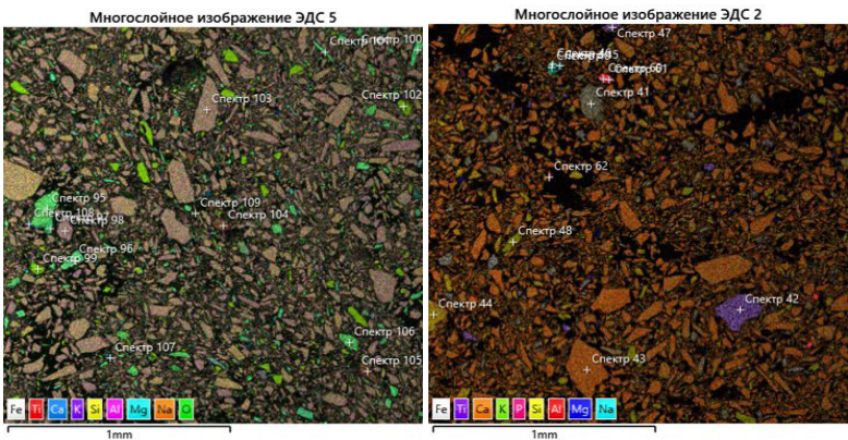
Fig. 1. Scanning electron microscopy results before ( left ) and after ( right ) the experiment. It is noted that such elements as titanium, magnesium, aluminum, and iron are practically not extracted at the current parameters of the experiment
