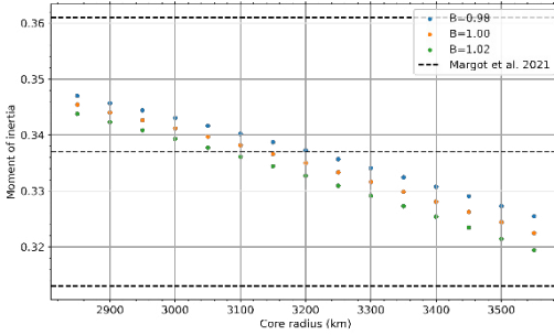
Fig. 2. Moment of inertia values of all 45 models. Dashed lines represent the measured value 0.337 \pm 0.024 [1]
