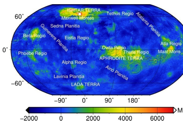
Fig. 1. Topographic map of Venus (in meters). Zero value corresponds to the average radius of the planet. The 60° meridian was chosen as the center of the projection. For clarity, areas with a height of more than 7000 m are marked in white
