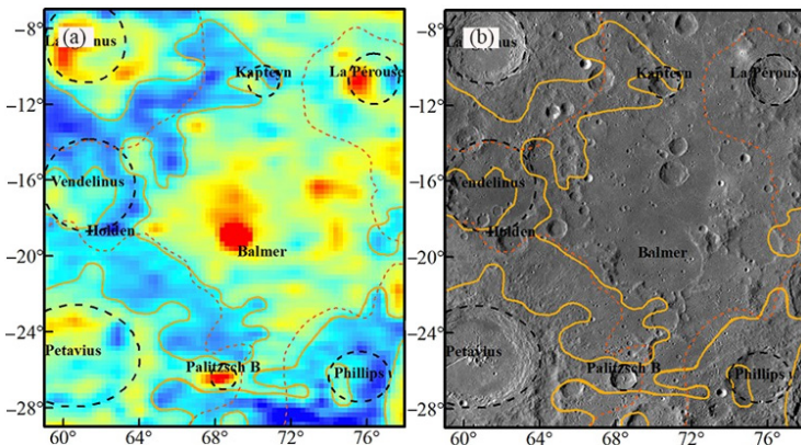
Fig. 2. (a) Low- dT_B anomaly outlined (orange line) in the dT_B map at 37 GHz. (b) Boundary of the low- dT_B anomaly expressed in the WAC image. The dashed lines are boundaries of the impact ejecta identified by B.R. Hawke et al. [2].
