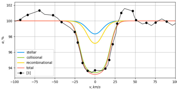
Fig. 1. Comparison of the calculated absorption spectrum with the observational spectrum for exoplanet WASP-12b
