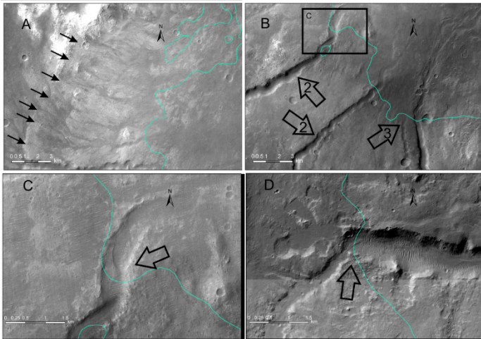
Fig 2. Type of channels: A. channels with funnel-like sources (indicated by black arrows); B. arrows 2 indicate the long and deep V-like channels; arrow 3 indicates the short and shallow channels. C and D. arrow indicate the knickpoint in long and deep V-like channels. The light blue line represents the -280-contour line. (CTX images)
