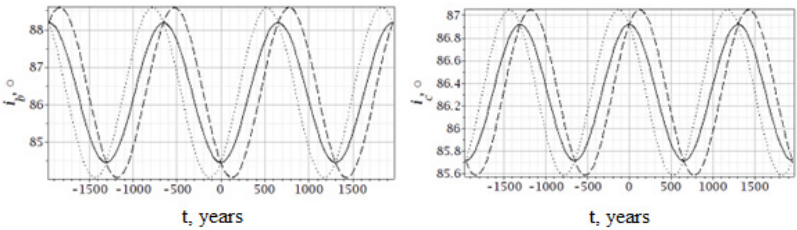
Fig. 3. Time dependence of the orbital inclination for the inner planet K2-36 b (left) and the outer planet K2-36 c (right). The dotted line corresponds to the value \Delta\Omega_0 = -\Delta i_0 , the solid line corresponds to the value and the dashed line corresponds to the value \Delta\Omega_0 = \Delta i_0 .
