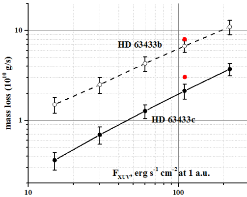
Fig. 1. The integral mass loss of HD 63433b (dashed lines) and HD 63433c (solid lines) as functions of the stellar XUV flux F_{\text{XUV}} . The red dots show data taken from [4]
