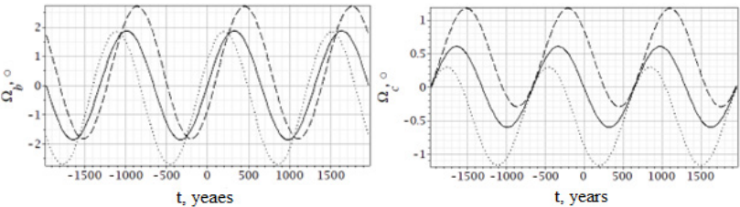
Fig. 4. Longitudes of ascending nodes for planet K2-36 b (left graph) and planet K2-36 c (right) versus time. The dotted line corresponds to the value \Delta\Omega_0 = -\Delta i_0 , the solid line corresponds to the value \Delta\Omega_0 = 0 , and the dashed line corresponds to the value \Delta\Omega_0 = -\Delta i_0 .
