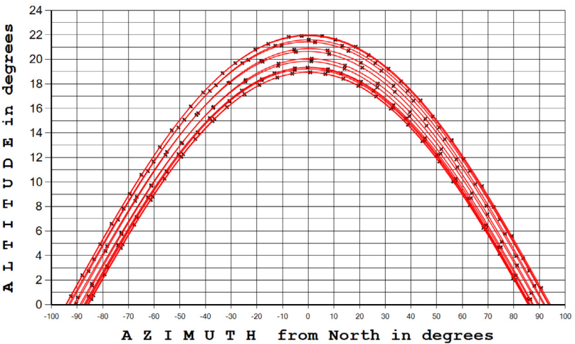
Fig. 3. The apparent motion graph of Sun across the lunar sky during the year (August 2023 – August 2024) at the main landing site
