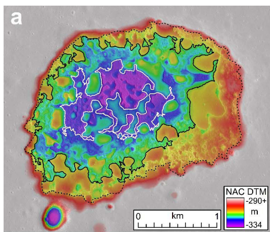
Fig. 3. Topography of Ina interior. LROC NAC DTM on LROC NAC M119815703 [6]
