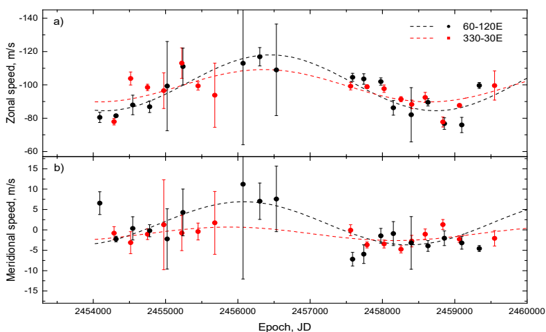
Fig. 1. Long-term variations in the zonal ( a ) and meridional ( b ) components of the mean horizontal flow with a period of 12.5 years at a latitude of 10 \pm 5^\circ S near afternoon ( 12 \pm 1 h) above the highland (black color) — Onda region, 60\text{--}120^\circ\text{E} and lowland (red color) — Navka Planitia and Tinatin Planitia, 330\text{--}30^\circ\text{E} . The dots indicate the mean speed over the Venusian year for a sample of measurements with a phase angle 60\text{--}90^\circ . The error bars correspond to the 99.6 % confidence interval ( 3\sigma_{\bar{x}} ). Dotted lines indicate sinusoids with a period of 12.5 \pm 0.5 years
