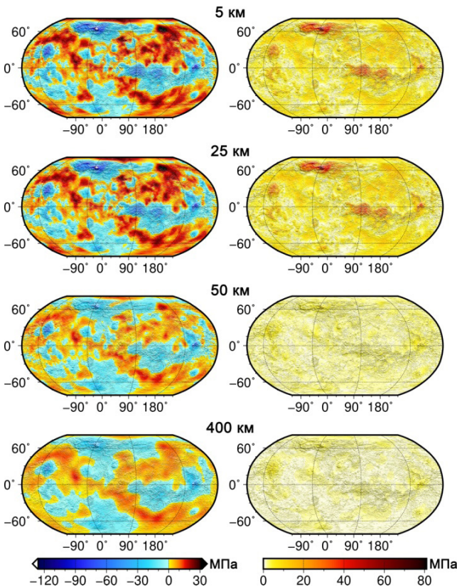
Fig. 2. Extensional-compression stresses (left) and shear stresses (right) (in MPa) in the crust at depths of 5 and 25 km and in the mantle at depths of 50 and 400 km for a model with a lithosphere of 300 km for model V_16 from [9]
