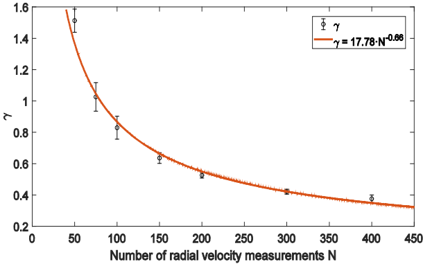
Fig. 2. The dependence of \gamma on the number of radial velocity measurements
