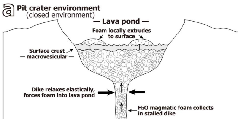
Fig. 2. Conceptual model for pit crater formation [7]
