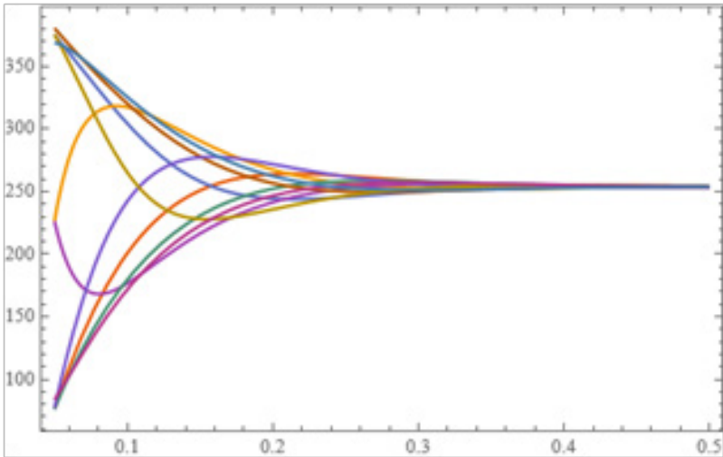
Fig. 2. Model of the daily course of temperature distribution in the lunar soil ( x ) of the equatorial region depending on the temperature on the surface ( y ) with superimposed fluctuations in the region of all possible values
