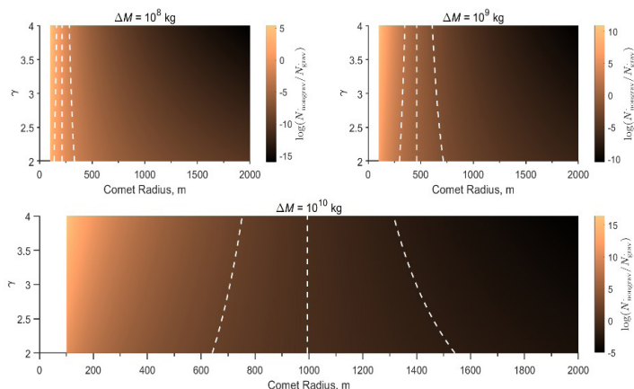
Fig. 1. Comets fluxes from the Oort cloud to the inner part of the Solar system due to gravitational and non-gravitational (cometary outburst) mechanisms. The ratio of fluxes for three masses of ejected material is presented as a function of a comet radius and an exponent in the distribution of comets in the current Oort cloud. The white dotted curves from left to right show the flux ratio 10^2 , 10^0 , 10^{-2} .
