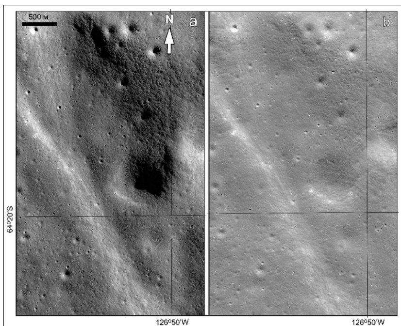
Fig. 3. Fragments of NAC images M1122039053LE/RE (a) and M135960042LE (b) with resolution 0,88 m and height of the Sun above the horizon 14,3 and 24,1°, correspondingly. Conclusion:
