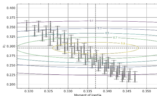
Fig. 4. Probability distribution of all models. Colorful solid lines represent the probability levels of 90, 70, 50, 30 and 10 %, while dashed lines represent the central values k_2 = 0.295 and I = 0.337
