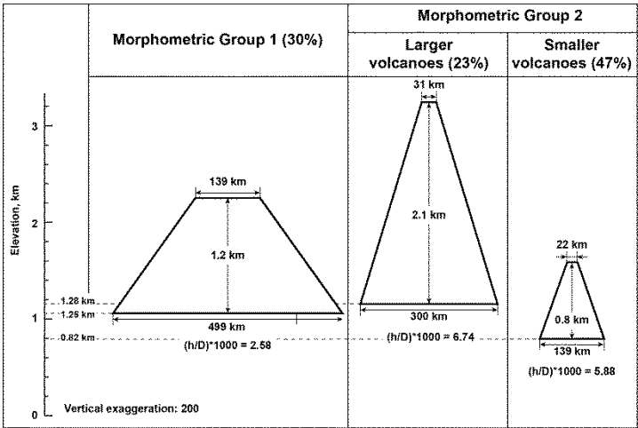
Fig. 2. Generalized shape of different morphological and topographical groups of large volcanoes
