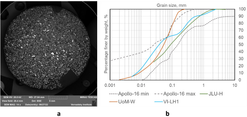
Fig. 1. Image of crushed sample using SEM (a); Cumulative curves of particle size distribution for continental lunar regolith (Apollo-16 [13]) and lunar soil analogues (b)
