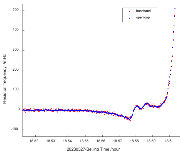
Fig. 1. The orbit determination residual error of the open-loop velocity measurement result during radio occultation procedure
