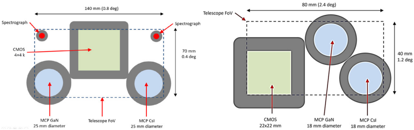
Fig. 2. Focal plane layouts for: 60–100 cm multipurpose telescope ( left ), 15–30 cm multiband imaging telescope ( right )
