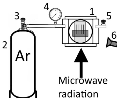
Fig. 1. Plasma chemical complex: 1 — plasma chemical reactor with regolith and solar panels inside, 2 — compressed argon, 3 — gas input valve, 4 — manometer, 5 — gas output valve, 6 — high speed camera
