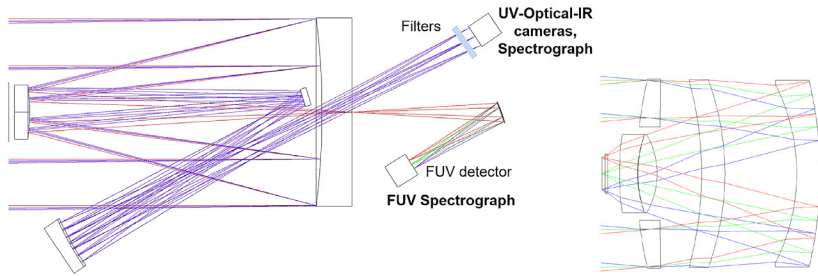
Fig. 1. 60–100 cm telescope for ILRS-5 with two independent focal planes ( left ), extra wide-field 16 cm UV telescope ( right )
