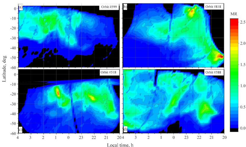
Fig. 1. Examples of O 2 (a 1 Δ g ) airglow emission on Venus nightside in local time — latitude coordinates. Emission intensity is calculated after removing the input of the lower atmosphere and surface, cloud scattering and water vapor absorption: (a) orbit 599 (images 00-07): peak emission is at 1–2 h, most of the bright areas are located on the morning side; (b) orbit 818 (images 00-10): two maxima on the evening side, one of which is near the equator, the other one is in the middle latitudes; (c) orbit 518 (images 00-01): two maxima on both sides of the midnight meridian; the stronger (but also more spatially compact) one is at 1 h, the weaker (but more extended) one is at 22 h; (d) orbit 588 (images 00-06): several local maxima at 22.5, 0 and 3–4 h LT [4].
