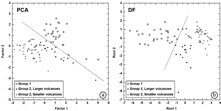
Fig. 1. Results of the principal component (PCA) and discriminant function (DF) analyses of parameters characterizing the gross shape of large volcanoes on Venus
