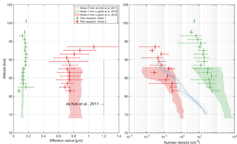
Fig. 1. Comparison of vertical profiles of effective radius ( left panel ) and number density ( right panel ) of mode 1 (green) and mode 2 (red) from this work (crosses), [3] (shaded area) and [5] (blue lines)
