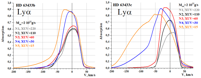
Fig. 2. The calculated Ly \alpha absorption profiles for the transiting HD 63433b (left) and HD 63433c (right) in the Doppler velocity units, obtained in the simulation runs, with different F_{\text{XUV}} ( \text{erg}\cdot\text{cm}^{-2}\cdot\text{s}^{-1} ) values at 1 a.u., under the fiducial SW conditions
