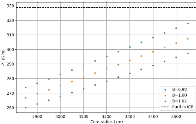
Fig. 1. Pressure at the center of Venus P_c in GPa for all models
