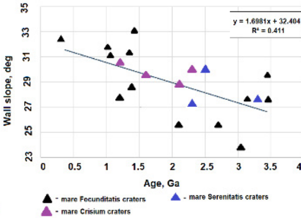
Fig. 1. Correlation between crater AMA and the slope of its walls
