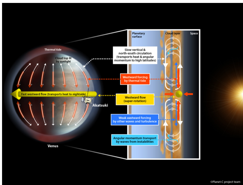
Fig. 1. The schematic of mechanisms how super-rotation of Venus' atmosphere is maintained (a press release illustration for [4])
