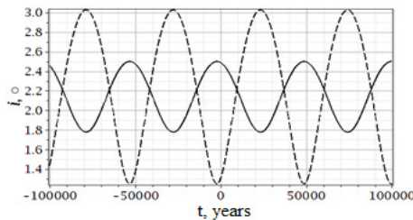
Fig. 2. Time dependence of the inclination (to the ecliptic) of the rings of Jupiter (solid line) and Saturn (dashes)
