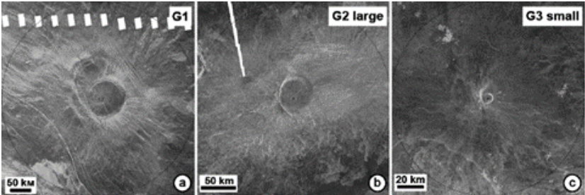
Fig. 3. Typical examples of large volcanoes from the different morphological and topographical groups
