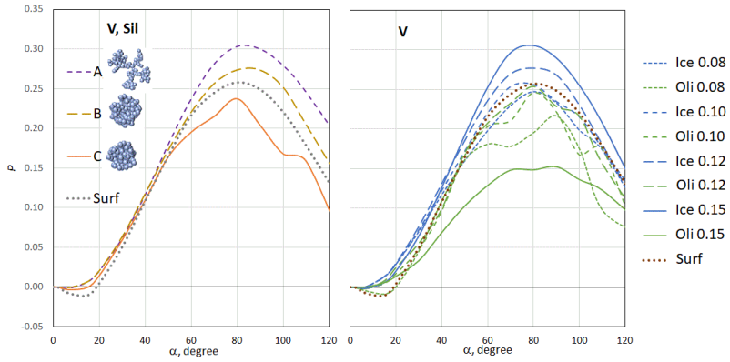
Fig. 2. The linear polarization degree of light P(\alpha) reflected by a model AA with an exosphere composed of aggregates (containing 100 grains). Left: Silicate aggregates are of different porosity, 0.94, 0.72, and 0.54 (for A, B, and C, respectively), and their grains are 0.1 \mu\text{m} in radius. Right: Aggregates of structure C contain ice or olivine grains with radii specified (in microns)
