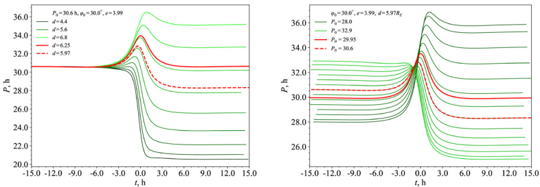
Fig. 1. The change of the rotational period of the asteroid P during its close encounter with Earth, plotted for different values of the pericentric distance d (left) and initial period values P_0 (right). Solid red line corresponds to the value of P_0 for which \Delta P = 0 . Dotted red line corresponds to the value of P_0 for Apophis [8]. The moment t = 0 corresponds to the point of the closest approach to Earth; R_E is the radius of the Earth
