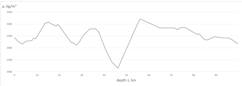
Fig. 1. Averaged density function of the “real” model depending on the depth
