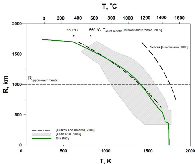
Fig. 1. Estimated current temperature distribution
