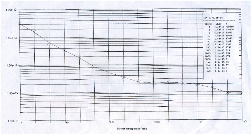
Fig. 2. Frequency stability (Alan variance) of “Bear Like” H2 Maser
