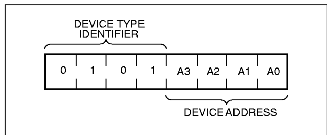
Figure 1. Slave Address
