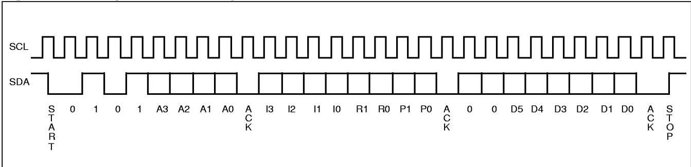
Figure 4. Three-Byte Command Sequence
