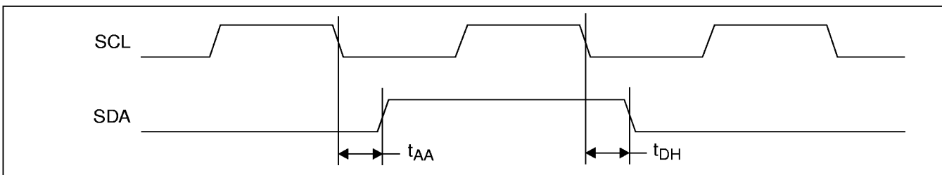
FIGURE 3. Output Timing
