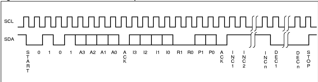
Figure 5. Increment/Decrement Command Sequence
