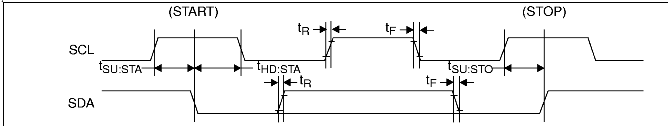
FIGURE 2. Input Timing
