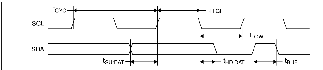
FIGURE 2. Input Timing
