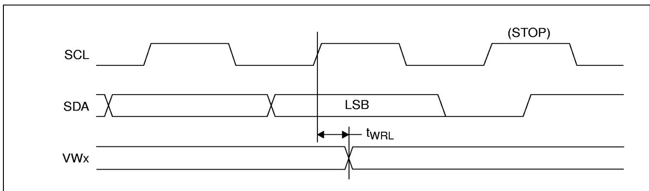
FIGURE 4. EEPROM Timing (for All Load Instructions)
