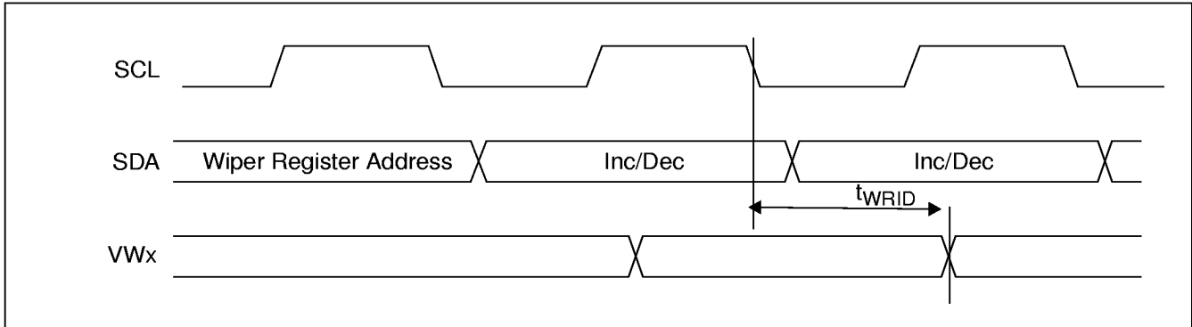
FIGURE 5. EEPROM Timing (for Increment/Decrement Instruction)
