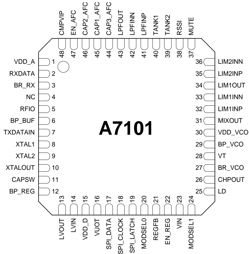
Figure 1. QFN Package Top View
