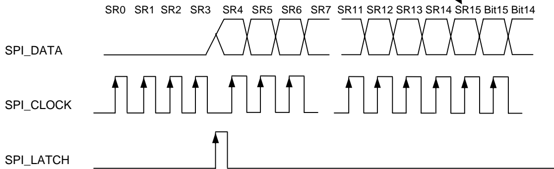
Figure 4. SPI READ mode timing diagram
