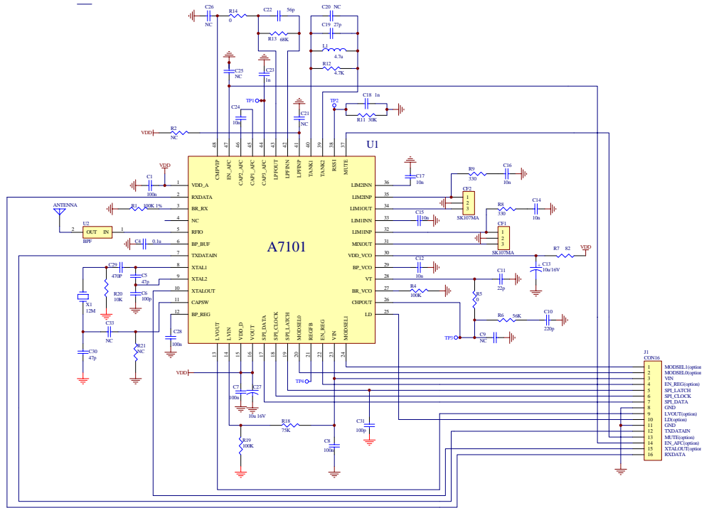
Figure 12. Application Circuit for Receiver
