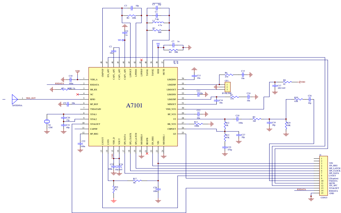
Figure 11. Application Circuit for Transceiver (Data rate = 250Kbps)
