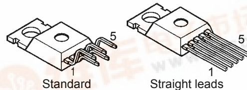
PG-TO220AB/5
