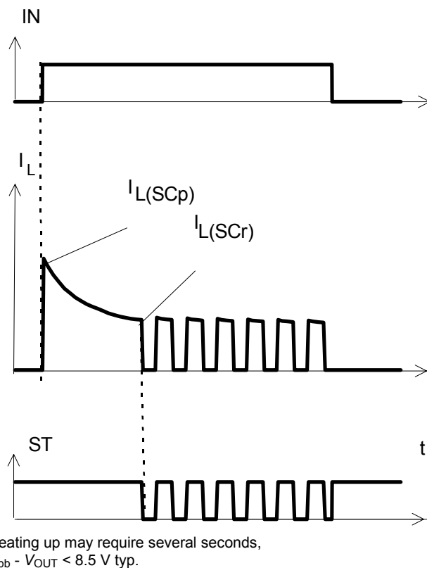
Figure 3b: Turn on into overload,
