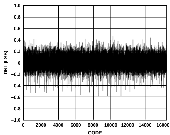
Figure 28. AD9248-65 Typical DNL
