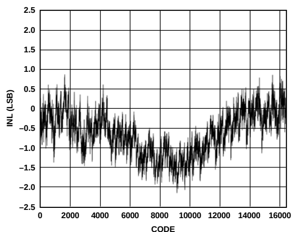
Figure 27. AD9248-65 Typical INL
