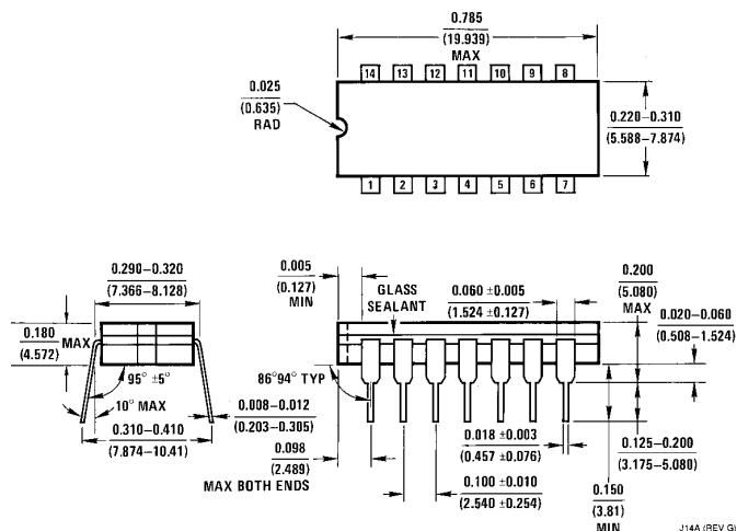
14-Lead Ceramic Dual-In-Line Package (J) Order Number 5402DMQB or DM5402J NS Package Number J14A
