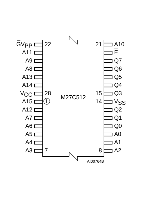
Figure 5. TSOP Connections
