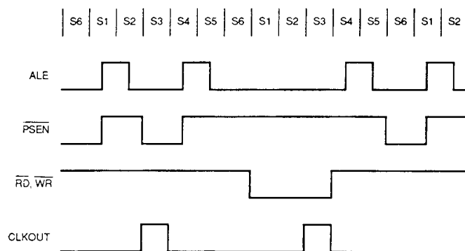
Figure 23. System Clock Timing Overview
