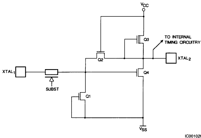
Figure 24. On-Chip Oscillator Circuitry
