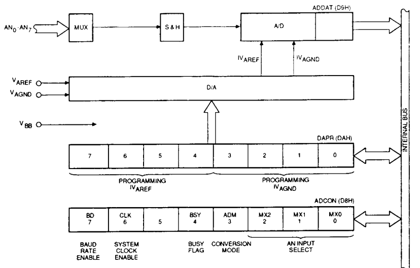
Figure 12. A/D Converter Block Diagram
