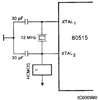
Figure 27. Generating a System Clock from the Oscillator Circuit
