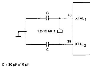
Crystal Oscillator Mode
