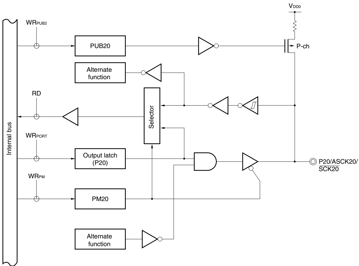
Figure 6-4. Block Diagram of P20
