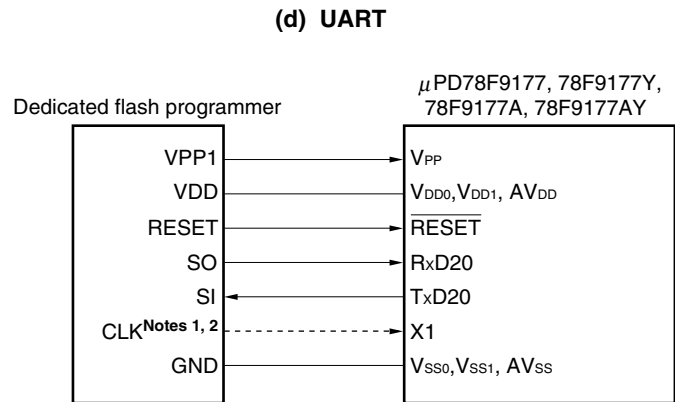
Figure 20-3. Example of Connection with Dedicated Flash Programmer (2/2)
