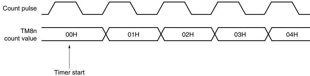
Figure 9-13. Start Timing of 8-Bit Timer Counters 80 to 82
