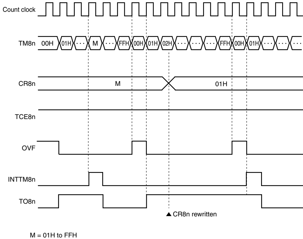
Figure 9-15. Operation Timing After Compare Register Is Rewritten During PWM Output
