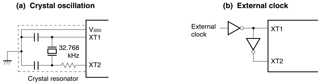
Figure 7-6. External Circuit of Subsystem Clock Oscillator
