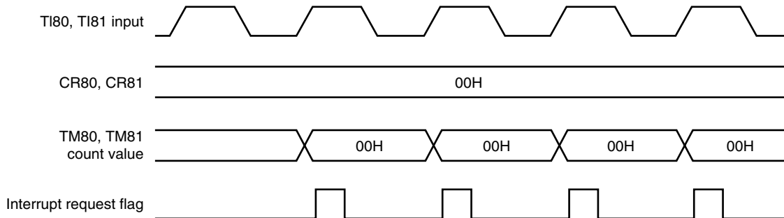
Figure 9-14. External Event Counter Operation Timing
