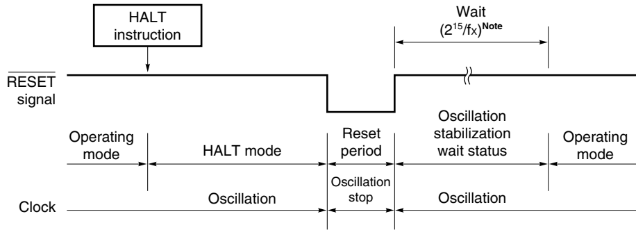
Figure 18-3. Releasing HALT Mode by \overline{\text{RESET}} Input
