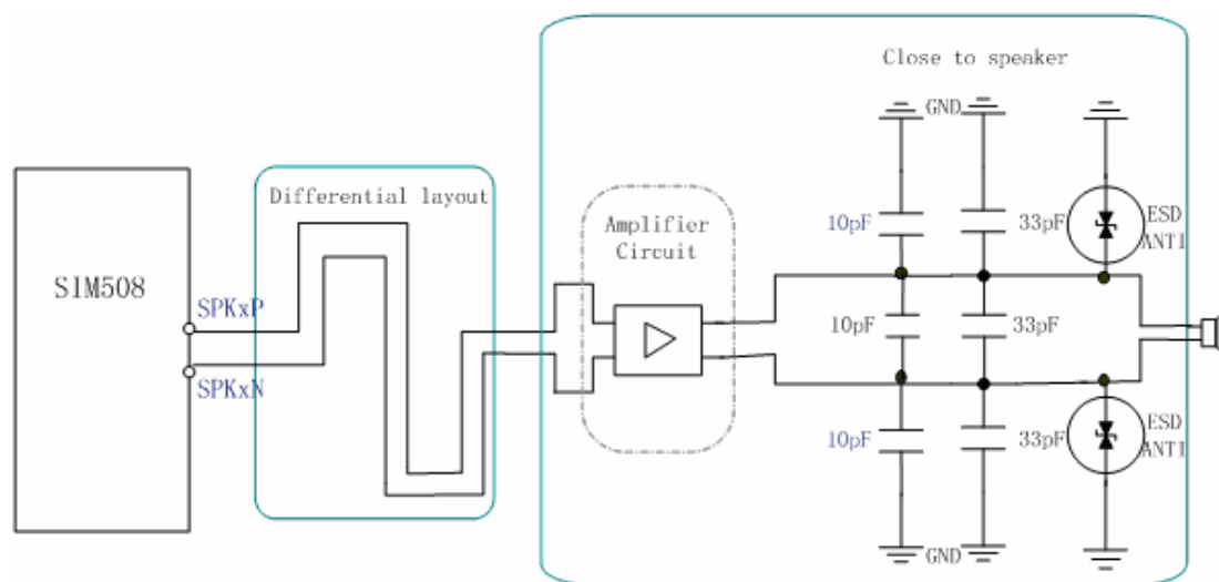
Figure 16: Speaker interface with amplifier configuration
