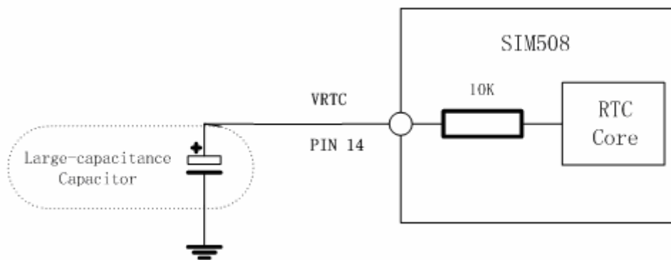
Figure 9: RTC supply from capacitor
