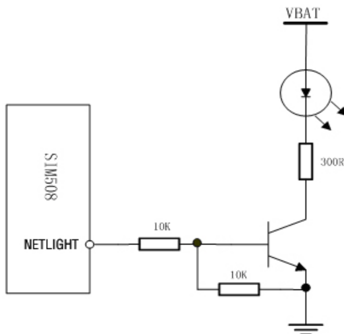
Figure 25: Reference circuit for Network status LED
