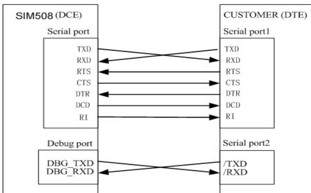
Figure 13: Interface of serial ports
