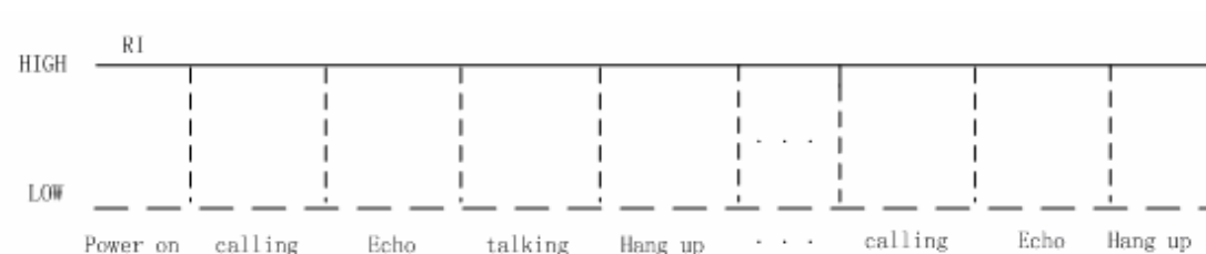
Figure 24: The GSM part of SIM508 Services as caller
