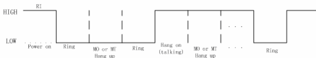
Figure 23: The GSM part of SIM508 Services as Receiver
