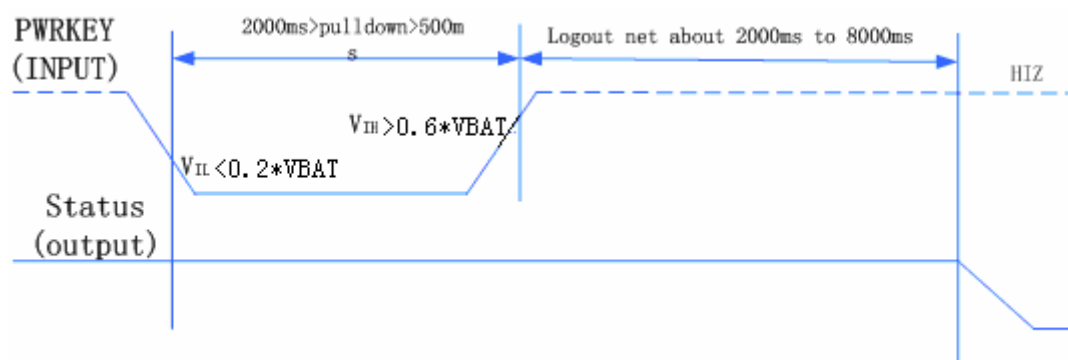
Figure 4: Timing of turn off system
