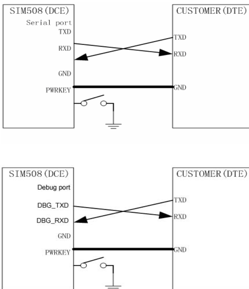
Figure 14: Interface of software upgrade&Debug
