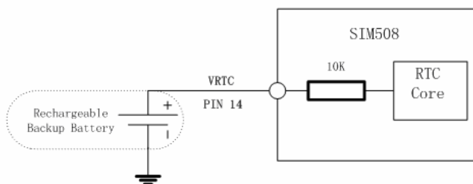
Figure 8: RTC supply from rechargeable battery
