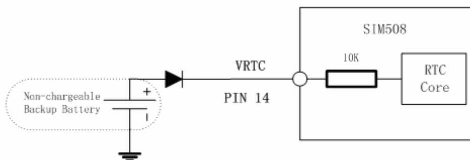
Figure 7: RTC supply from non-chargeable battery
