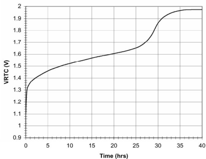
Figure 12: Seiko TS621 Charge Characteristic
