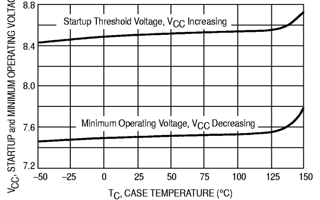
Figure 8. Undervoltage Lockout Thresholds versus Temperature
