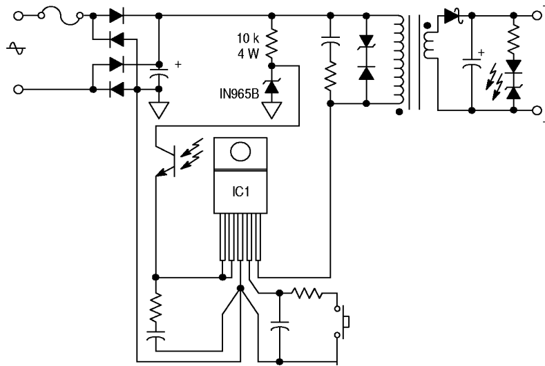
Figure 31. Transformer Auxillary Winding Elimination Zener Shunt Regulator Method
