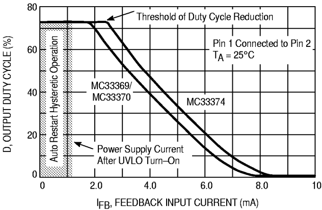
Figure 5. Power Switch Circuit Output Duty Cycle versus Feedback Input Current
