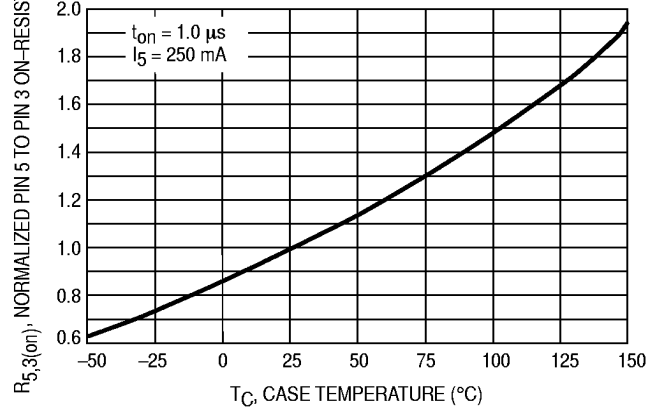
Figure 14. Normalized Power Switch Circuit On-Resistance Pin 5 to Pin 3 versus Temperature
