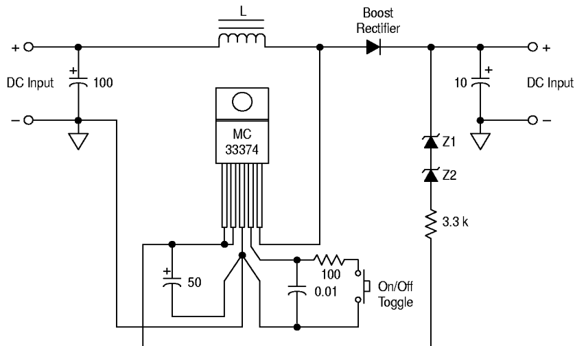
MC33369 thru MC33374 Figure 35. High Voltage Step-Up Converter
