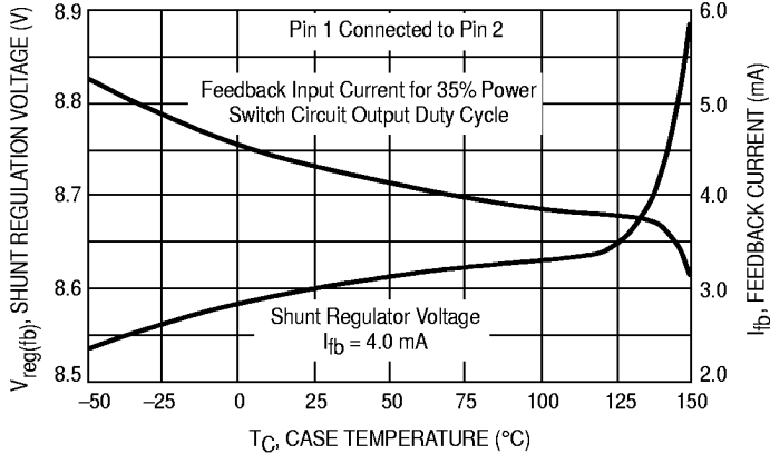
Figure 7. Feedback Input Shunt Regulation Voltage and Current versus Temperature
