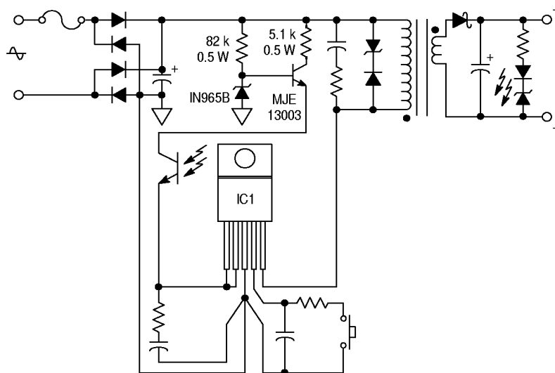
Figure 32. Transformer Auxillary Winding Elimination Bipolar Transistor Series Regulator Method
