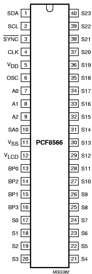
Fig.2 Pin configuration.
