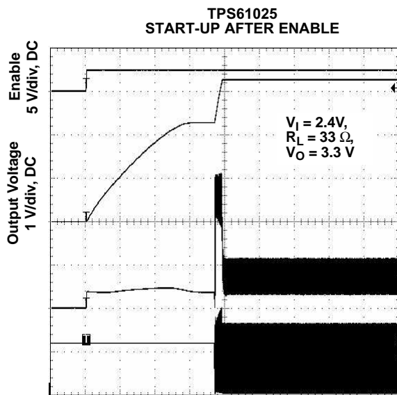
t - Time - 1 ms/div Figure 19.
