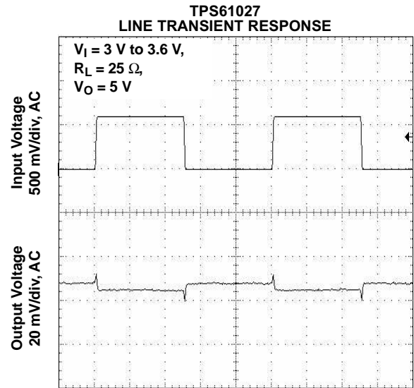
t - Time - 2 ms/div Figure 18.
