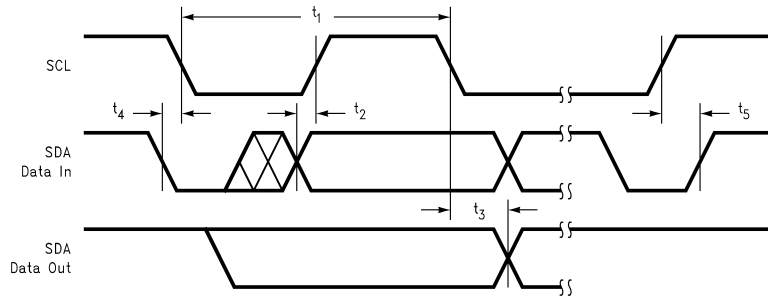
FIGURE 3. Serial Bus Timing Diagram
