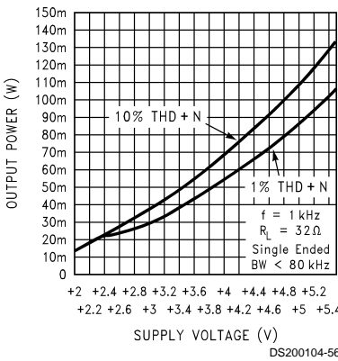
Output Power vs Supply Voltage
