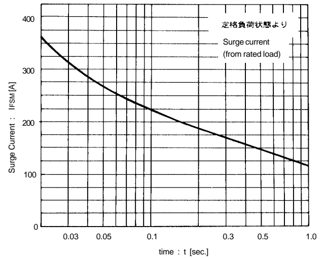
Surge Current
