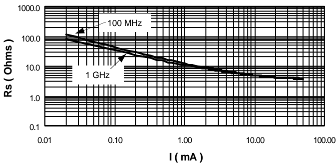
R_S vs. I @ 100 MHz and 1 GHz
