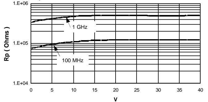
R_P vs. V @ 100 MHz and 1 GHz
