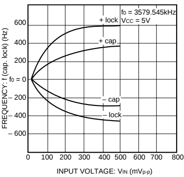
Fig. 13 Capture range and lock range (Ⅱ) vs. input voltage
