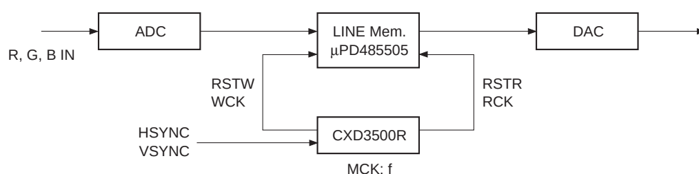
Double-speed display system diagram
