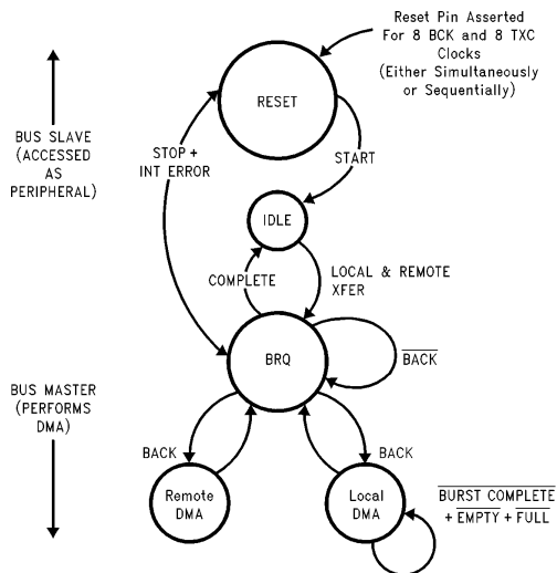
FIGURE 37. DP83907 Core Bus States
