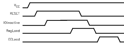
FIGURE 6. RESET Operation
