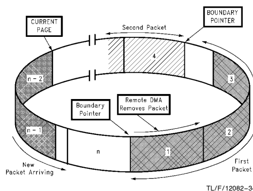
FIGURE 39. 1st Received Packet Removed by Remote DMA
