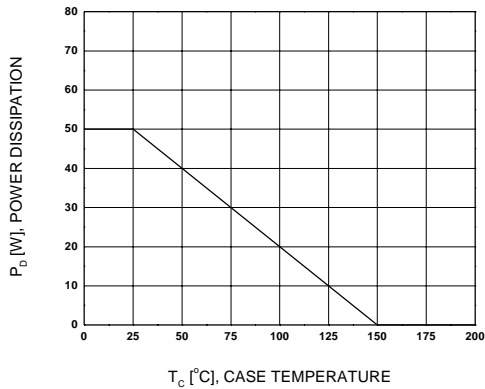
Figure 11. Power Derating
