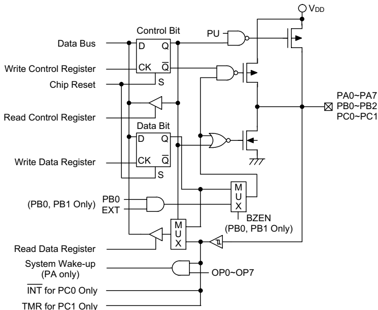
Input/Output Ports
