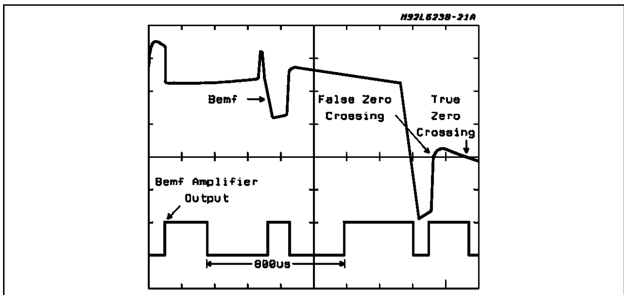
Figure 4-9: Effect of Slow Slew Rate.
