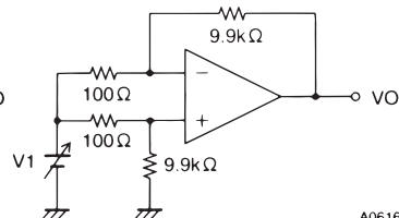
(3) CMRR, V_{ICM}
