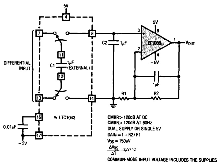
± 5V Precision Instrumentation Amplifier
