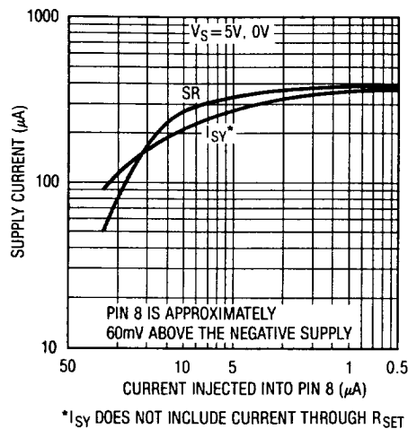
Reducing Power Dissipation
