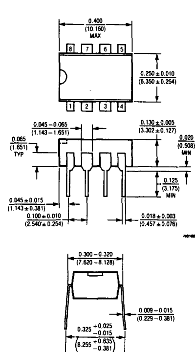
N8 Package Plastic DIP
