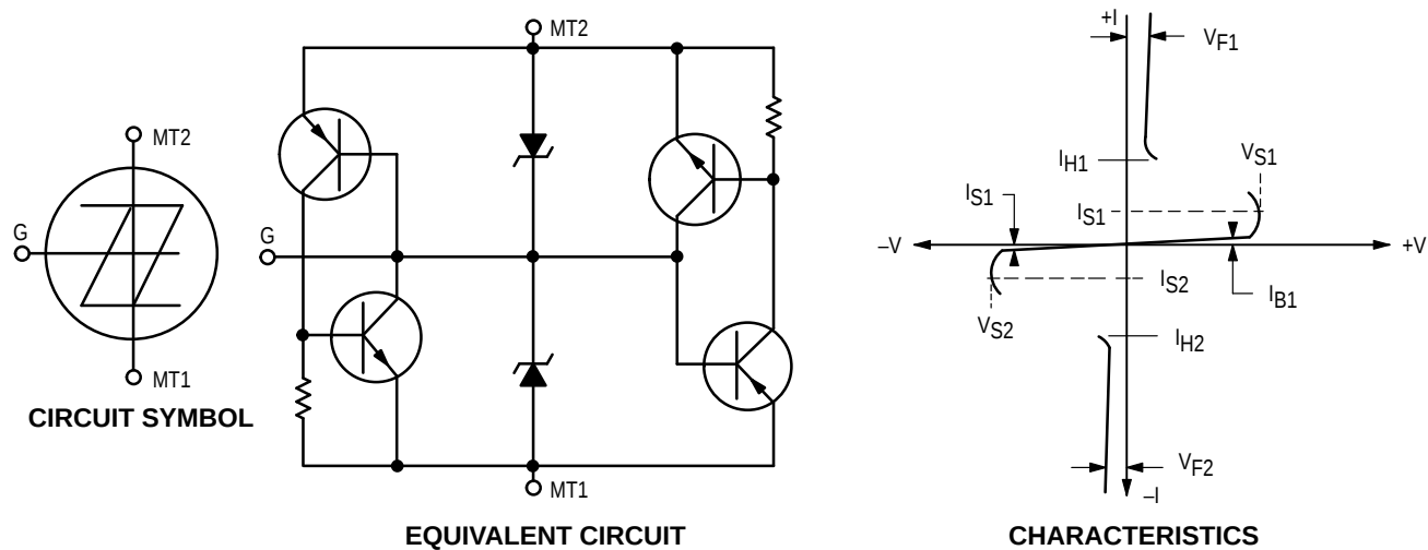
EQUIVALENT CIRCUIT
