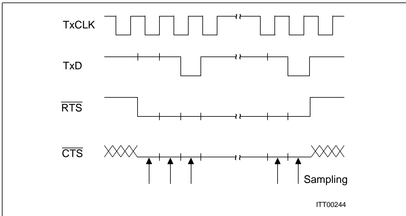
Figure 59 \overline{\text{RTS}}/\overline{\text{CTS}} Handshaking
