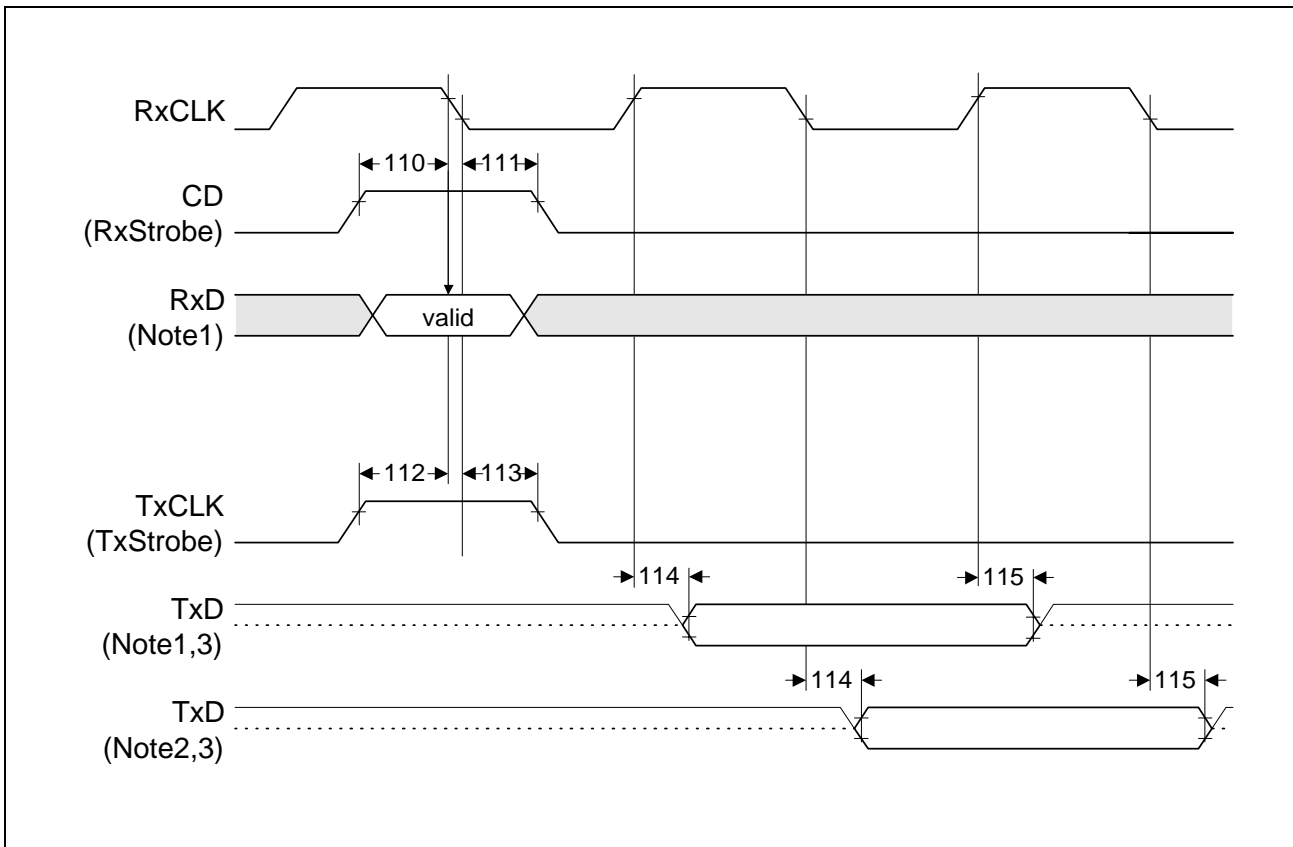
Figure 102 Strobe Timing
