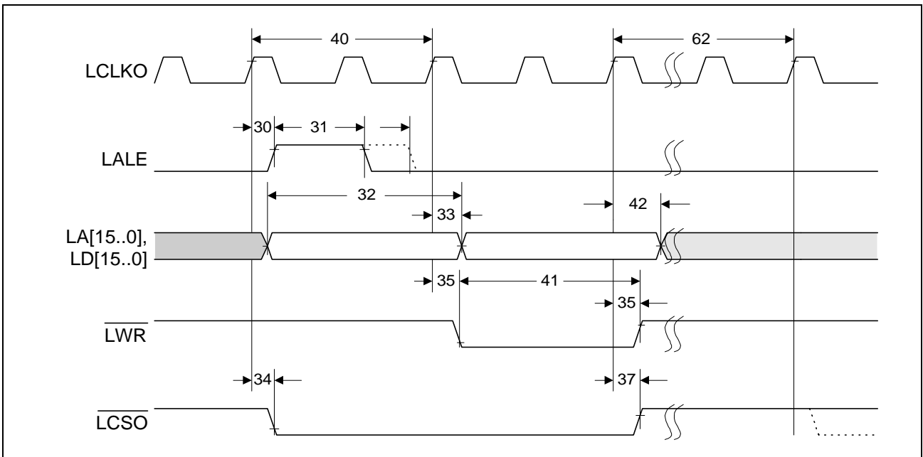
Figure 94 Synchronous LBI Write Cycle Timing Multiplexed Bus
