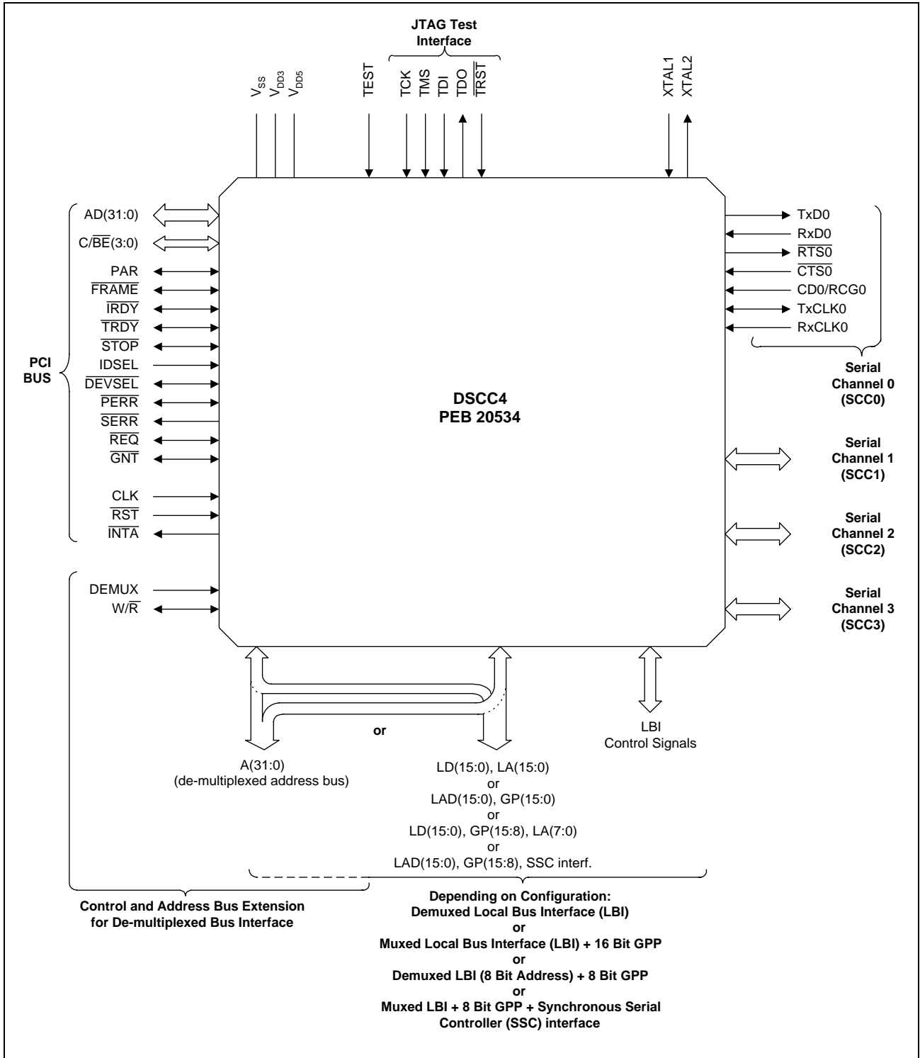
Figure 1 Logic Symbol
