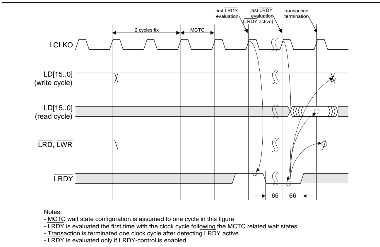
Figure 28 \overline{\text{LRDY}} Timing
