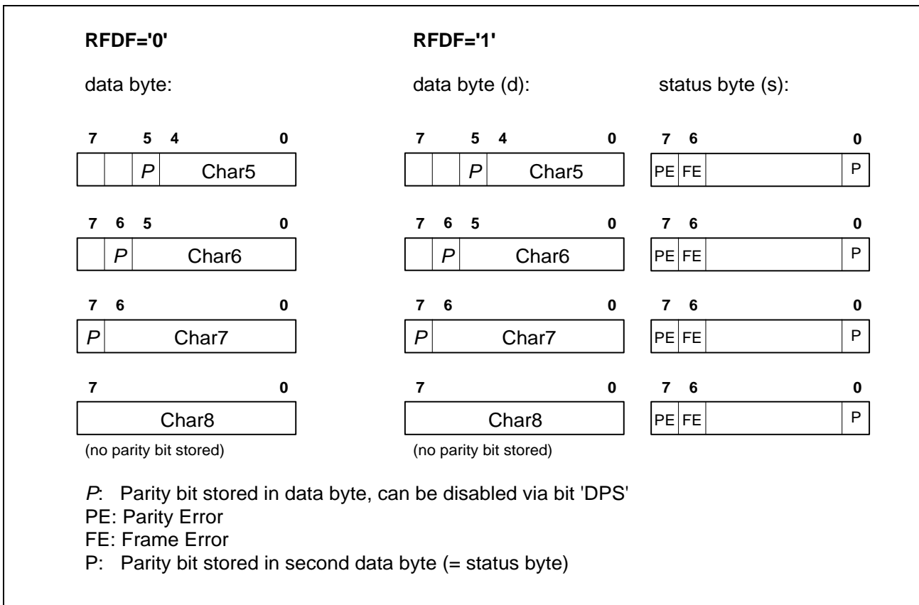
Figure 79 ASYNCR/BISYNCR Receive Status Character Format
