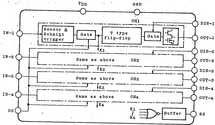
BLOCK DIAGRAM
