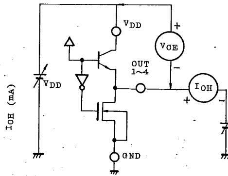
TEST CIRCUIT
