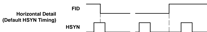
Figure 2–14. 525-Line Vertical Synchronization Signal
