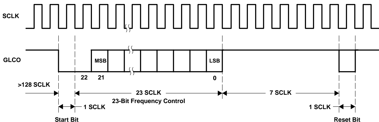
Figure 2–18. GLCO Timing
