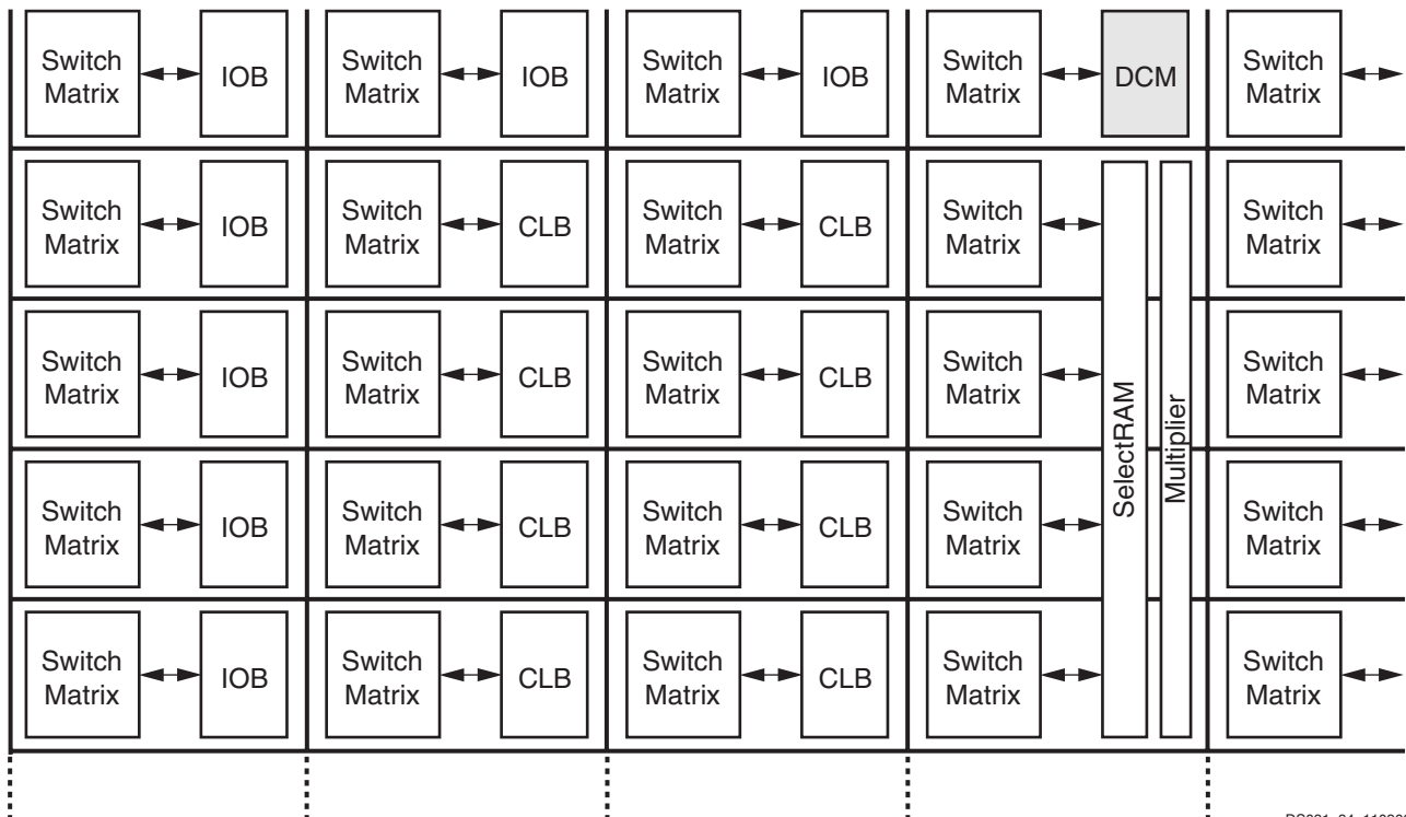
Figure 48: Routing Resources
