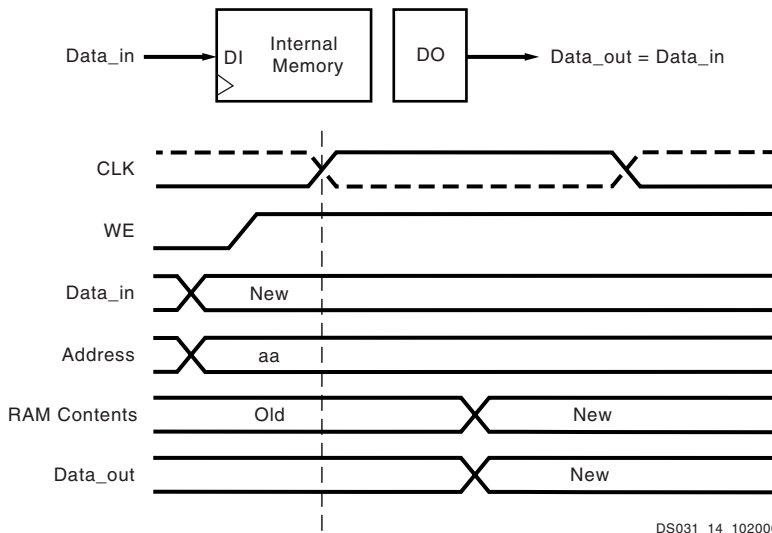
Figure 31: WRITE_FIRST Mode
