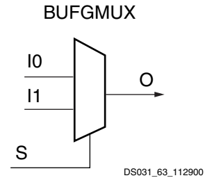
Figure 43: Virtex-II BUFGMUX Function
