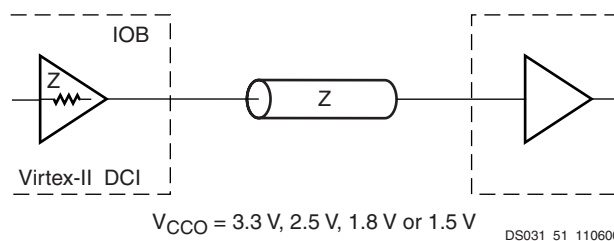
Figure 10: Internal Series Termination
