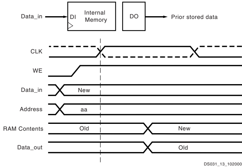
Figure 32: READ_FIRST Mode
