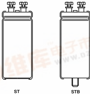
Fig.1 Component outlines
