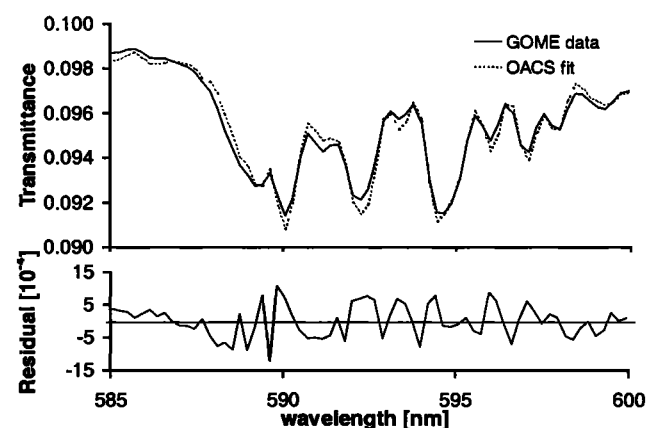
Figure 1. A sample OACS fit (dotted line) to the transmittance obtained from a single set of GOME radiance spectra (solid line) as a function of wavelength (upper plot), along with the residuals of the fit (lower plot). The radiance measurements were taken on October 23, 1998 at 18:00 UTC, 32.74°N, 252.36°E.
